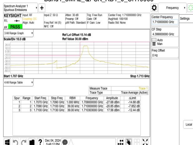
Band4_3MHz_QPSK_RB15_0_CH19965
