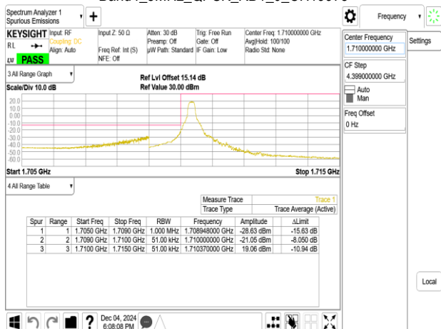
Band4_5MHz_QPSK_RB1_0_CH19975
