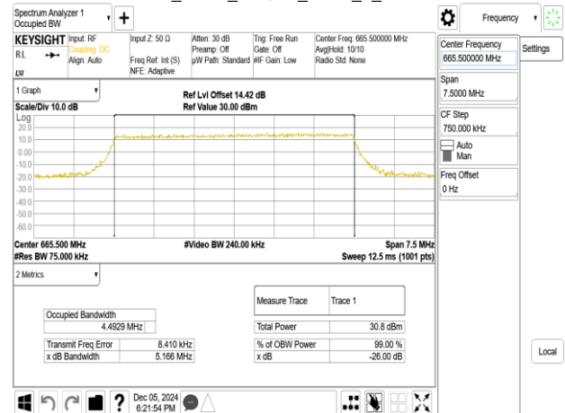
Band71_5MHz_64QAM_RB25_0_CH133147
