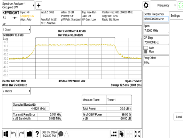
Band71_5MHz_64QAM_RB25_0_CH133297
