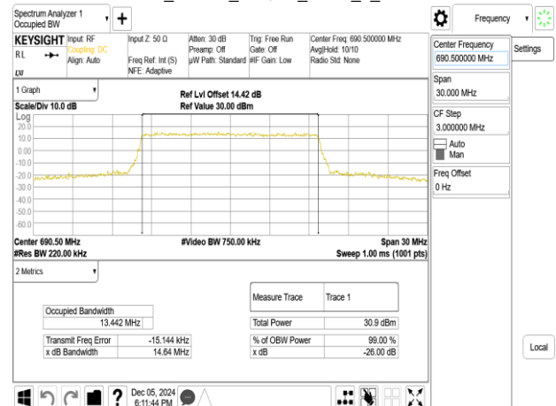
Band71_15MHz_16QAM_RB75_0_CH133397
