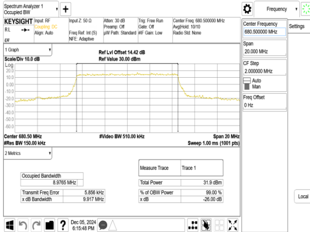
Band71_10MHz_16QAM_RB50_0_CH133297
