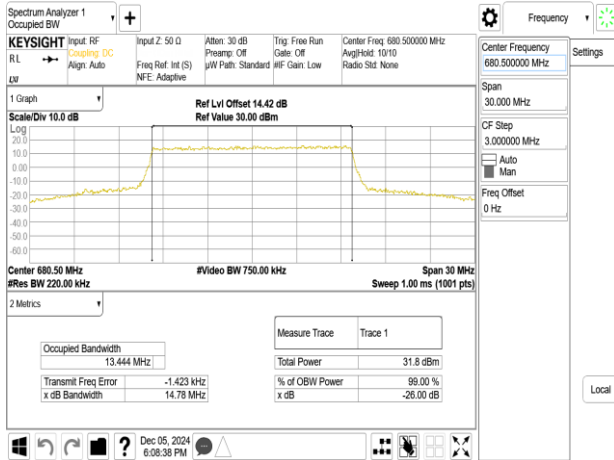
Band71_15MHz_16QAM_RB75_0_CH133297
