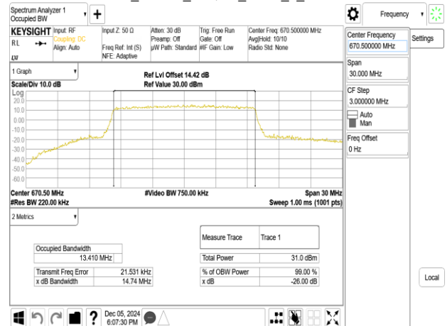
Band71_15MHz_64QAM_RB75_0_CH133197
