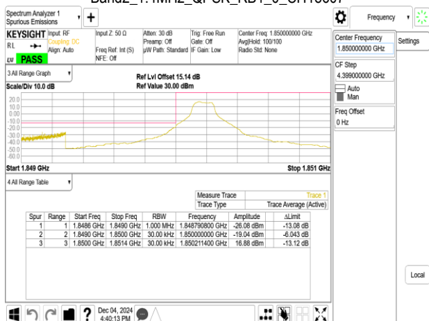
Band2_1.4MHz_QPSK_RB6_0_CH18607
