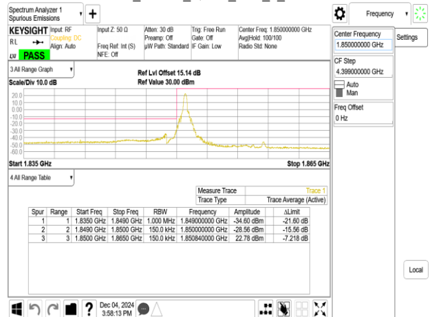
Band2_15MHz_QPSK_RB75_0_CH18675
