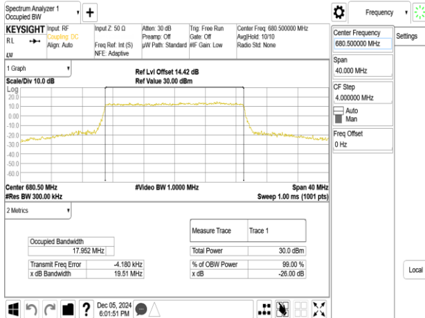
Band71_20MHz_64QAM_RB100_0_CH133297
