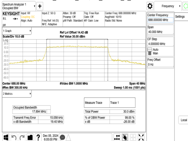
Band71_20MHz_256QAM_RB100_0_CH133372
