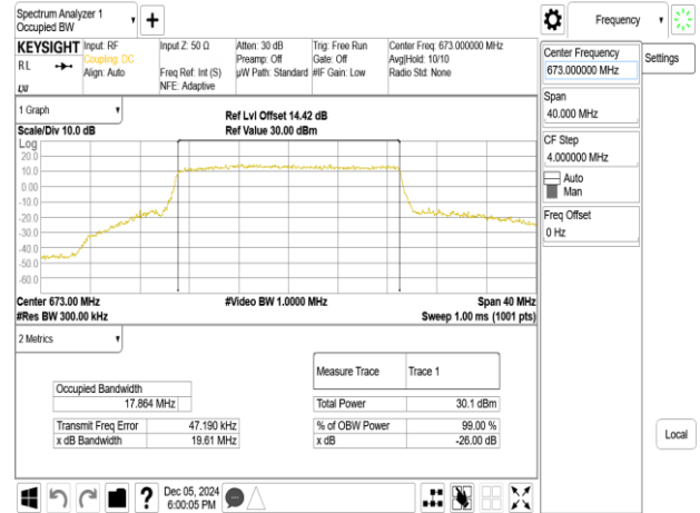
Band71_20MHz_256QAM_RB100_0_CH133222
