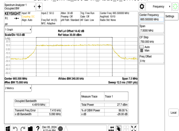
Band71_5MHz_256QAM_RB25_0_CH133147
