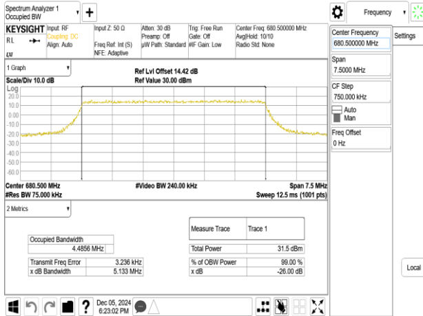
Band71_5MHz_16QAM_RB25_0_CH133297
