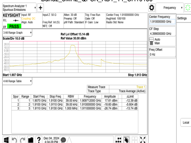
Band2_3MHz_QPSK_RB15_0_CH19185
