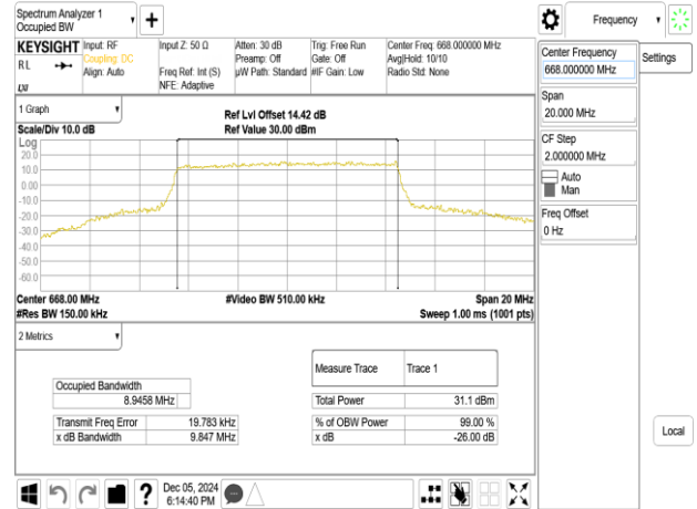
Band71_10MHz_64QAM_RB50_0_CH133172
