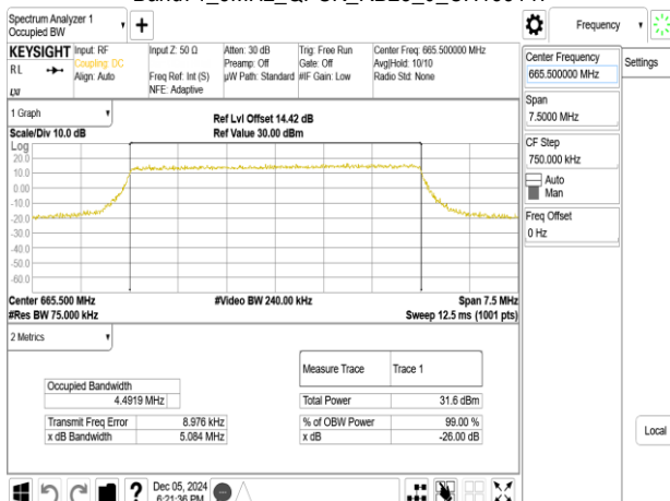
Band71_5MHz_QPSK_RB25_0_CH133147
