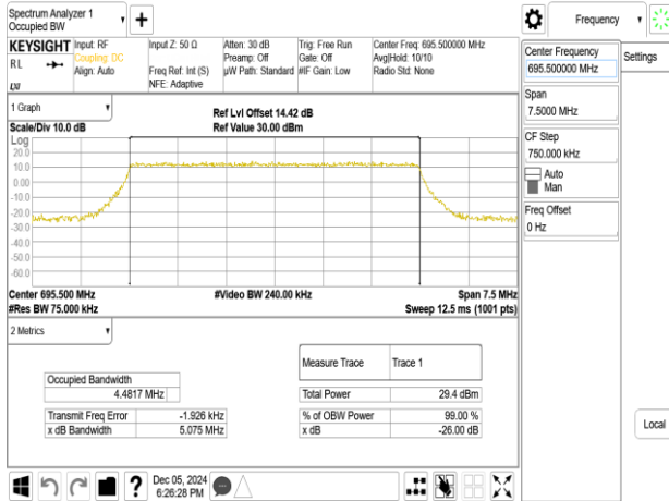
Band71_5MHz_256QAM_RB25_0_CH133447
