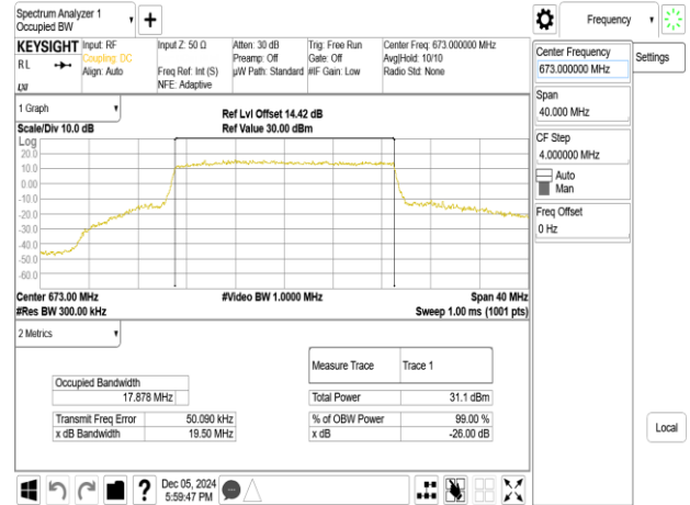
Band71_20MHz_64QAM_RB100_0_CH133222
