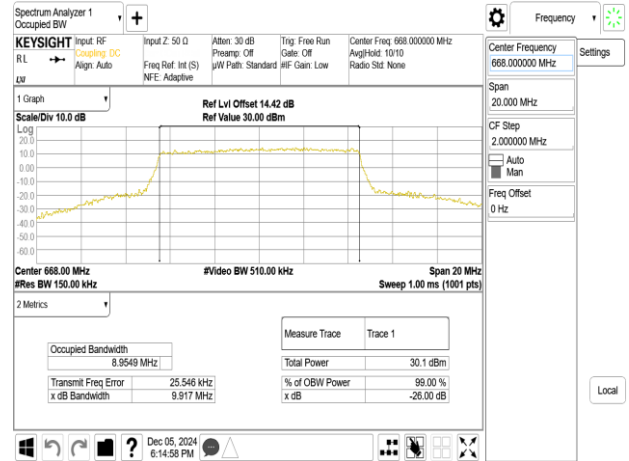
Band71_10MHz_256QAM_RB50_0_CH133172
