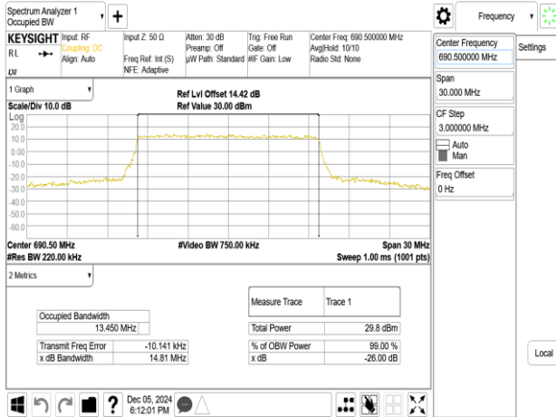
Band71_15MHz_256QAM_RB75_0_CH133397
