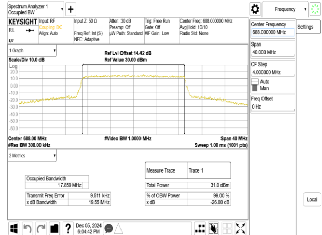
Band71_20MHz_16QAM_RB100_0_CH133372
