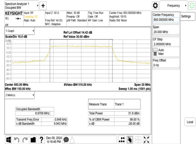
Band71_10MHz_16QAM_RB50_0_CH133422
