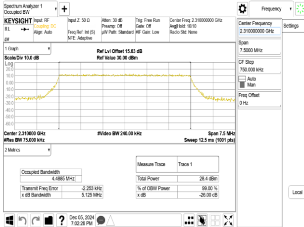
Band30_5MHz_256QAM_RB25_0_CH27710
