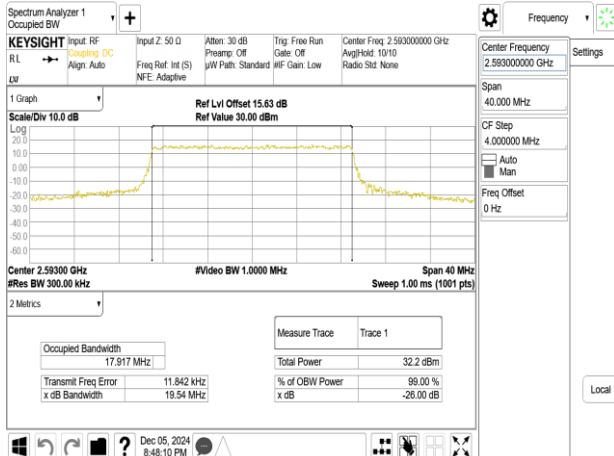
Band41_20MHz_64QAM_RB100_0_CH40620
