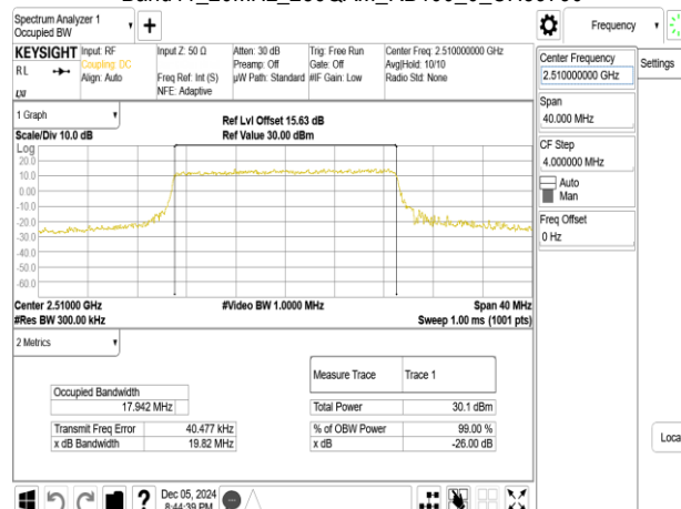
Band41_20MHz_256QAM_RB100_0_CH39790
