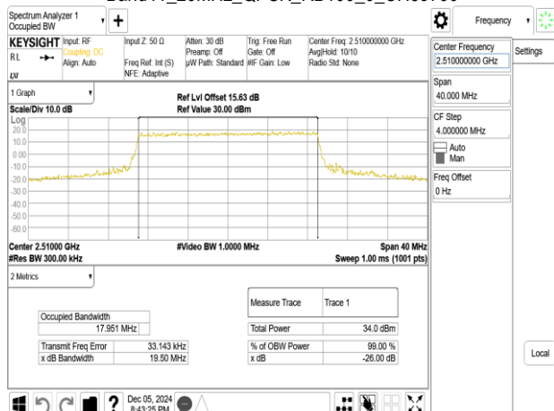
Band41_20MHz_QPSK_RB100_0_CH39790
