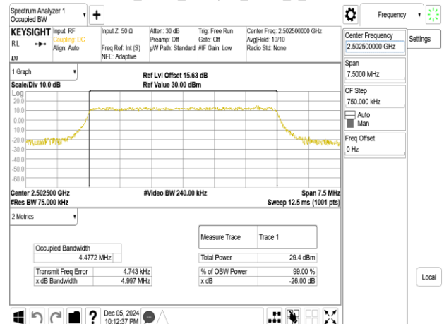
Band41_5MHz_256QAM_RB25_0_CH39715
