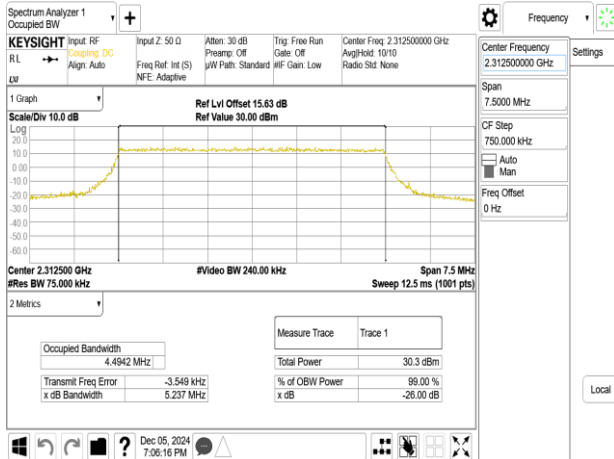
Band30_5MHz_QPSK_RB25_0_CH27735
