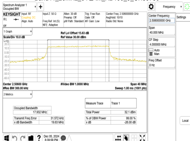
Band41_20MHz_256QAM_RB100_0_CH39750
