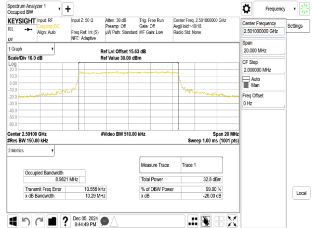
Band41_10MHz_64QAM_RB50_0_CH39700
