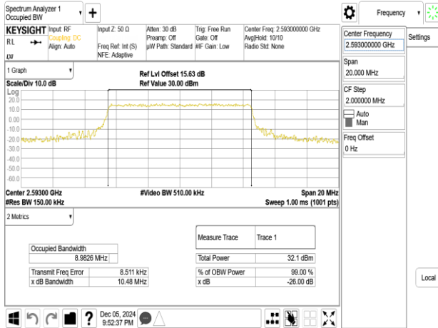
Band41_10MHz_256QAM_RB50_0_CH40620
