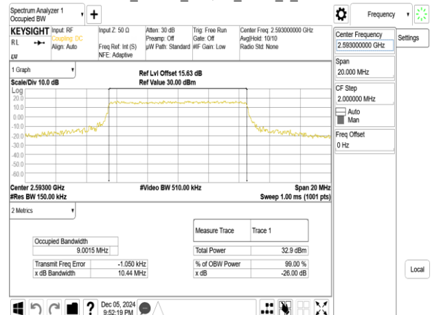
Band41_10MHz_16QAM_RB50_0_CH40620
