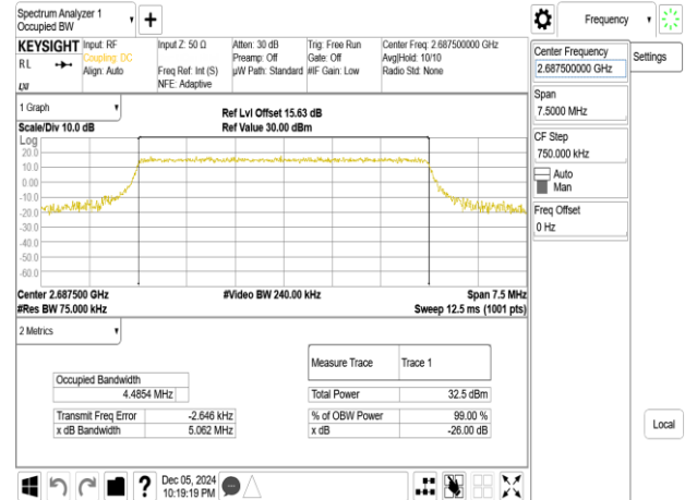
Band41_5MHz_16QAM_RB25_0_CH41565
