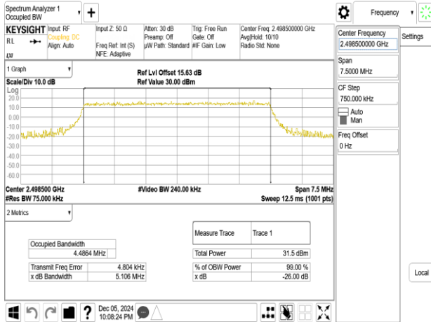
Band41_5MHz_256QAM_RB25_0_CH39675
