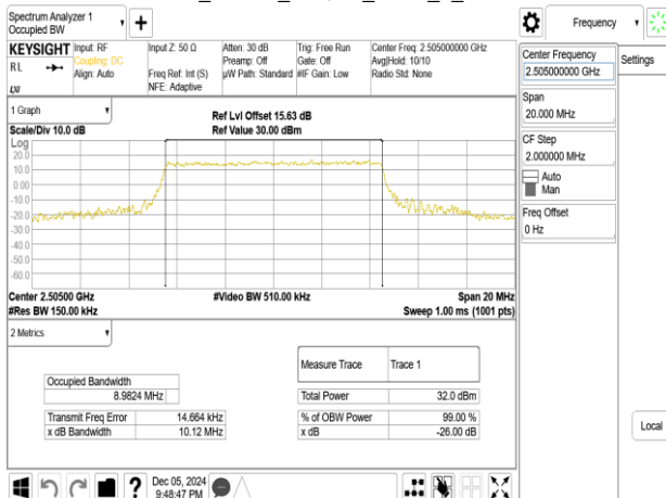
Band41_10MHz_64QAM_RB50_0_CH39740
