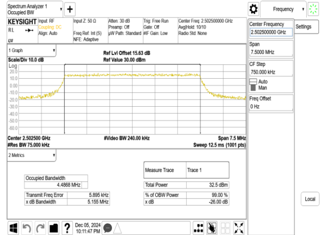
Band41_5MHz_64QAM_RB25_0_CH39715
