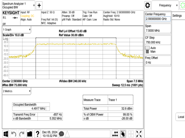
Band41_5MHz_64QAM_RB25_0_CH40620
