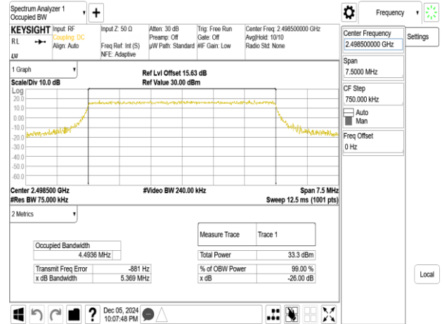
Band41_5MHz_16QAM_RB25_0_CH39675
