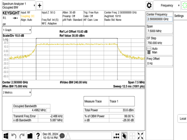
Band41_5MHz_16QAM_RB25_0_CH40620
