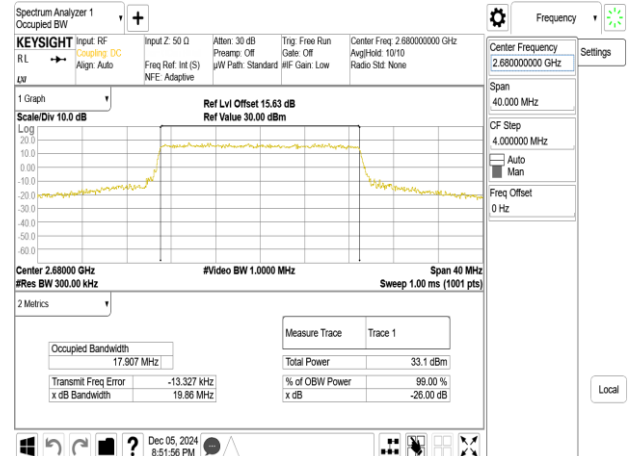
Band41_20MHz_16QAM_RB100_0_CH41490
