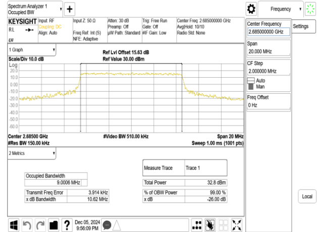
Band41_10MHz_64QAM_RB50_0_CH41540
