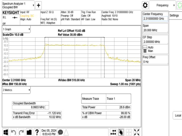
Band30_10MHz_64QAM_RB50_0_CH27710
