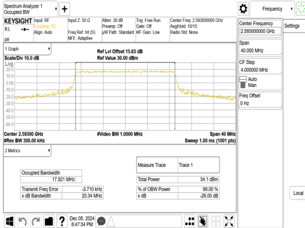
Band41_20MHz_16QAM_RB100_0_CH40620
