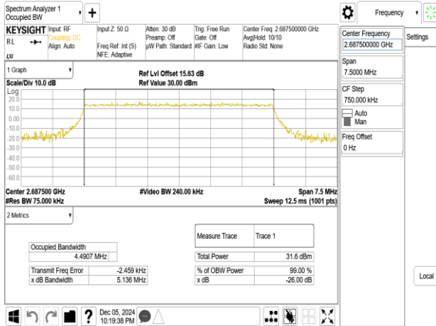
Band41_5MHz_256QAM_RB25_0_CH41565
