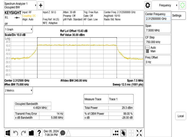
Band30_5MHz_64QAM_RB25_0_CH27735
