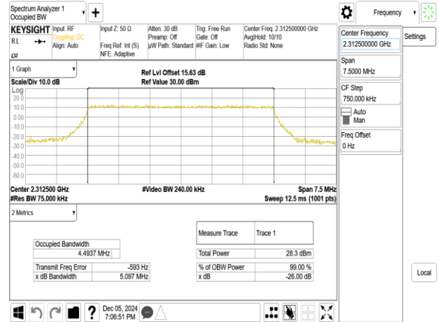
Band30_5MHz_256QAM_RB25_0_CH27735
