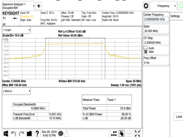
Band41_10MHz_16QAM_RB50_0_CH39740
