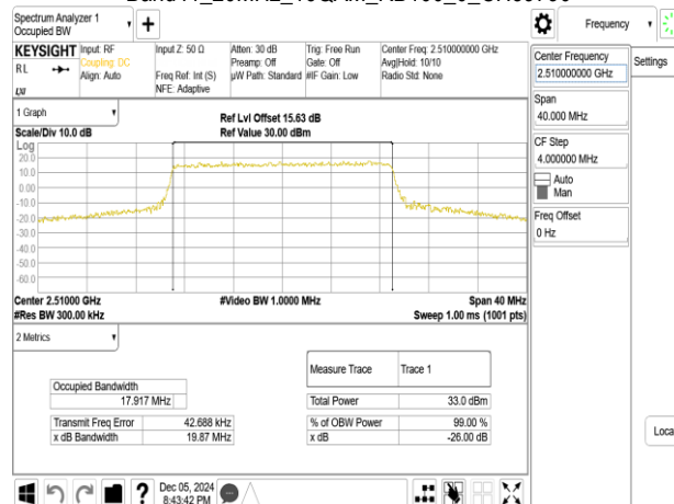
Band41_20MHz_64QAM_RB100_0_CH39790
