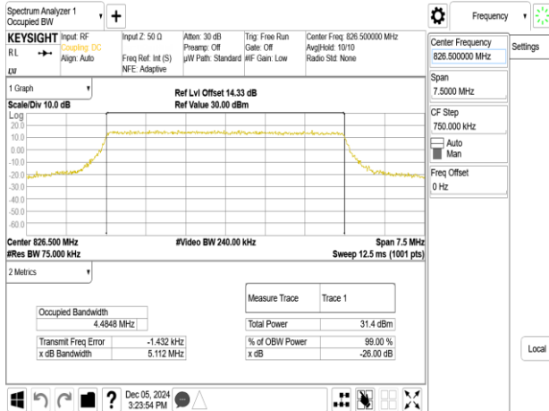
Band26_5MHz_QPSK_RB25_0_CH26815
