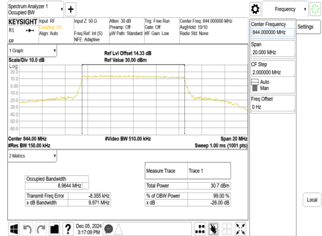
Band26_10MHz_64QAM_RB50_0_CH26990
