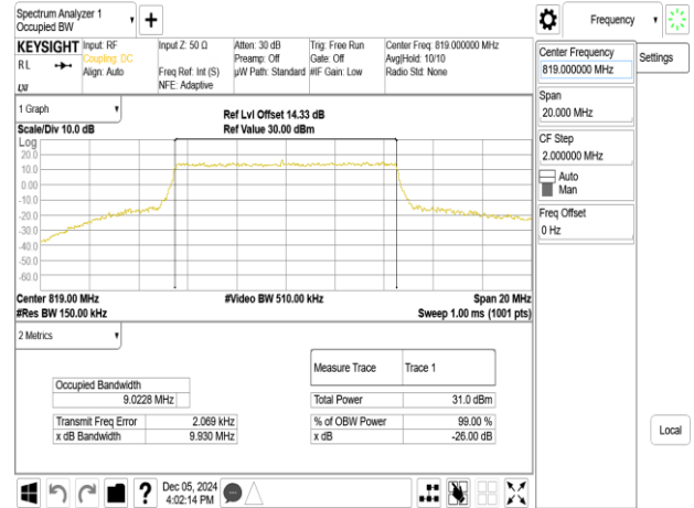
Band26-Part90s_10MHz_64QAM_RB50_0_CH26740
