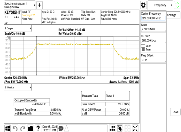
Band26_5MHz_256QAM_RB25_0_CH26815
