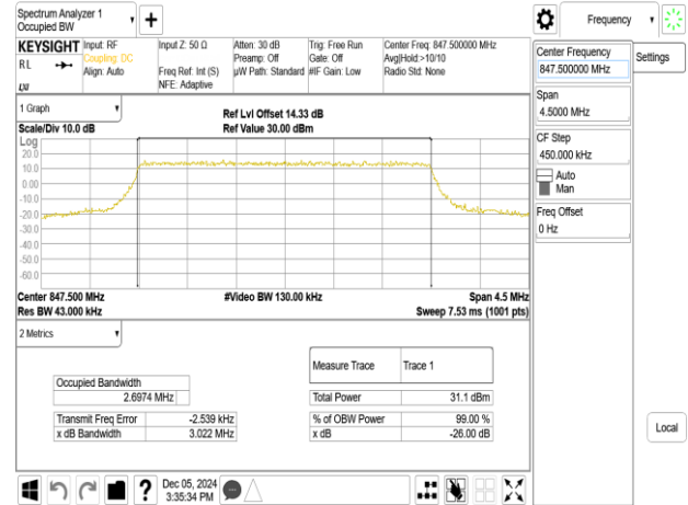
Band26_3MHz_16QAM_RB15_0_CH27025
