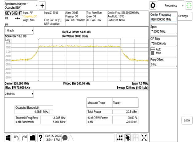
Band26_5MHz_64QAM_RB25_0_CH26815
