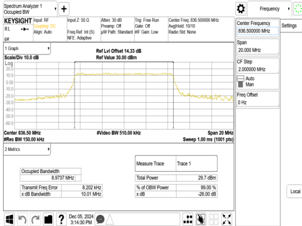
Band26_10MHz_256QAM_RB50_0_CH26915
