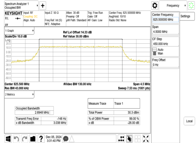
Band26_3MHz_64QAM_RB15_0_CH26805
