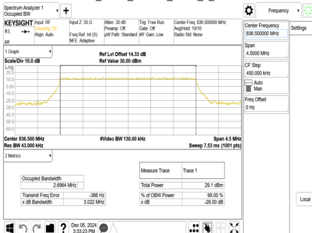
Band26_3MHz_64QAM_RB15_0_CH26915
