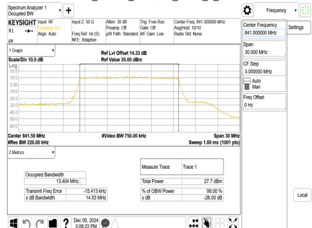
Band26_15MHz_256QAM_RB75_0_CH26965
