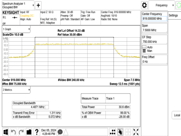
Band26-Part90s_5MHz_64QAM_RB25_0_CH26740
