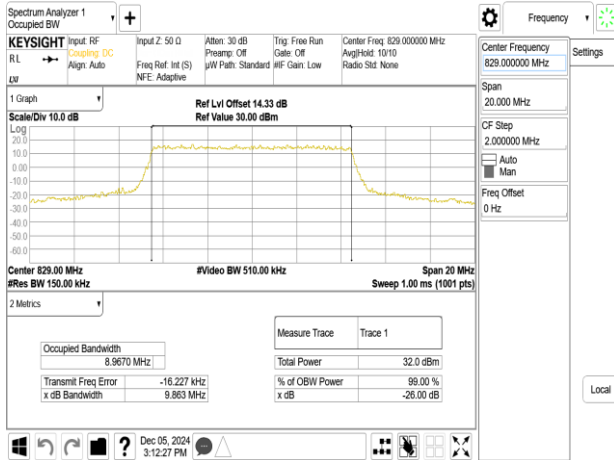
Band26_10MHz_16QAM_RB50_0_CH26840
