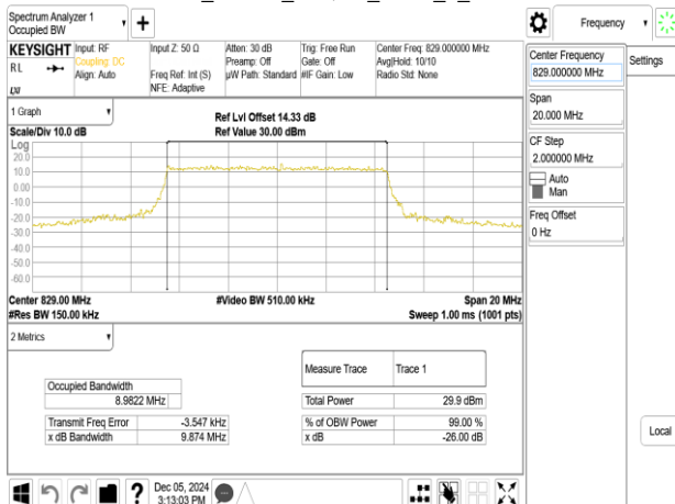
Band26_10MHz_64QAM_RB50_0_CH26840
