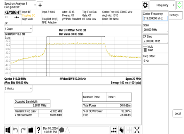
Band26-Part90s_10MHz_256QAM_RB50_0_CH26740
