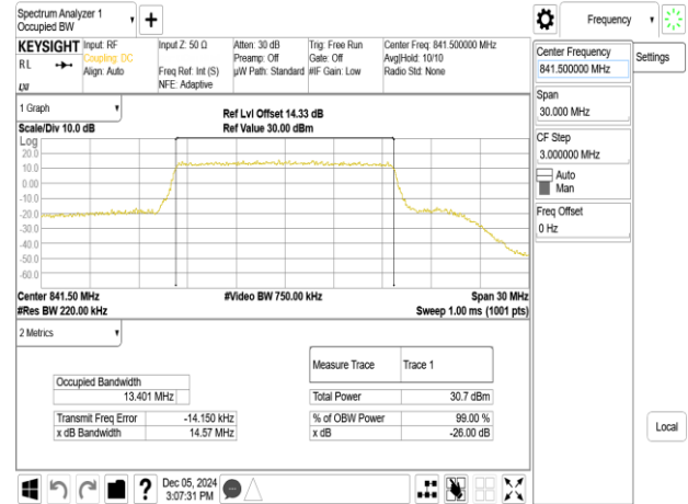
Band26_15MHz_64QAM_RB75_0_CH26965
