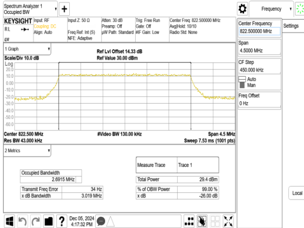
Band26-Part90s_3MHz_256QAM_RB15_0_CH26775
