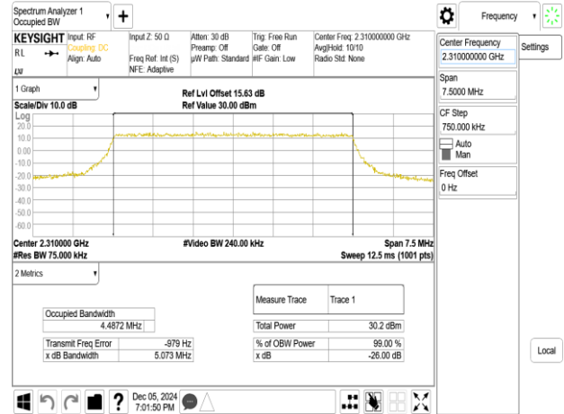
Band30_5MHz_16QAM_RB25_0_CH27710
