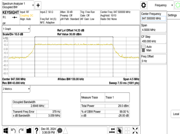
Band26_3MHz_256QAM_RB15_0_CH27025
