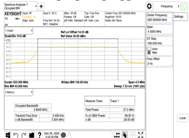
Band26_3MHz_256QAM_RB15_0_CH26805
