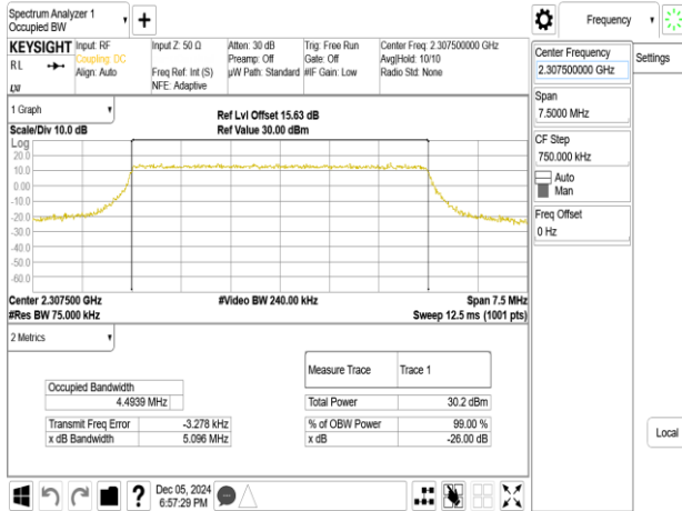
Band30_5MHz_16QAM_RB25_0_CH27685
