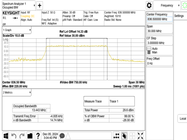
Band26_15MHz_256QAM_RB75_0_CH26915
