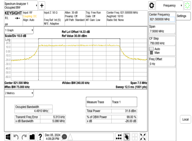
Band26-Part90s_5MHz_16QAM_RB25_0_CH26765
