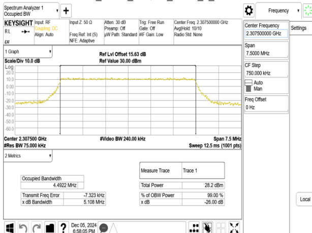
Band30_5MHz_64QAM_RB25_0_CH27685
