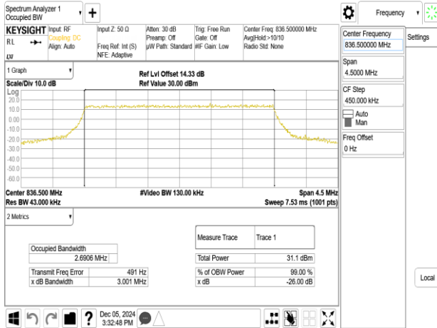
Band26_3MHz_16QAM_RB15_0_CH26915
