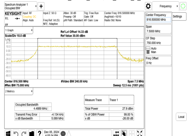
Band26-Part90s_5MHz_256QAM_RB25_0_CH26715
