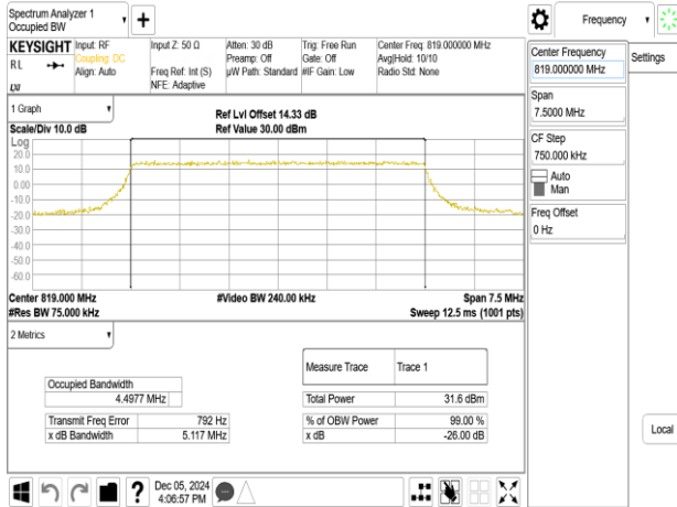
Band26-Part90s_5MHz_16QAM_RB25_0_CH26740
