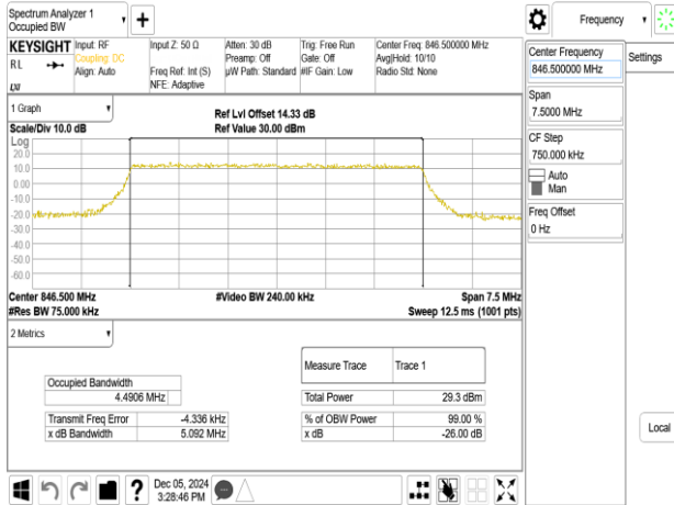
Band26_5MHz_256QAM_RB25_0_CH27015
