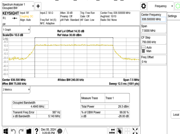
Band26_5MHz_64QAM_RB25_0_CH26915
