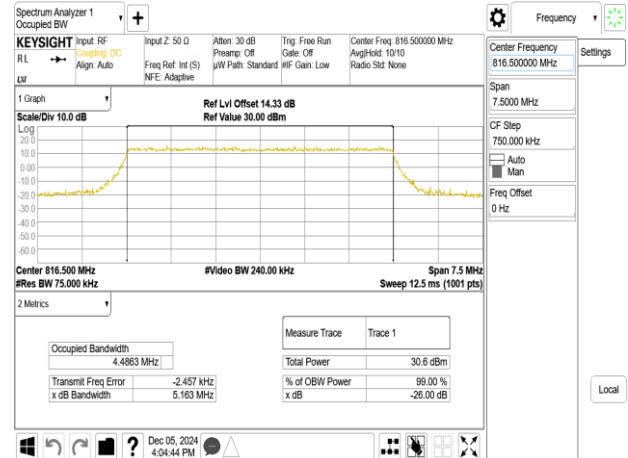
Band26-Part90s_5MHz_64QAM_RB25_0_CH26715
