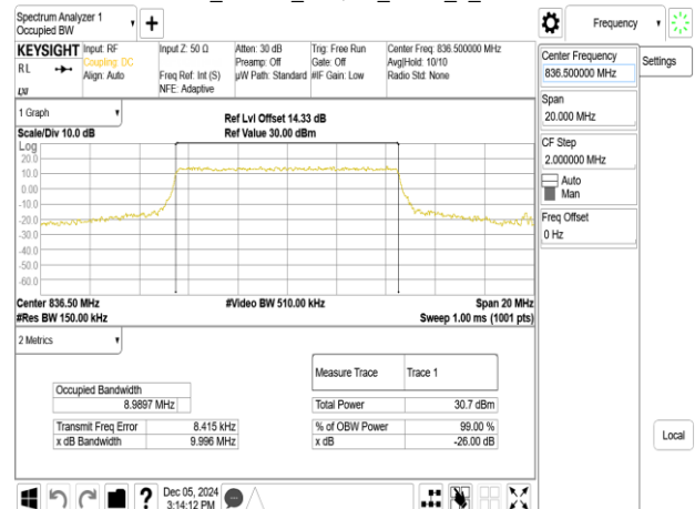
Band26_10MHz_16QAM_RB50_0_CH26915
