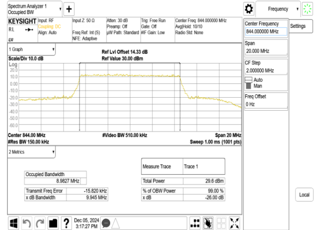
Band26_10MHz_256QAM_RB50_0_CH26990
