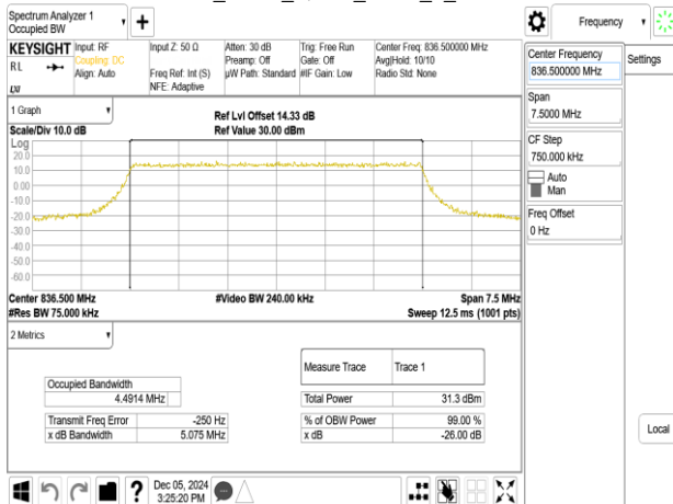
Band26_5MHz_16QAM_RB25_0_CH26915
