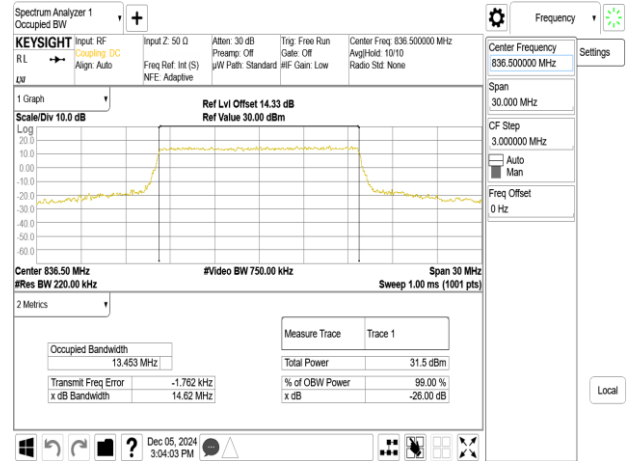
Band26_15MHz_16QAM_RB75_0_CH26915
