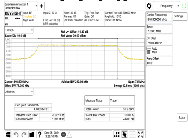
Band26_5MHz_16QAM_RB25_0_CH27015
