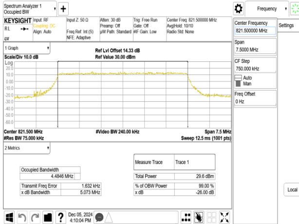
Band26-Part90s_5MHz_256QAM_RB25_0_CH26765
