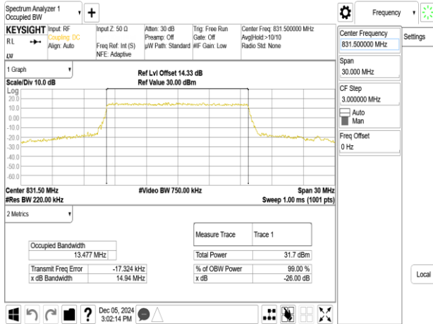
Band26_15MHz_16QAM_RB75_0_CH26865
