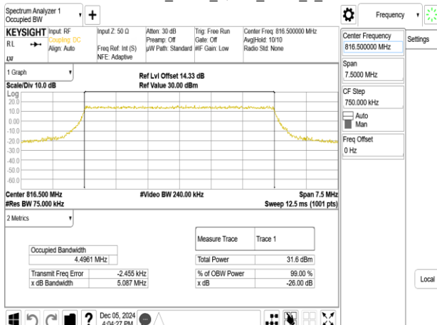
Band26-Part90s_5MHz_QPSK_RB25_0_CH26715
