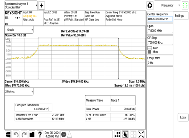
Band26-Part90s_5MHz_256QAM_RB25_0_CH26715
