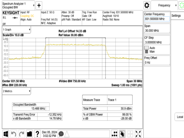
Band26_15MHz_64QAM_RB75_0_CH26865
