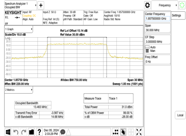
Band25_15MHz_64QAM_RB75_0_CH26115
