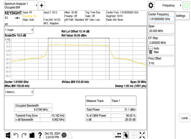
Band25_10MHz_16QAM_RB50_0_CH26640
