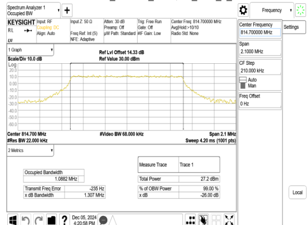
Band26-Part90s_1.4MHz_256QAM_RB6_0_CH26697
