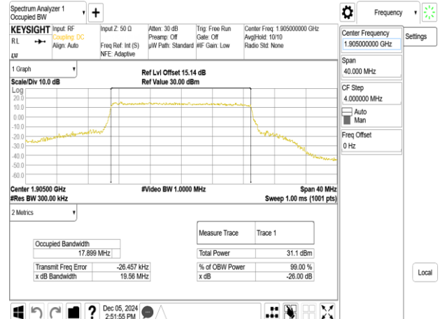
Band25_20MHz_16QAM_RB100_0_CH26590
