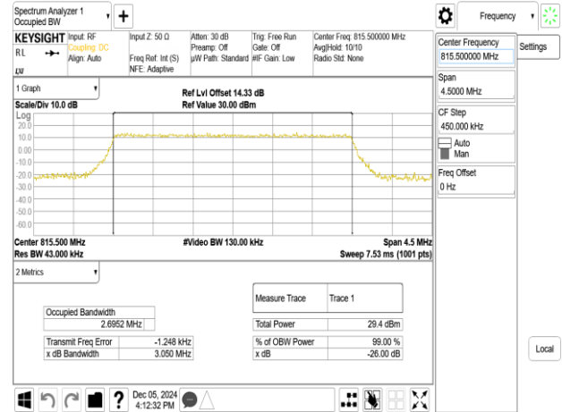
Band26-Part90s_3MHz_256QAM_RB15_0_CH26705
