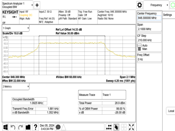
Band26_1.4MHz_256QAM_RB6_0_CH27033
