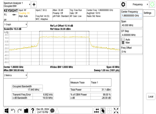
Band25_20MHz_64QAM_RB100_0_CH26140
