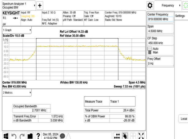
Band26-Part90s_3MHz_64QAM_RB15_0_CH26740
