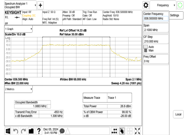
Band26_1.4MHz_QPSK_RB6_0_CH27033
