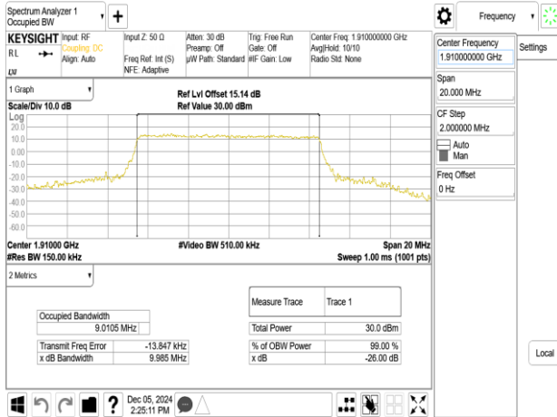
Band25_10MHz_256QAM_RB50_0_CH26640
