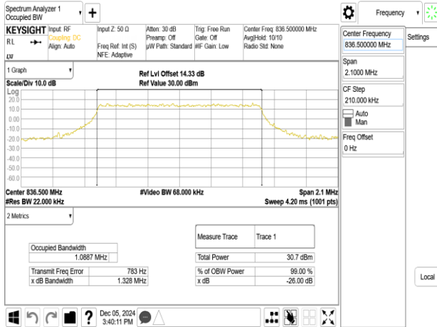
Band26_1.4MHz_16QAM_RB6_0_CH26915
