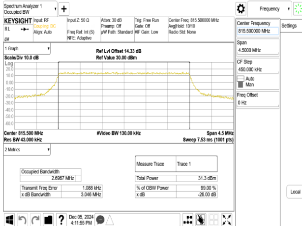
Band26-Part90s_3MHz_QPSK_RB15_0_CH26705
