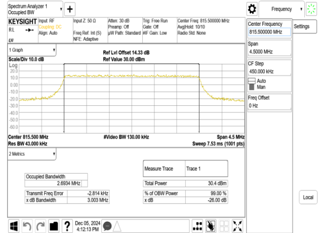
Band26-Part90s_3MHz_64QAM_RB15_0_CH26705
