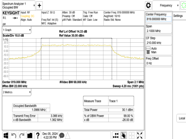
Band26-Part90s_1.4MHz_64QAM_RB6_0_CH26740
