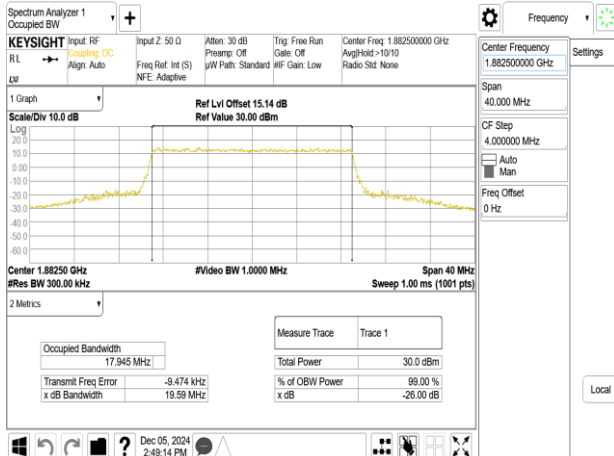
Band25_20MHz_64QAM_RB100_0_CH26365
