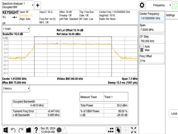
Band25_5MHz_256QAM_RB25_0_CH26665
