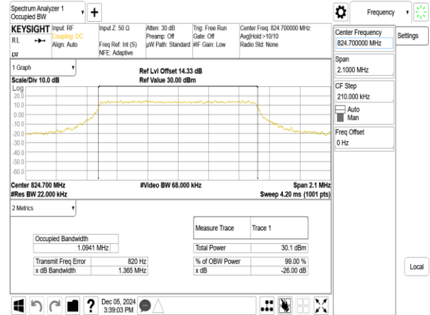
Band26_1.4MHz_64QAM_RB6_0_CH26797
