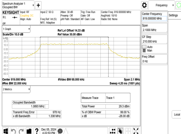
Band26-Part90s_1.4MHz_64QAM_RB6_0_CH26740
