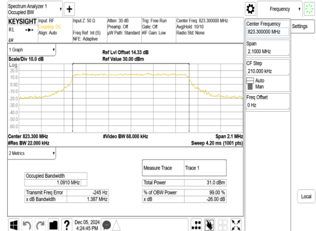
Band26-Part90s_1.4MHz_16QAM_RB6_0_CH26783
