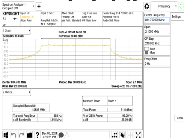
Band26-Part90s_1.4MHz_QPSK_RB6_0_CH26697
