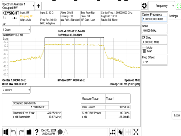
Band25_20MHz_256QAM_RB100_0_CH26590
