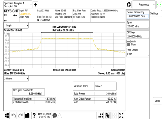
Band25_10MHz_64QAM_RB50_0_CH26090
