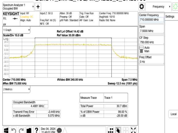
Band17_5MHz_64QAM_RB25_0_CH23790
