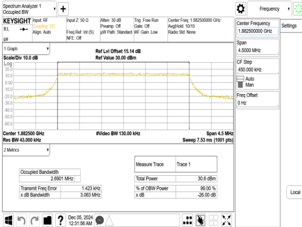
Band25_3MHz_64QAM_RB15_0_CH26365
