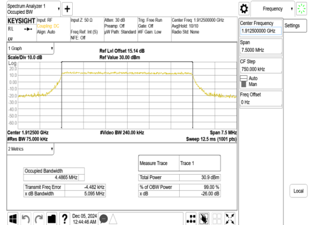
Band25_5MHz_16QAM_RB25_0_CH26665
