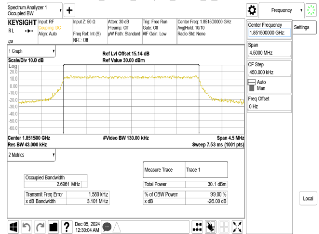
Band25_3MHz_64QAM_RB15_0_CH26055
