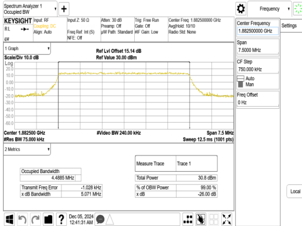
Band25_5MHz_64QAM_RB25_0_CH26365
