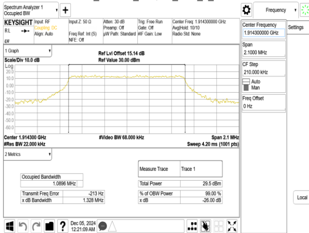
Band25_1.4MHz_256QAM_RB6_0_CH26683
