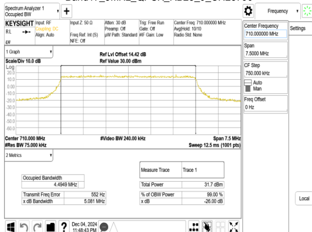
Band17_5MHz_16QAM_RB25_0_CH23790
