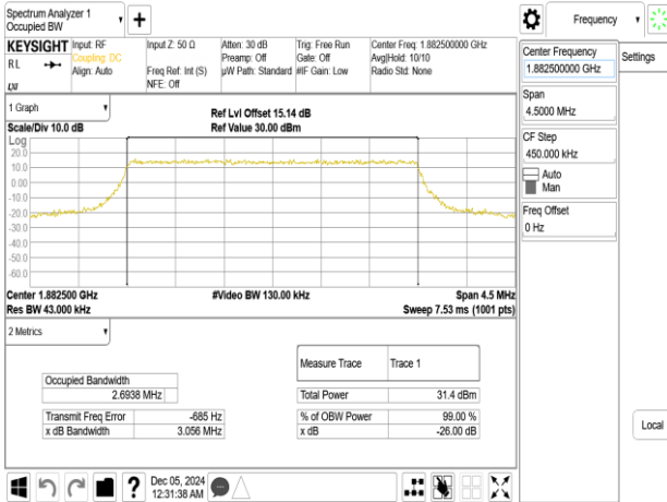
Band25_3MHz_16QAM_RB15_0_CH26365
