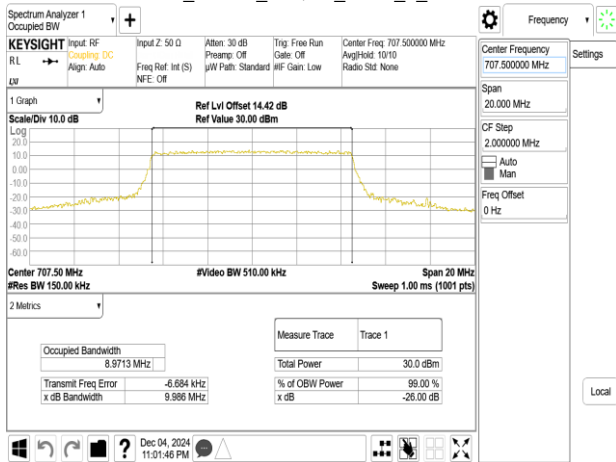
Band12_10MHz_256QAM_RB50_0_CH23095
