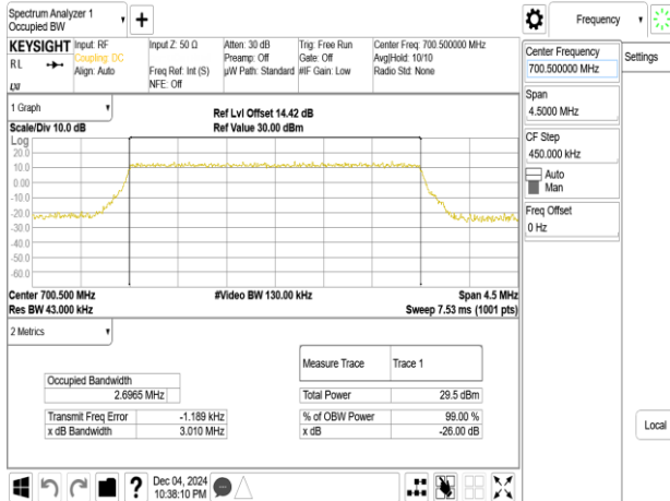
Band12_3MHz_64QAM_RB15_0_CH23025
