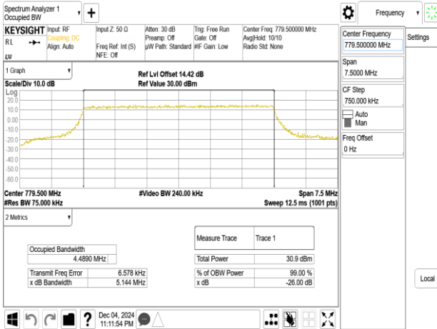
Band13_5MHz_64QAM_RB25_0_CH23205
