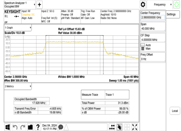
Band7_20MHz_64QAM_RB100_0_CH21350
