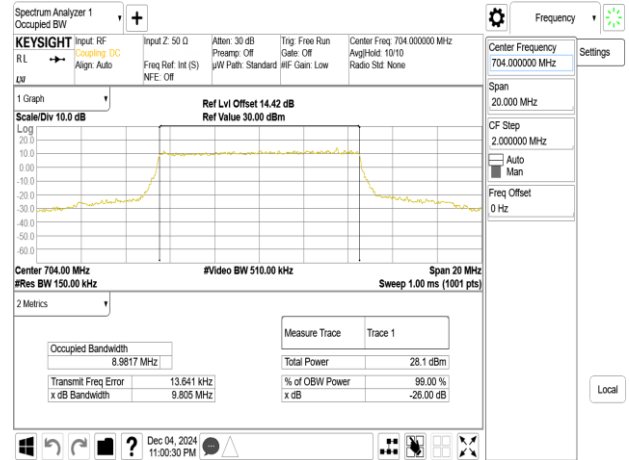
Band12_10MHz_QPSK_RB50_0_CH23095
