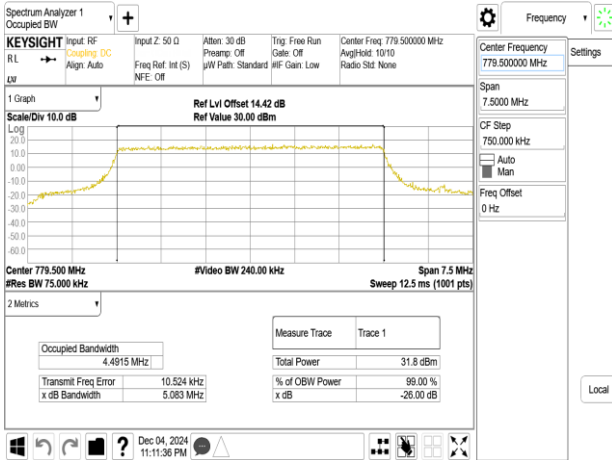
Band13_5MHz_16QAM_RB25_0_CH23205
