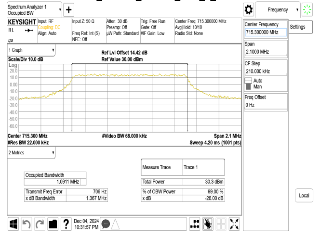
Band12_1.4MHz_64QAM_RB6_0_CH23173
