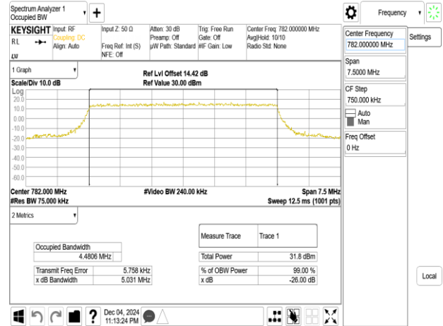
Band13_5MHz_16QAM_RB25_0_CH23230
