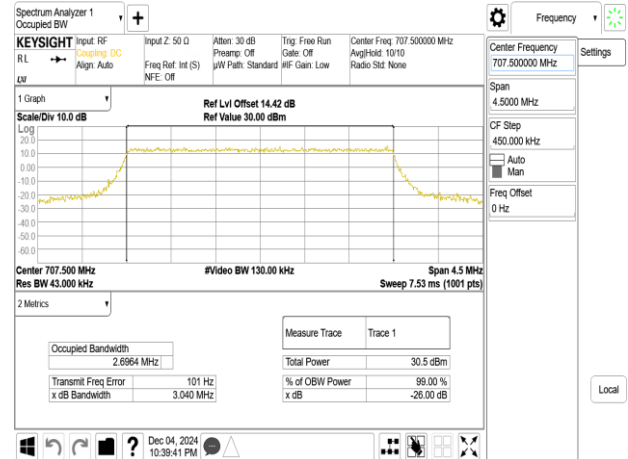
Band12_3MHz_16QAM_RB15_0_CH23095
