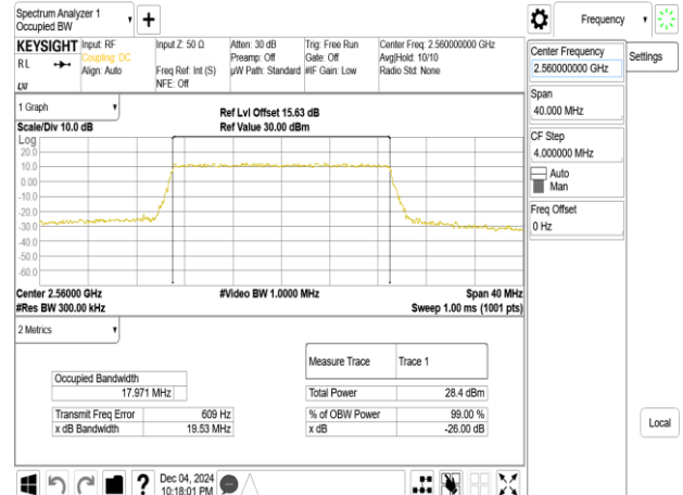
Band7_20MHz_256QAM_RB100_0_CH21350
