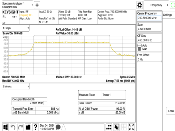
Band12_3MHz_16QAM_RB15_0_CH23025
