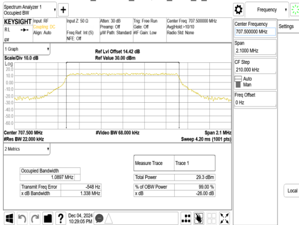
Band12_1.4MHz_256QAM_RB6_0_CH23095
