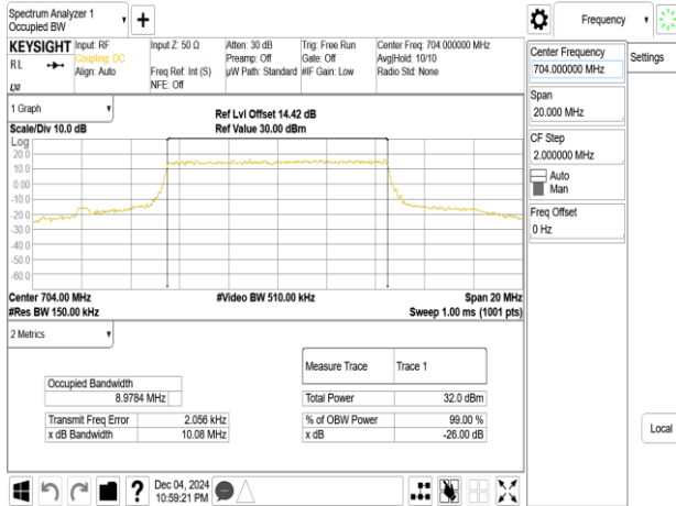
Band12_10MHz_16QAM_RB50_0_CH23060
