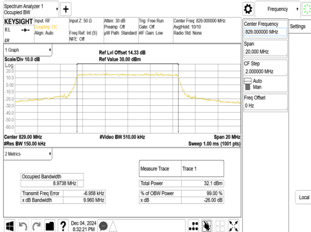
Band5_10MHz_16QAM_RB50_0_CH20450
