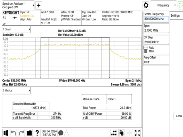
Band5_1.4MHz_256QAM_RB6_0_CH20525
