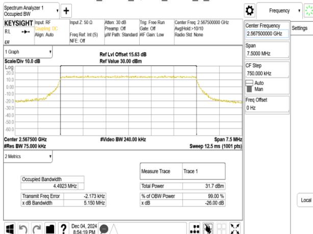
Band7_5MHz_QPSK_RB25_0_CH21425
