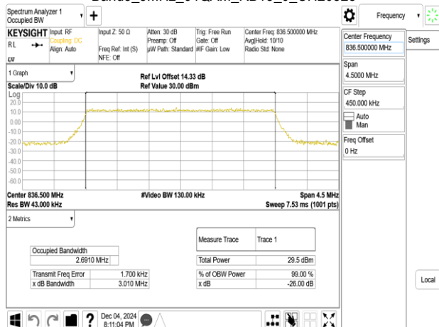
Band5_3MHz_256QAM_RB15_0_CH20525
