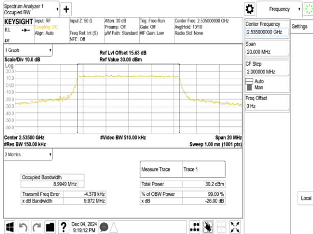
Band7_10MHz_256QAM_RB50_0_CH21100
