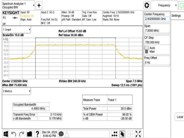
Band7_5MHz_64QAM_RB25_0_CH20775
