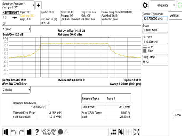
Band5_1.4MHz_16QAM_RB6_0_CH20407
