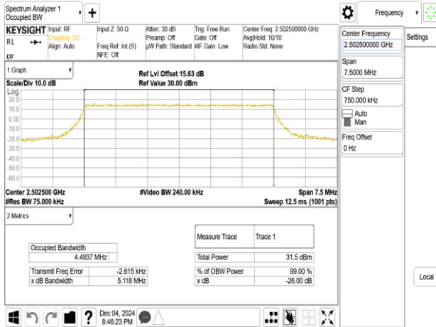
Band7_5MHz_16QAM_RB25_0_CH20775
