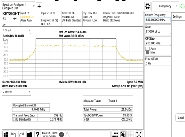
Band5_5MHz_64QAM_RB25_0_CH20425
