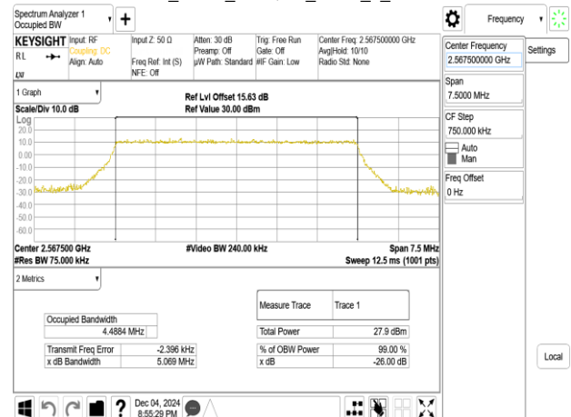
Band7_5MHz_256QAM_RB25_0_CH21425
