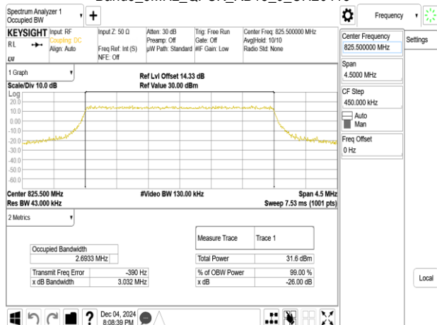
Band5_3MHz_16QAM_RB15_0_CH20415
