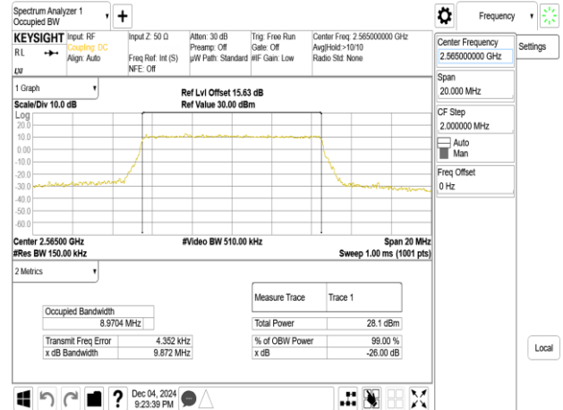
Band7_10MHz_256QAM_RB50_0_CH21400
