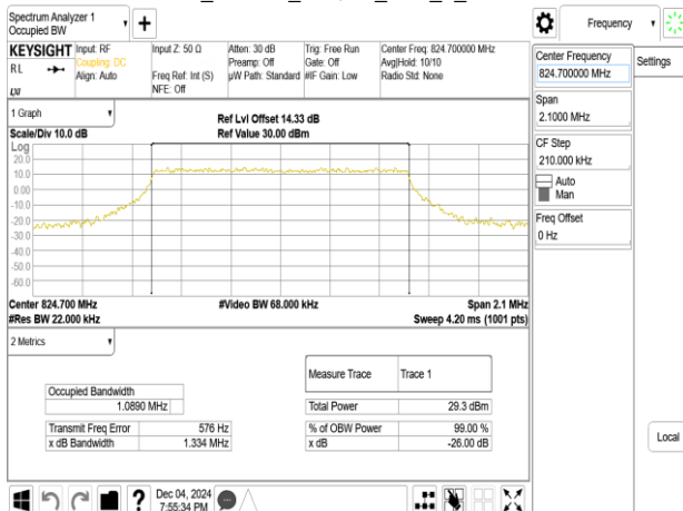
Band5_1.4MHz_64QAM_RB6_0_CH20407
