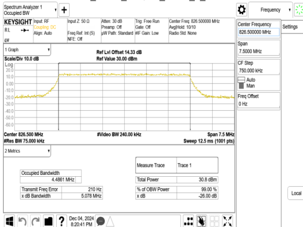
Band5_5MHz_64QAM_RB25_0_CH20425
