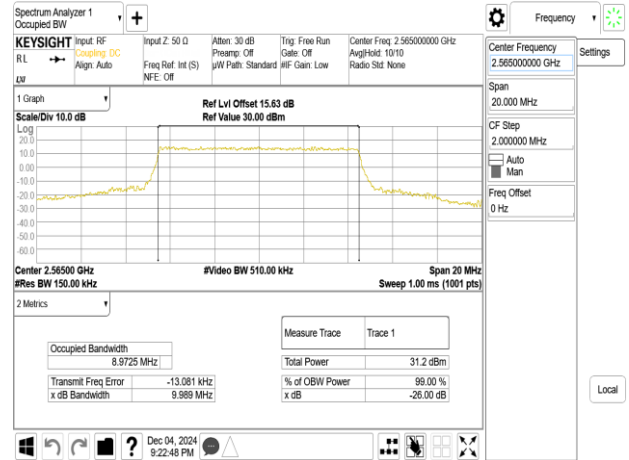
Band7_10MHz_64QAM_RB50_0_CH21400
