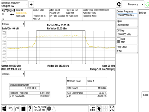
Band7_10MHz_16QAM_RB50_0_CH20800
