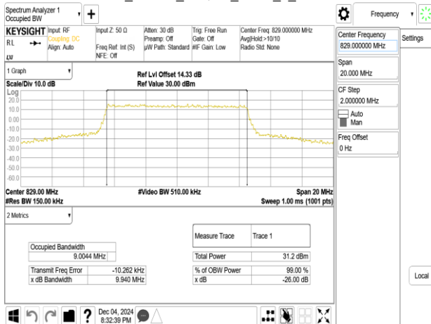
Band5_10MHz_64QAM_RB50_0_CH20450
