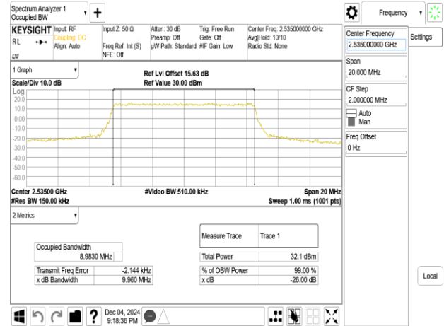
Band7_10MHz_16QAM_RB50_0_CH21100
