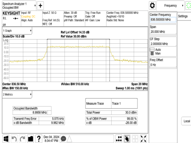
Band5_10MHz_256QAM_RB50_0_CH20525
