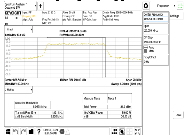
Band5_10MHz_16QAM_RB50_0_CH20525
