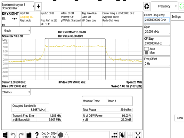
Band7_10MHz_64QAM_RB50_0_CH20800
