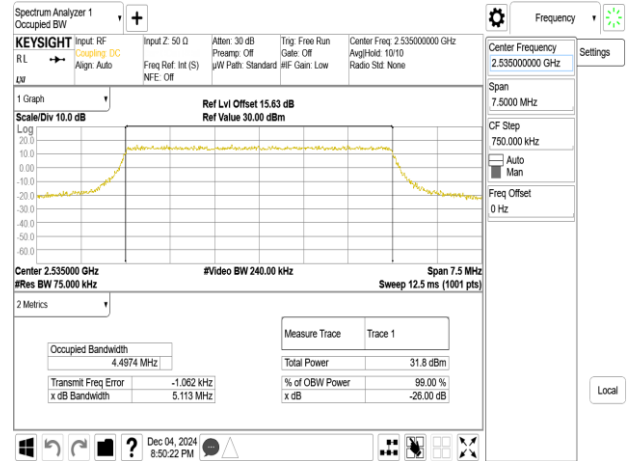
Band7_5MHz_16QAM_RB25_0_CH21100
