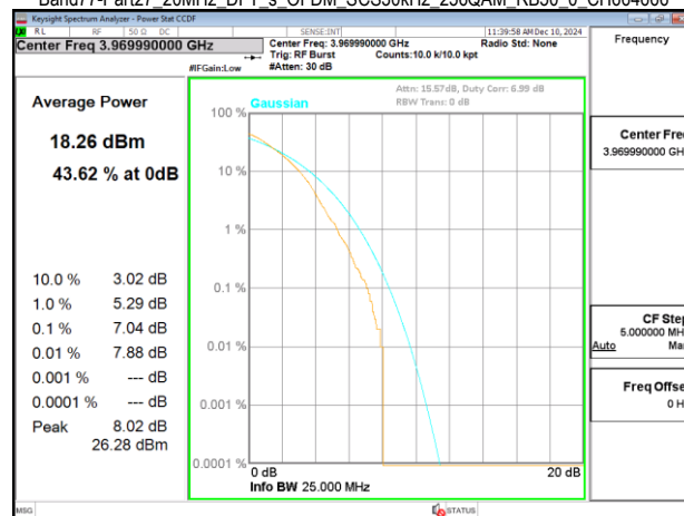
Band77-Part27_20MHz_DFT_s_OFDM_SCS30kHz_256QAM_RB50_0_CH664666
