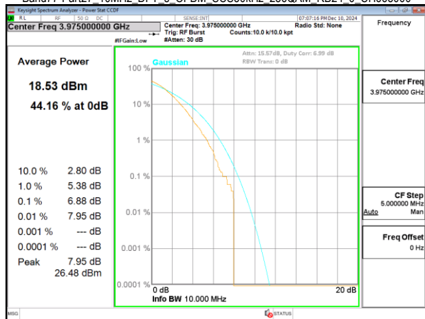
Band77-Part27_10MHz_DFT_s_OFDM_SCS30kHz_256QAM_RB24_0_CH665000
