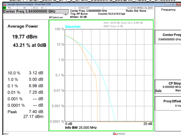
Band77-Part27_20MHz_DFT_s_OFDM_SCS30kHz_256QAM_RB50_0_CH656000
