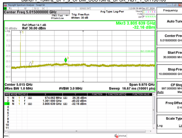
Band71_15MHz_DFT_s_OFDM_SCS15kHz_BPSK_RB1_1_CH138100
