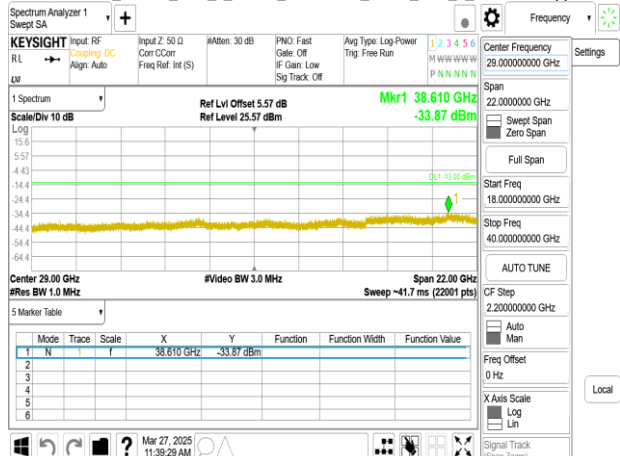
Band77-Part27_10MHz_DFT_s_OFDM_SCS30kHz_BPSK_RB1_1_CH636332upper 18G
