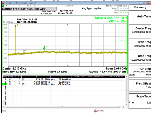
Band71_20MHz_DFT_s_OFDM_SCS15kHz_BPSK_RB1_1_CH137600
