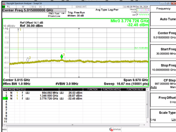
Band71_20MHz_DFT_s_OFDM_SCS15kHz_BPSK_RB1_1_CH136100
