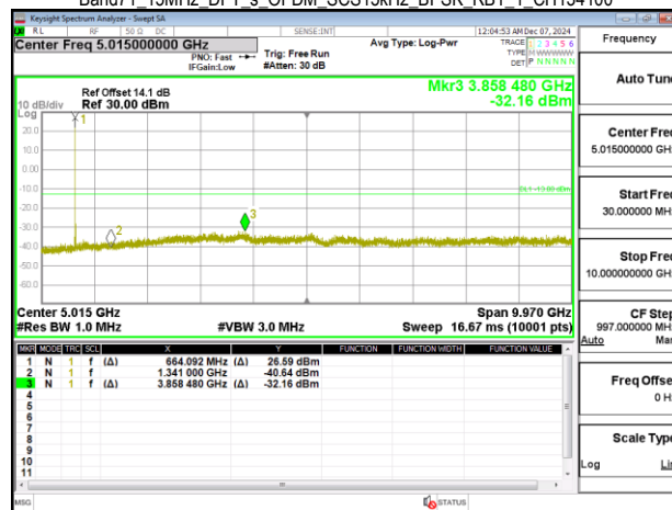
Band71 15MHz DFT s OFDM SCS15kHz BPSK RB1 1 CH136100
