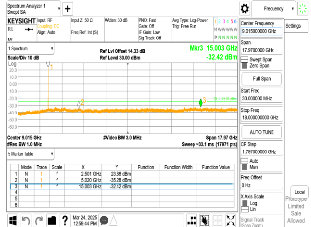
Band41_20MHz_DFT_s_OFDM_SCS30kHz_BPSK_RB1_1_CH502002upper 18G
