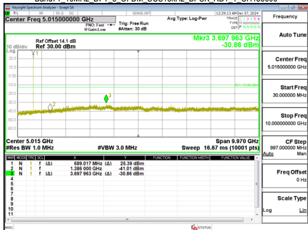
Band71_10MHz_DFT_s_OFDM_SCS15kHz_BPSK_RB1_1_CH138600
