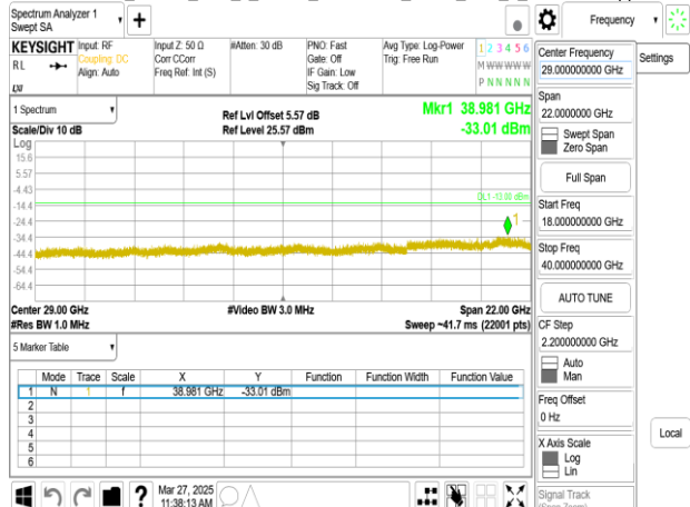
Band77-Part27_15MHz_DFT_s_OFDM_SCS30kHz_BPSK_RB1_1_CH664832upper 18G
