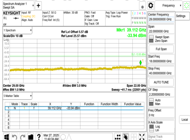
Band77-Part27_10MHz_DFT_s_OFDM_SCS30kHz_BPSK_RB1_1_CH665000upper 18G
