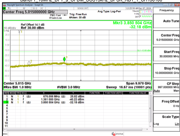
Band71_10MHz_DFT_s_OFDM_SCS15kHz_BPSK_RB1_1_CH138600
