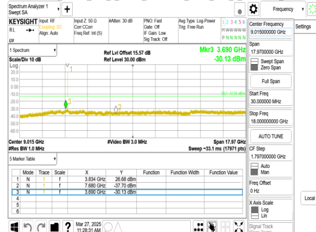
Band77-Part27_15MHz_DFT_s_OFDM_SCS30kHz_BPSK_RB1_1_CH656000_below 18G
