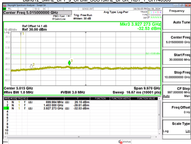
Band12 5MHz DFT s OFDM SCS15kHz BPSK RB1 1 CH141500
