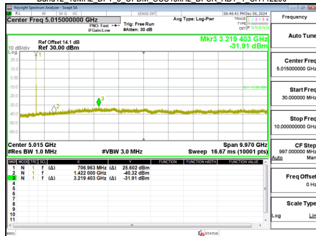
Band12 10MHz DFT s OFDM SCS15kHz BPSK RB1 1 CH142200
