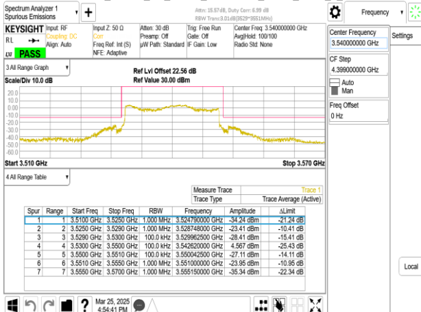
Band77-Part27_20MHz_CP_OFDM_SCS30kHz_QPSK_RB51_0_CH636000
