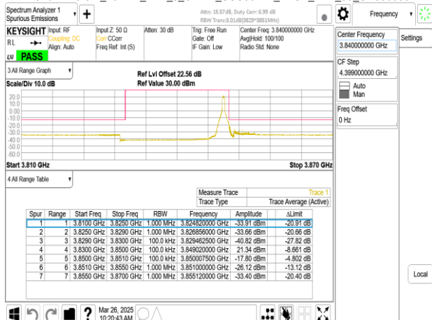
Band77-Part27_20MHz_DFT_s_OFDM_SCS30kHz_BPSK_RB50_0_CH656000
