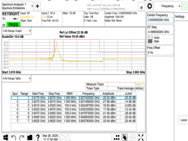
Band77-Part27_15MHz_CP_OFDM_SCS30kHz_QPSK_RB1_37_CH656000
