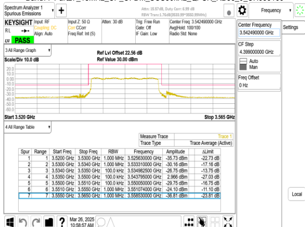
Band77-Part27_15MHz_CP_OFDM_SCS30kHz_QPSK_RB38_0_CH636166
