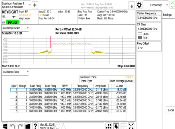
Band77-Part27_20MHz_CP_OFDM_SCS30kHz_QPSK_RB51_0_CH656000
