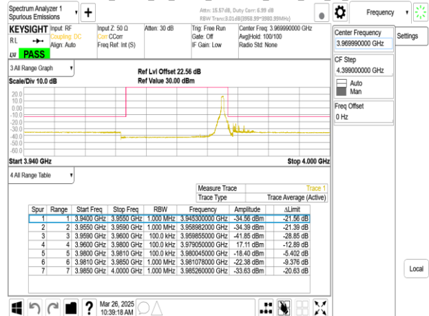
Band77-Part27_20MHz_CP_OFDM_SCS30kHz_QPSK_RB51_0_CH664666
