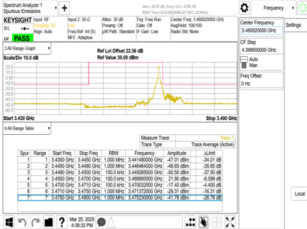
Band77-Part27_20MHz_DFT_s_OFDM_SCS30kHz_BPSK_RB50_0_CH630668
