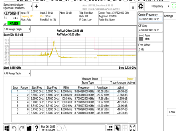
Band77-Part27_15MHz_CP_OFDM_SCS30kHz_QPSK_RB1_37_CH647168
