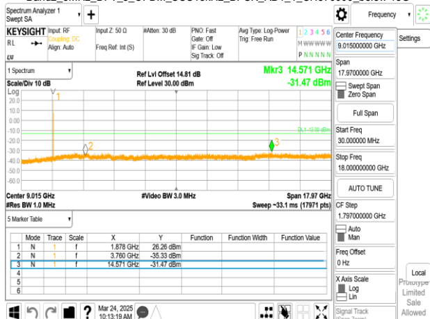
Band2_5MHz_DFT_s_OFDM_SCS15kHz_BPSK_RB1_1_CH376000_below 18G
