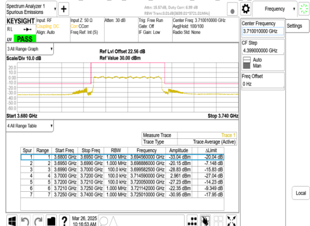
Band77-Part27_20MHz_CP_OFDM_SCS30kHz_QPSK_RB51_0_CH647334
