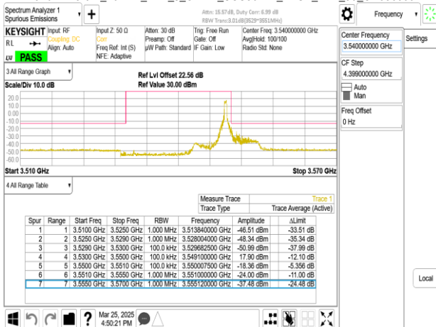
Band77-Part27_20MHz_DFT_s_OFDM_SCS30kHz_BPSK_RB50_0_CH636000
