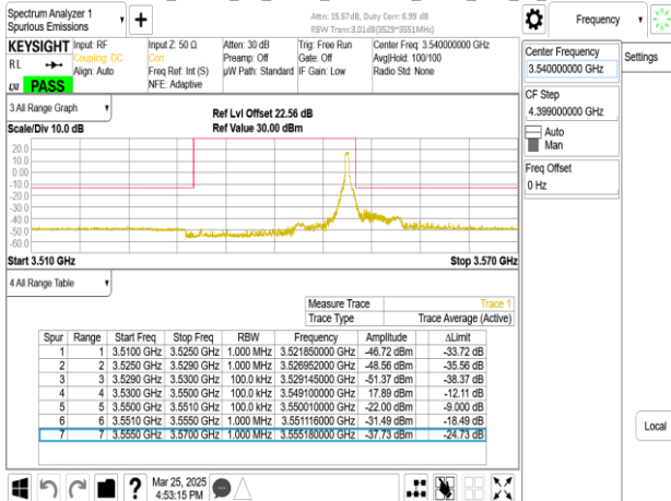
Band77-Part27_20MHz_CP_OFDM_SCS30kHz_QPSK_RB51_0_CH636000
