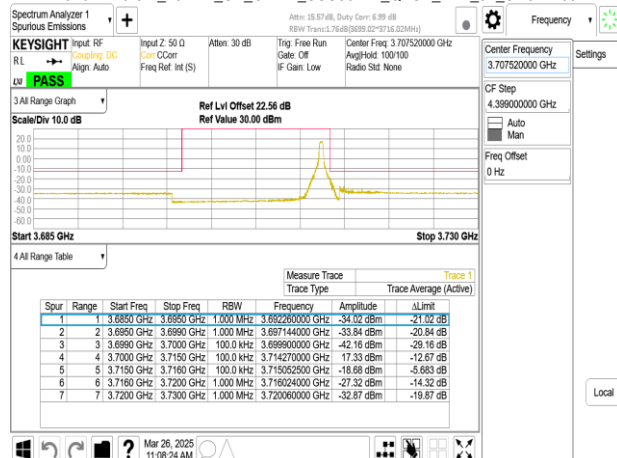
Band77-Part27_15MHz_CP_OFDM_SCS30kHz_QPSK_RB38_0_CH647168
