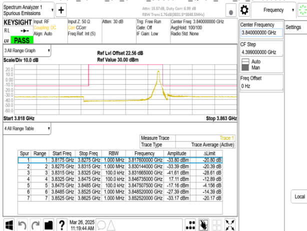
Band77-Part27_15MHz_CP_OFDM_SCS30kHz_QPSK_RB38_0_CH656000
