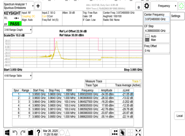
Band77-Part27_15MHz_CP_OFDM_SCS30kHz_QPSK_RB1_37_CH664832
