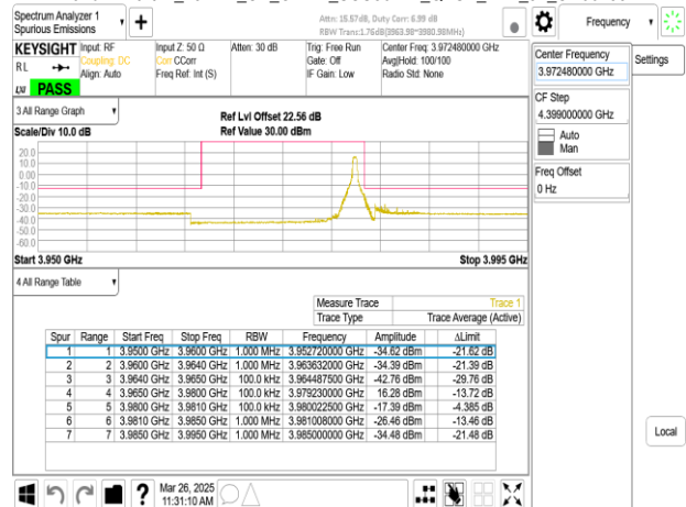
Band77-Part27_15MHz_CP_OFDM_SCS30kHz_QPSK_RB38_0_CH664832
