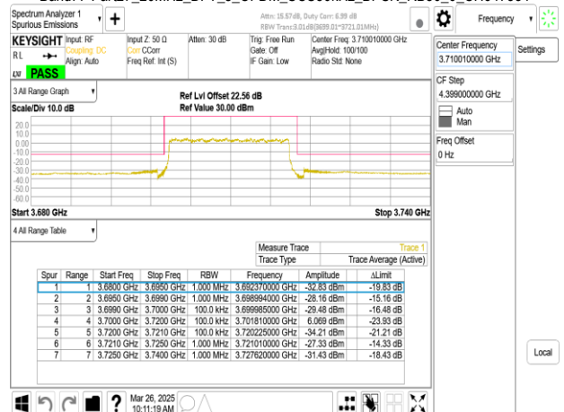
Band77-Part27_20MHz_DFT_s_OFDM_SCS30kHz_BPSK_RB50_0_CH647334
