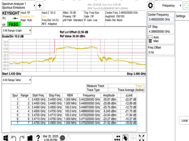
Band77-Part27_20MHz_DFT_s_OFDM_SCS30kHz_BPSK_RB50_0_CH630668
