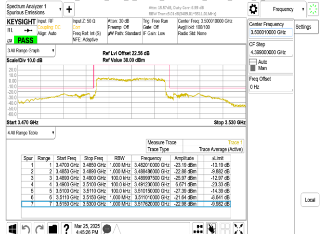
Band77-Part27_20MHz_DFT_s_OFDM_SCS30kHz_BPSK_RB50_0_CH633334
