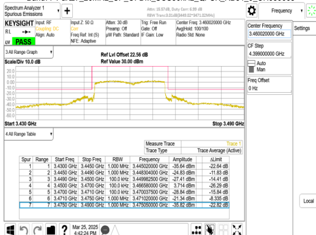
Band77-Part27_20MHz_CP_OFDM_SCS30kHz_QPSK_RB51_0_CH630668
