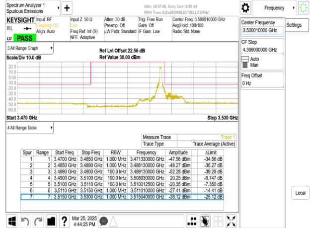
Band77-Part27_20MHz_DFT_s_OFDM_SCS30kHz_BPSK_RB50_0_CH633334
