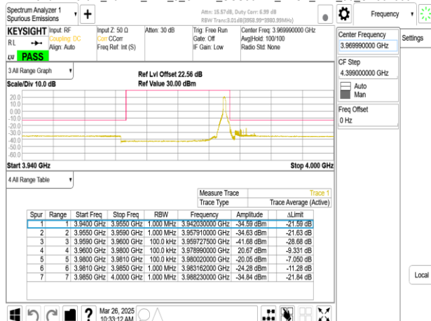
Band77-Part27_20MHz_DFT_s_OFDM_SCS30kHz_BPSK_RB50_0_CH664666
