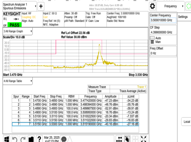
Band77-Part27_20MHz_CP_OFDM_SCS30kHz_QPSK_RB51_0_CH633334
