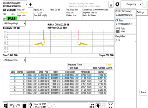
Band77-Part27_20MHz_CP_OFDM_SCS30kHz_QPSK_RB51_0_CH664666
