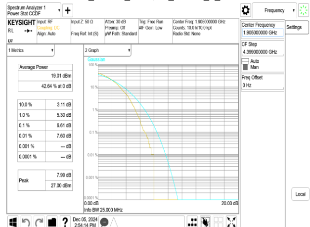
Band25_20MHz_256QAM_RB100_0_CH26590
