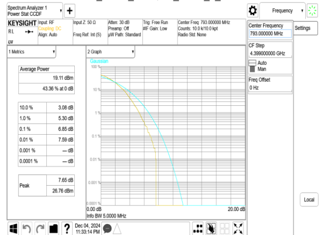
Band14_5MHz_256QAM_RB25_0_CH23330
