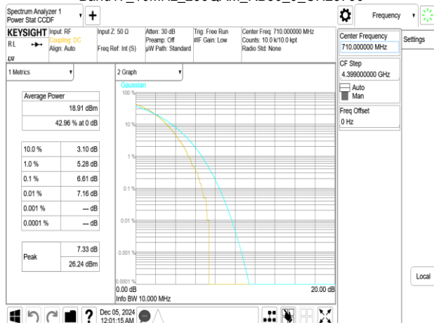
Band17_10MHz_256QAM_RB50_0_CH23800
