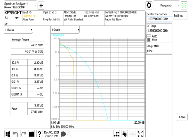
Band25_15MHz_QPSK_RB1_0_CH26615
