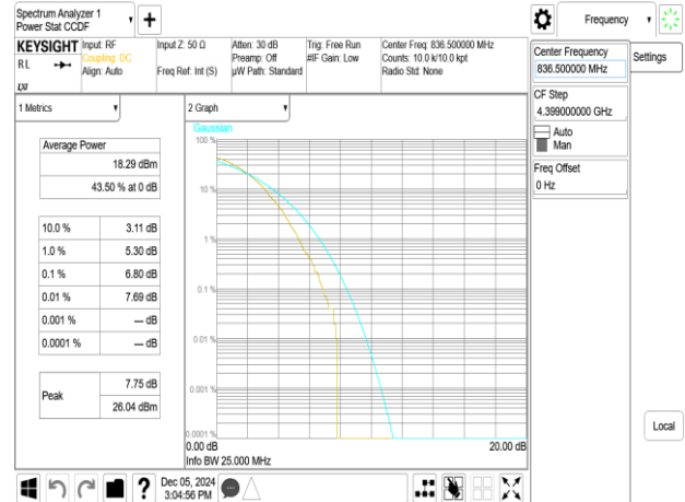
Band26_15MHz_256QAM_RB75_0_CH26915
