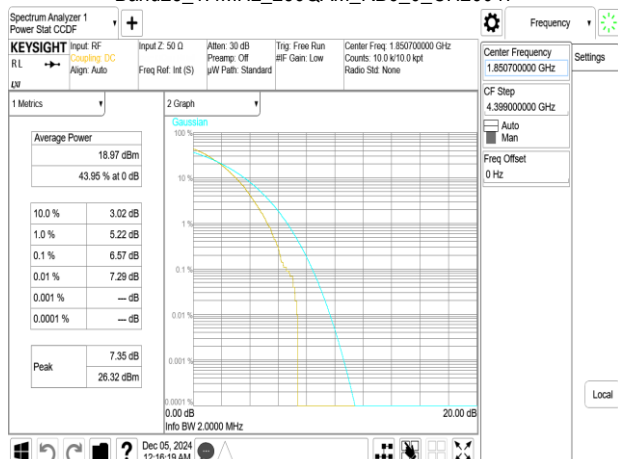
Band25_1.4MHz_256QAM_RB6_0_CH26047
