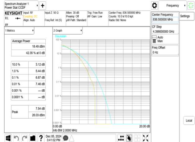
Band26_1.4MHz_256QAM_RB6_0_CH26915
