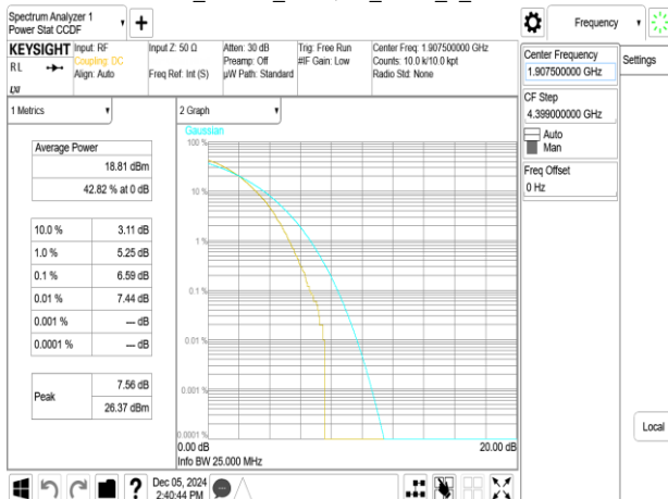
Band25_15MHz_256QAM_RB75_0_CH26615
