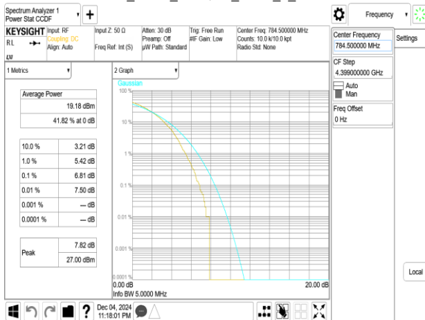
Band13_5MHz_256QAM_RB25_0_CH23255
