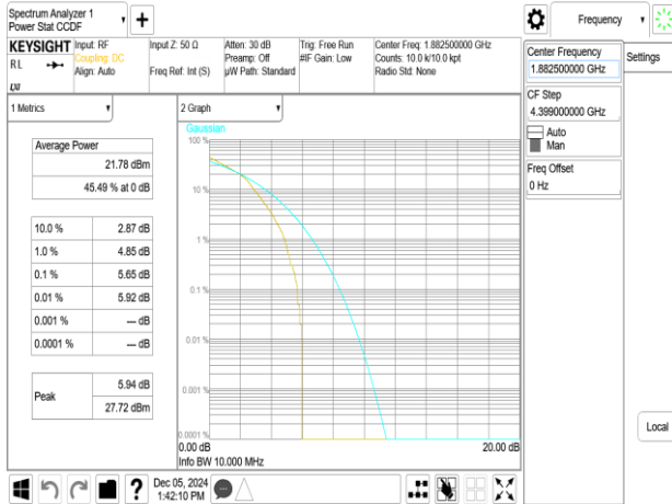
Band25_10MHz_64QAM_RB50_0_CH26365
