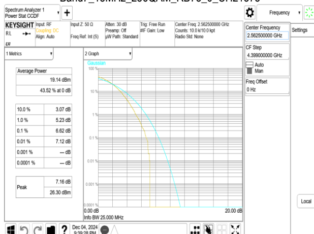
Band7_15MHz_256QAM_RB75_0_CH21375
