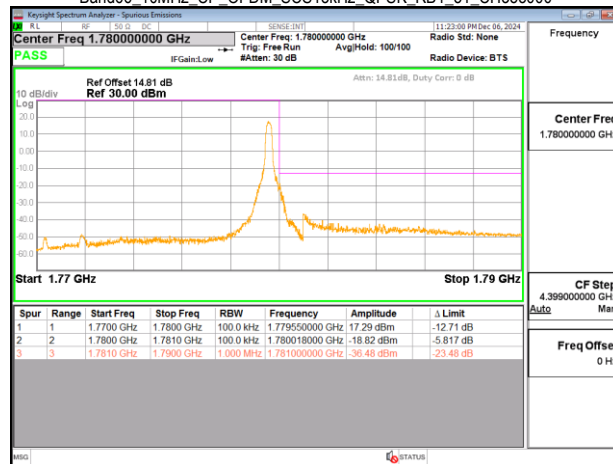
Band66_10MHz_CP_OFDM_SCS15kHz_QPSK_RB52_0_CH355000
