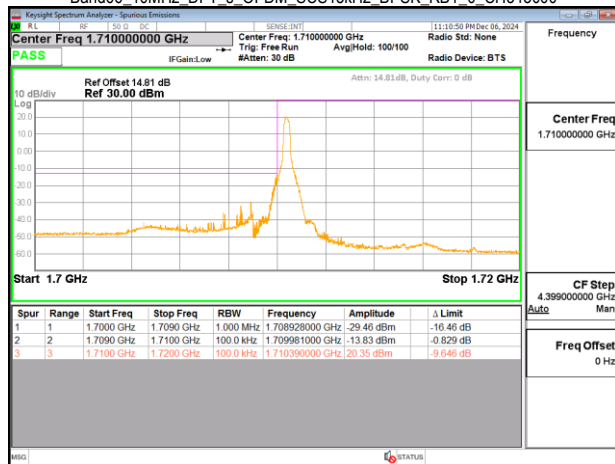
Band66_10MHz_DFT_s_OFDM_SCS15kHz_BPSK_RB50_0_CH343000
