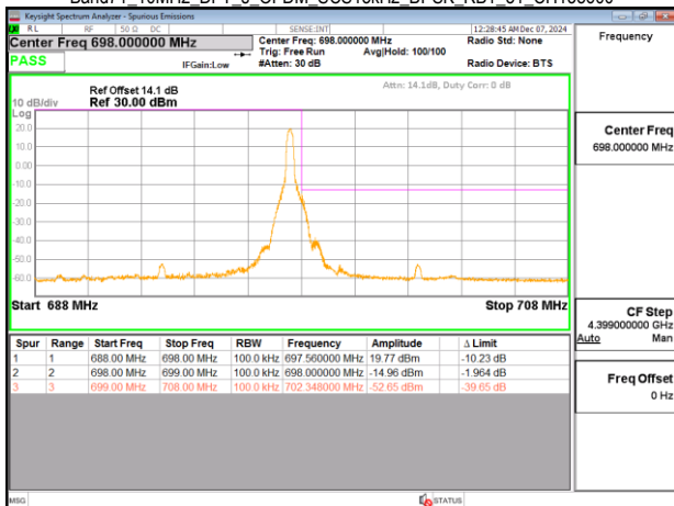
Band71_10MHz_DFT_s_OFDM_SCS15kHz_BPSK_RB1_51_CH138600
