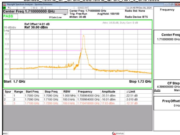
Band66_10MHz_CP_OFDM_SCS15kHz_QPSK_RB1_0_CH343000
