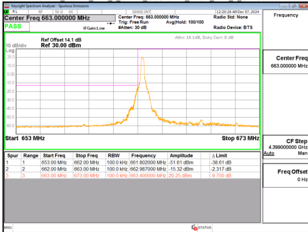
Band71_10MHz_DFT_s_OFDM_SCS15kHz_BPSK_RB50_0_CH133600
