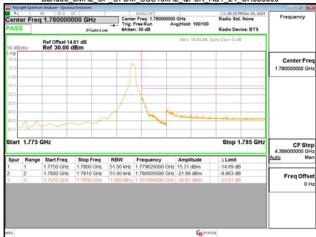
Band66_5MHz_CP_OFDM_SCS15kHz_QPSK_RB1_24_CH355500
