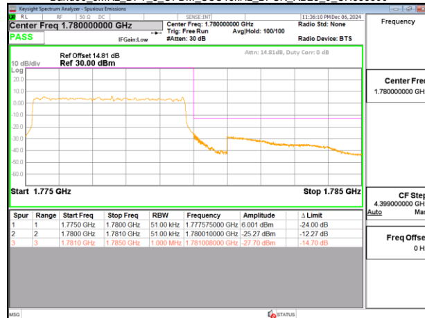
Band66_5MHz_DFT_s_OFDM_SCS15kHz_BPSK_RB25_0_CH355500
