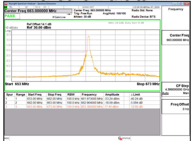
Band71_10MHz_CP_OFDM_SCS15kHz_QPSK_RB52_0_CH133600
