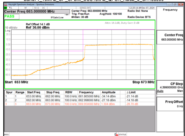
Band71_10MHz_CP_OFDM_SCS15kHz_QPSK_RB52_0_CH133600
