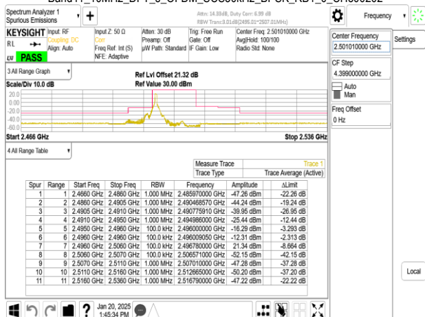
Band41_10MHz_DFT_s_OFDM_SCS30kHz_BPSK_RB1_0_CH500202
