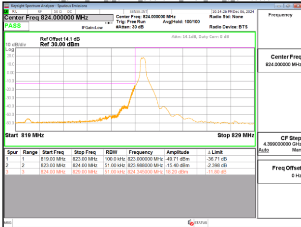
Band26 5MHz DFT s OFDM SCS15kHz BPSK RB25 0 CH165300
