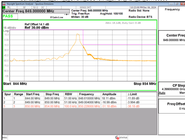
Band26 5MHz DFT s OFDM SCS15kHz BPSK RB1 24 CH169300
