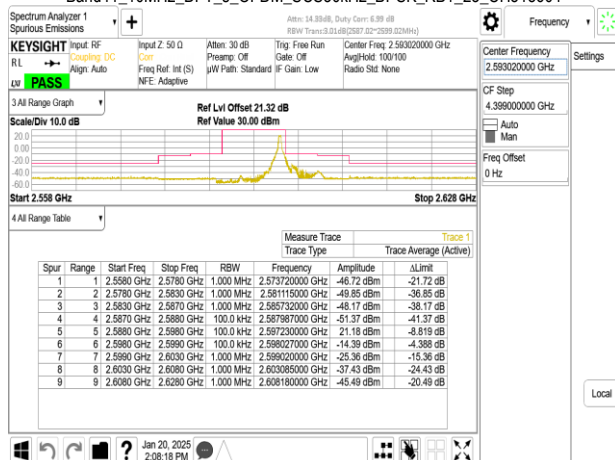
Band41_10MHz_DFT_s_OFDM_SCS30kHz_BPSK_RB24_0_CH518604
