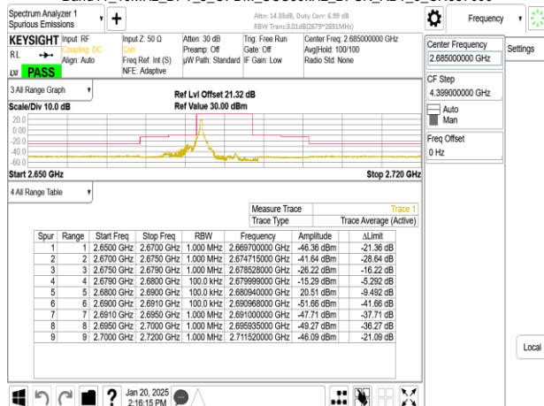
Band41_10MHz_DFT_s_OFDM_SCS30kHz_BPSK_RB1_0_CH537000
