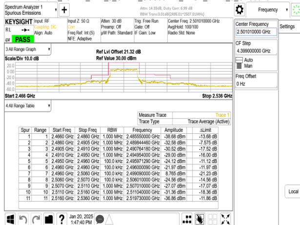
Band41_10MHz_DFT_s_OFDM_SCS30kHz_BPSK_RB1_0_CH501000
