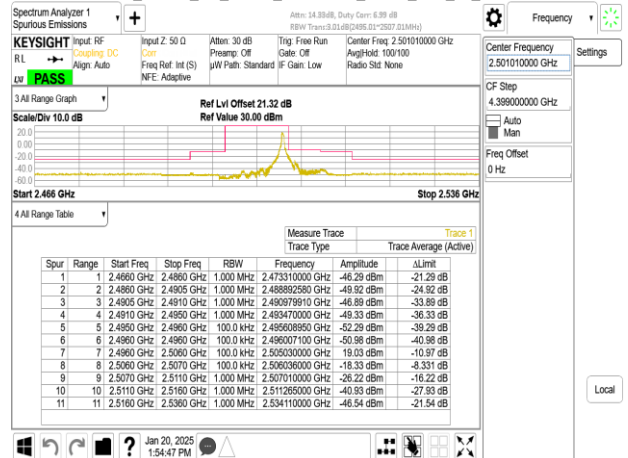
Band41_10MHz_CP_OFDM_SCS30kHz_QPSK_RB24_0_CH500202
