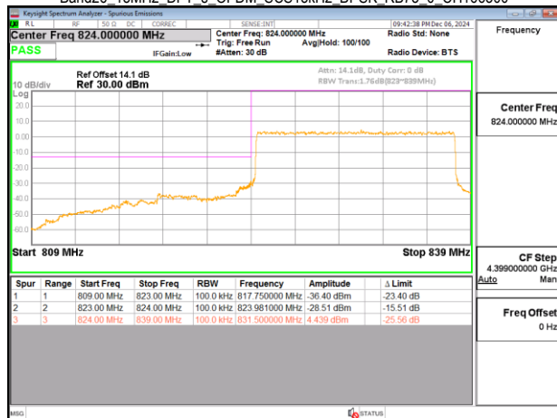
Band26_15MHz_DFT_s_OFDM_SCS15kHz_BPSK_RB75_0_CH166300
