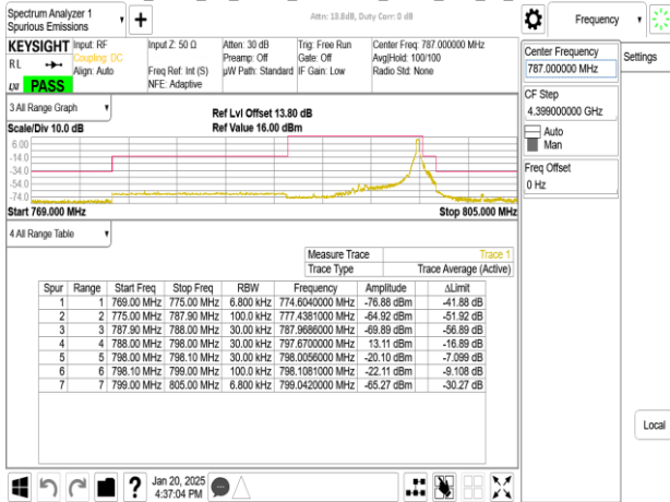
Band14_5MHz_CP_OFDM_SCS15kHz_QPSK_RB25_0_CH159100
