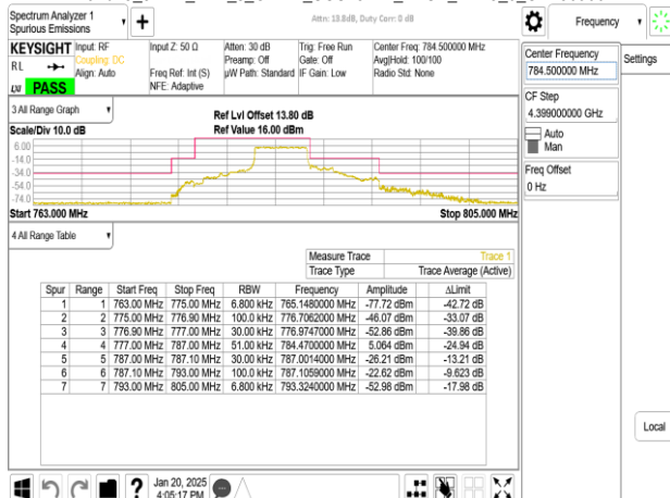
Band13_5MHz_CP_OFDM_SCS15kHz_QPSK_RB1_0_CH155900
