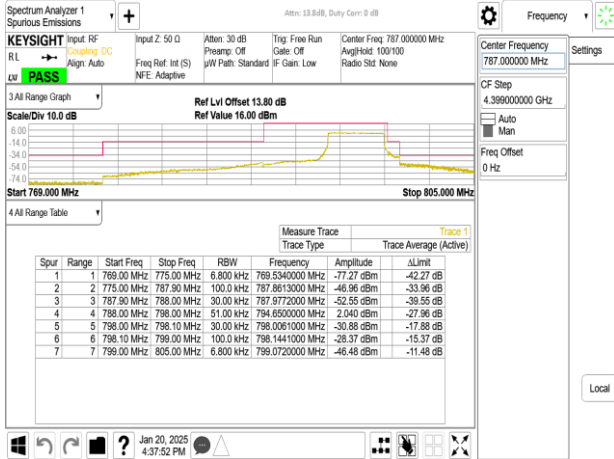
Band14_10MHz_DFT_s_OFDM_SCS15kHz_BPSK_RB1_0_CH158600
