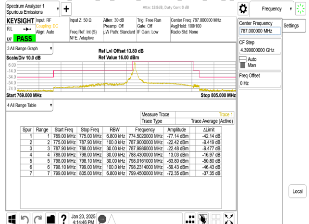
Band14_10MHz_CP_OFDM_SCS15kHz_QPSK_RB1_0_CH158600
