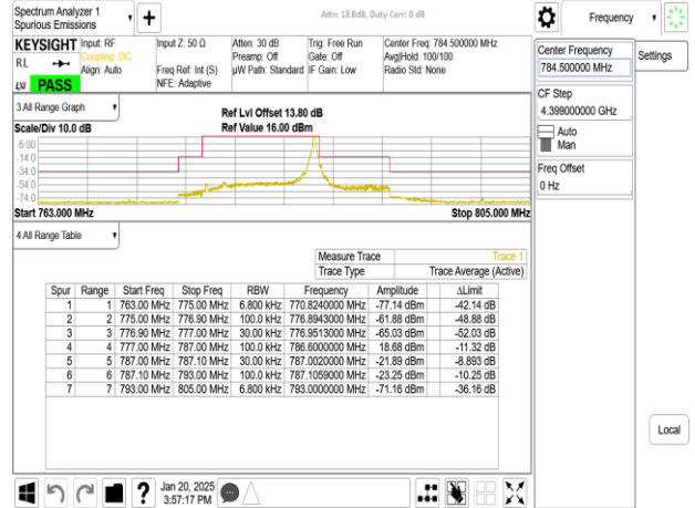
Band13_10MHz_CP_OFDM_SCS15kHz_QPSK_RB50_0_CH156400
