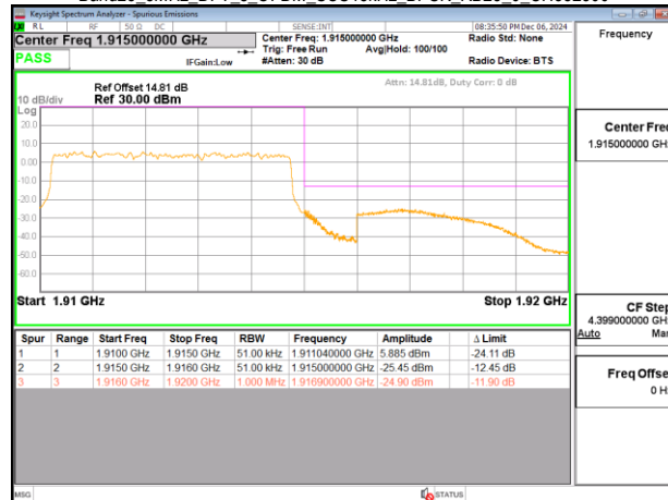
Band25_5MHz_DFT_s_OFDM_SCS15kHz_BPSK_RB25_0_CH382500
