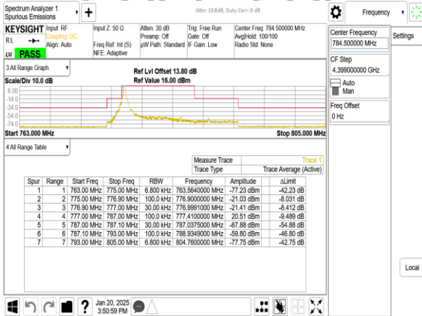
Band13_10MHz_DFT_s_OFDM_SCS15kHz_BPSK_RB1_51_CH156400
