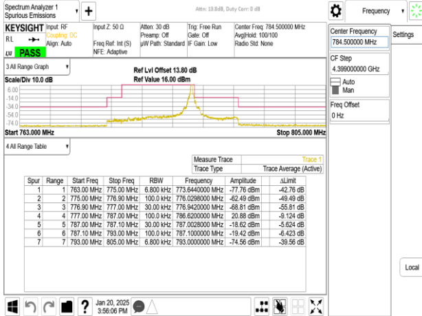
Band13_10MHz_DFT_s_OFDM_SCS15kHz_BPSK_RB50_0_CH156400
