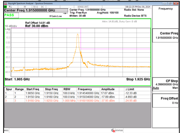
Band25_10MHz_CP_OFDM_SCS15kHz_QPSK_RB52_0_CH382000
