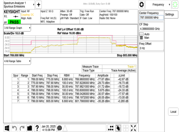
Band14_10MHz_CP_OFDM_SCS15kHz_QPSK_RB1_0_CH158600
