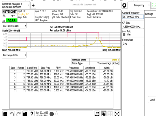
Band14_5MHz_DFT_s_OFDM_SCS15kHz_BPSK_RB1_24_CH159100
