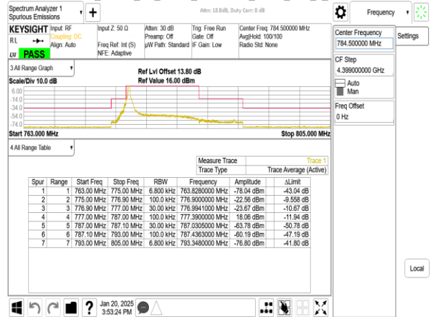
Band13_10MHz_CP_OFDM_SCS15kHz_QPSK_RB1_51_CH156400
