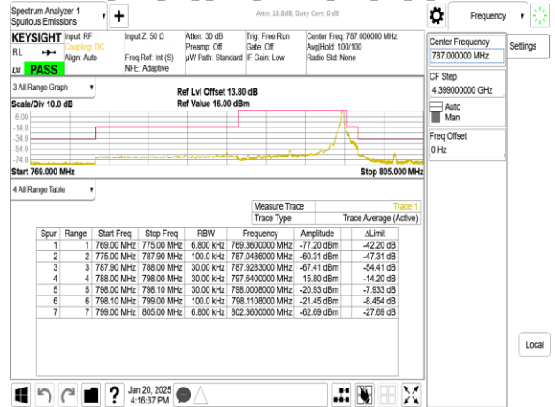
Band14_10MHz_DFT_s_OFDM_SCS15kHz_BPSK_RB50_0_CH158600
