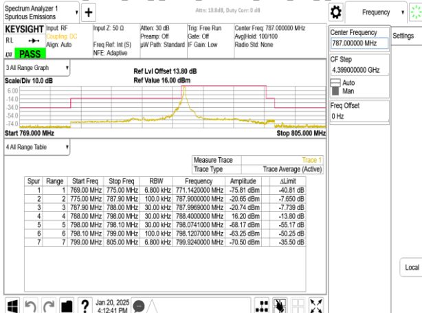
Band14_10MHz_DFT_s_OFDM_SCS15kHz_BPSK_RB1_0_CH158600
