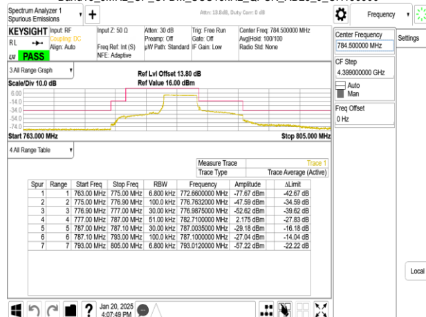
Band13_5MHz_CP_OFDM_SCS15kHz_QPSK_RB25_0_CH156900
