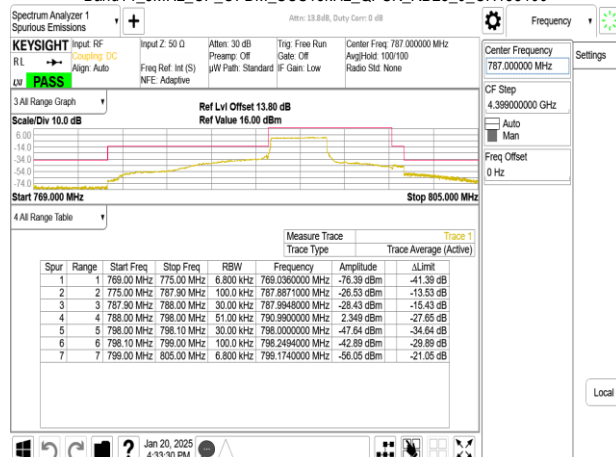
Band14_5MHz_CP_OFDM_SCS15kHz_QPSK_RB25_0_CH158100
