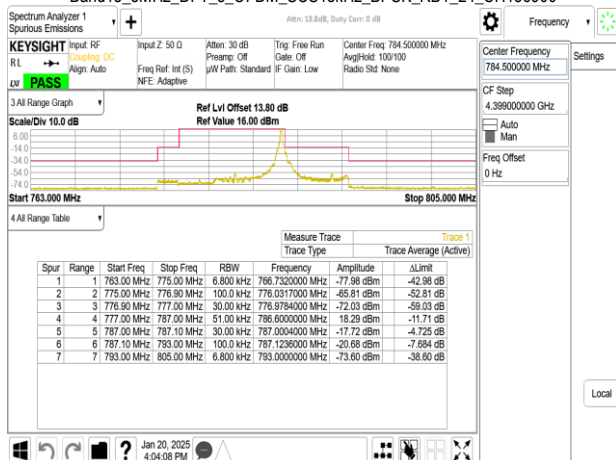
Band13_5MHz_DFT_s_OFDM_SCS15kHz_BPSK_RB25_0_CH156900
