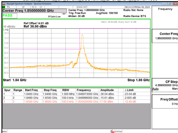
Band25_10MHz_CP_OFDM_SCS15kHz_QPSK_RB1_0_CH371000
