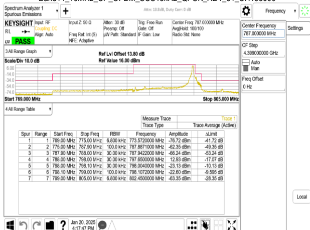
Band14_10MHz_CP_OFDM_SCS15kHz_QPSK_RB2_0_CH158600
