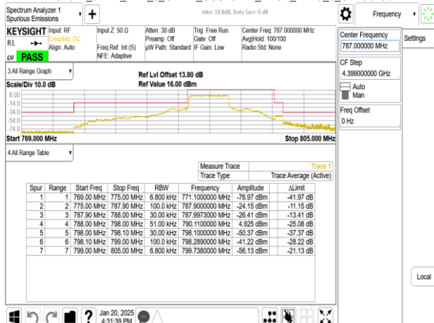
Band14_5MHz_DFT_s_OFDM_SCS15kHz_BPSK_RB1_24_CH159100
