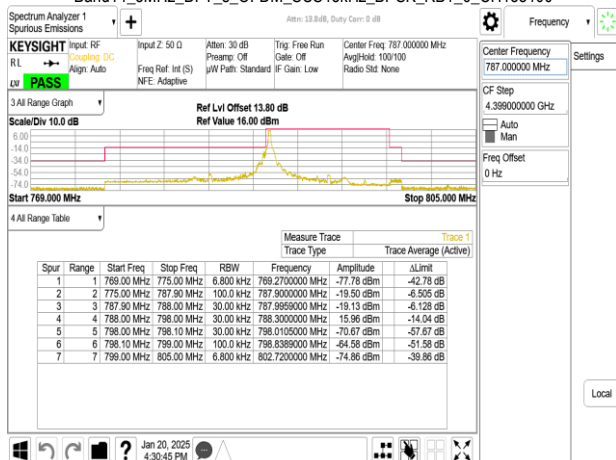
Band14_5MHz_DFT_s_OFDM_SCS15kHz_BPSK_RB25_0_CH158100
