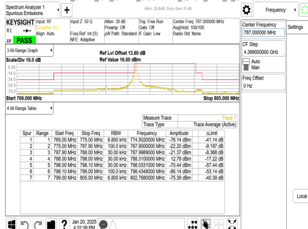
Band14_5MHz_CP_OFDM_SCS15kHz_QPSK_RB25_0_CH158100
