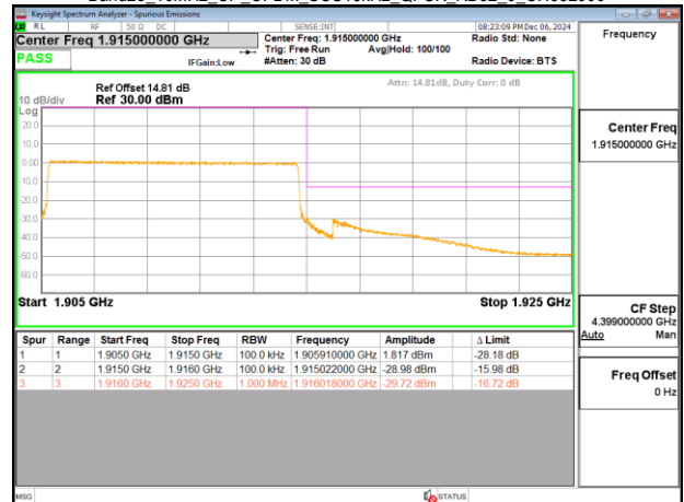
Band25_10MHz_CP_OFDM_SCS15kHz_QPSK_RB52_0_CH382000
