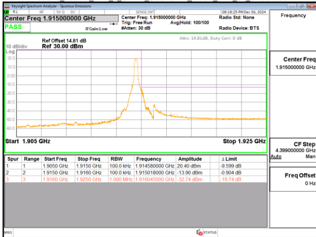
Band25_10MHz_DFT_s_OFDM_SCS15kHz_BPSK_RB50_0_CH382000
