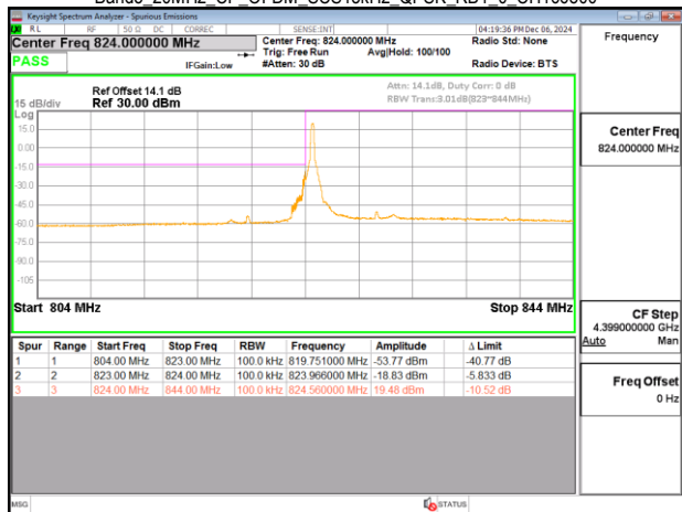
Band5_20MHz_CP_OFDM_SCS15kHz_QPSK_RB106_0_CH167800
