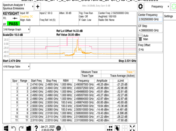
Band7_5MHz_DFT_s_OFDM_SCS15kHz_BPSK_RB1_24_CH500500
