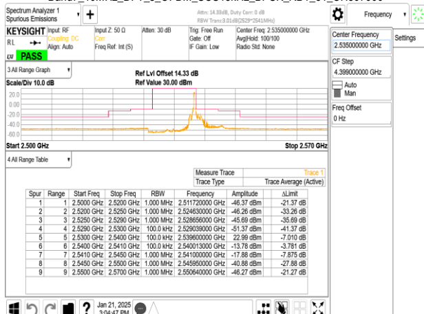
Band7_10MHz_DFT_s_OFDM_SCS15kHz_BPSK_RB1_51_CH507000
