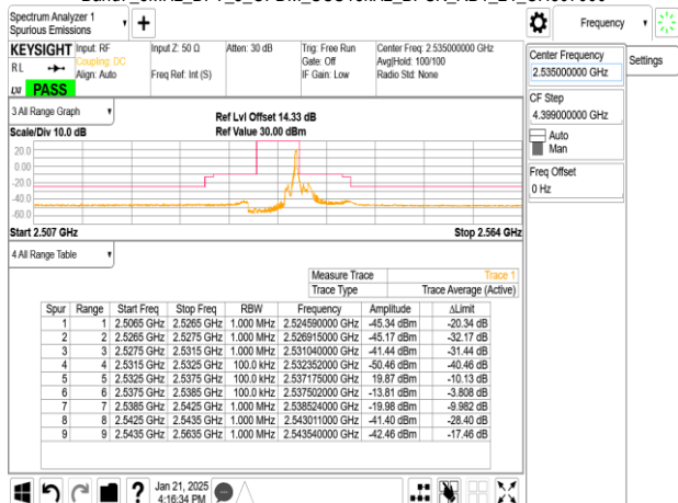
Band7_5MHz_DFT_s_OFDM_SCS15kHz_BPSK_RB1_24_CH507000
