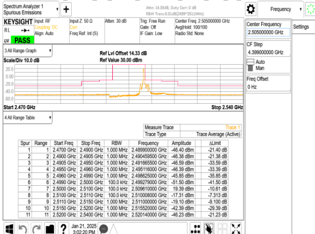
Band7_10MHz_CP_OFDM_SCS15kHz_QPSK_RB1_51_CH501000
