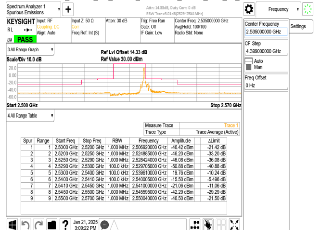
Band7_10MHz_CP_OFDM_SCS15kHz_QPSK_RB1_51_CH507000
