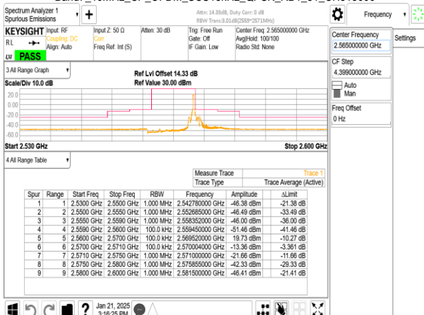
Band7_10MHz_CP_OFDM_SCS15kHz_QPSK_RB1_51_CH513000
