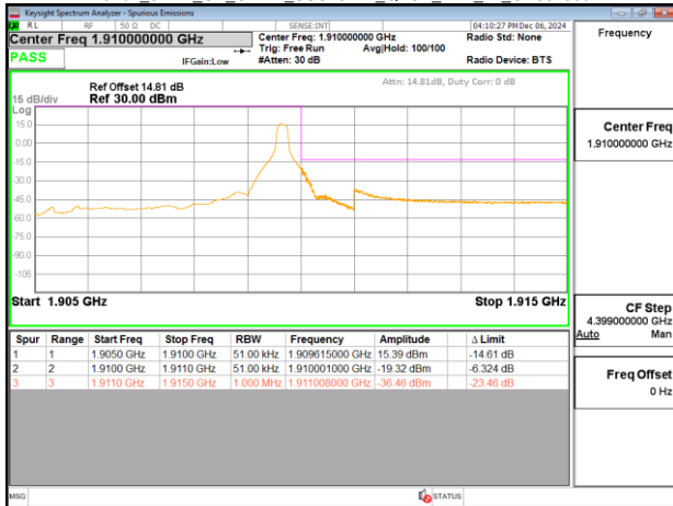
Band2_5MHz_CP_OFDM_SCS15kHz_QPSK_RB25_0_CH381500
