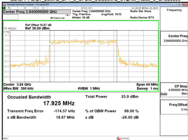
Band77-Part27_20MHz DFT s OFDM SCS30kHz 64QAM RB50_0 CH656000
