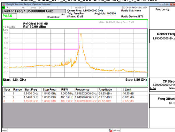
Band2_10MHz_DFT_s_OFDM_SCS15kHz_BPSK_RB1_0_CH371000
