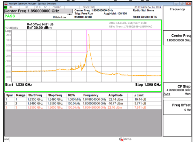
Band2_15MHz_DFT_s_OFDM_SCS15kHz_BPSK_RB75_0_CH371500
