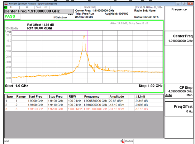
Band2_10MHz_DFT_s_OFDM_SCS15kHz_BPSK_RB50_0_CH381000
