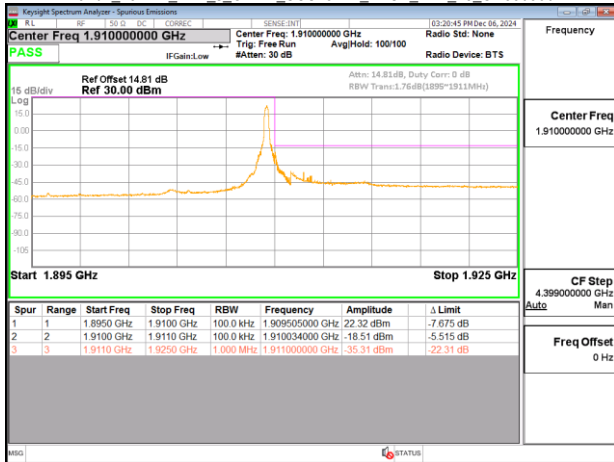
Band2_15MHz DFT s_OFDM_SCS15kHz BPSK RB75_0_CH380500
