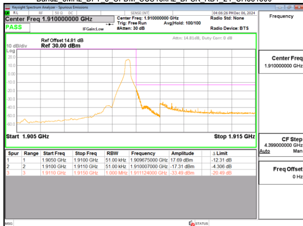
Band2_5MHz_DFT_s_OFDM_SCS15kHz_BPSK_RB1_24_CH381500
