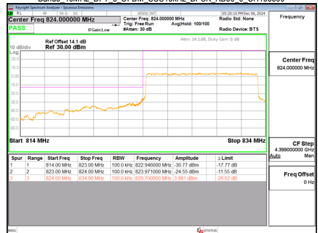
Band5 10MHz DFT s OFDM SCS15kHz BPSK RB50 0 CH165800
