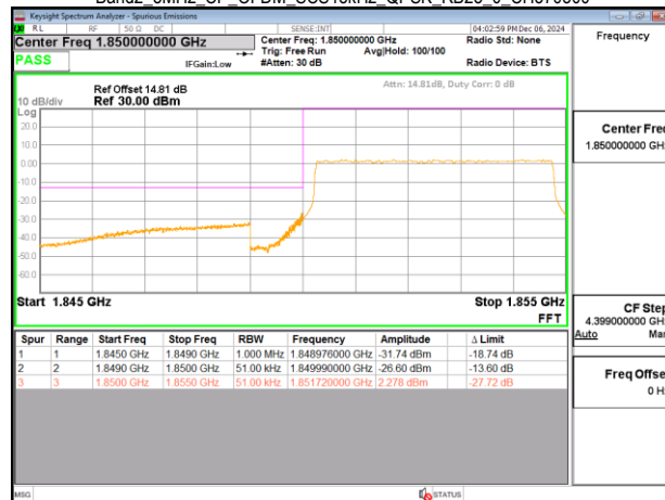
Band2_5MHz_CP_OFDM_SCS15kHz_QPSK_RB25_0_CH370500
