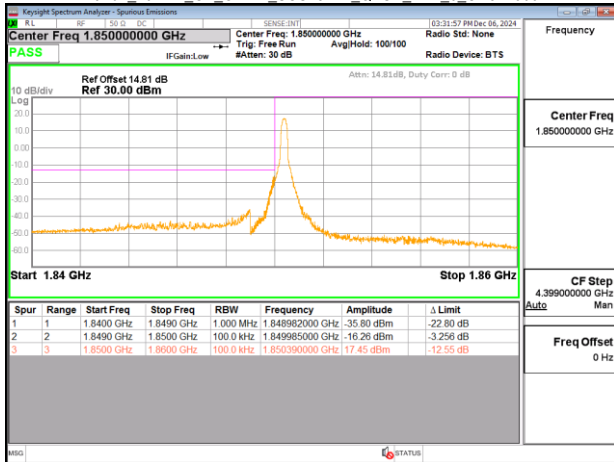
Band2_10MHz_CP_OFDM_SCS15kHz_QPSK_RB52_0_CH371000
