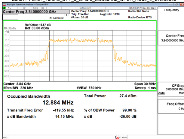
Band77-Part27_15MHz_DFT_s_OFDM_SCS30kHz_QPSK_RB36_0_CH656000
