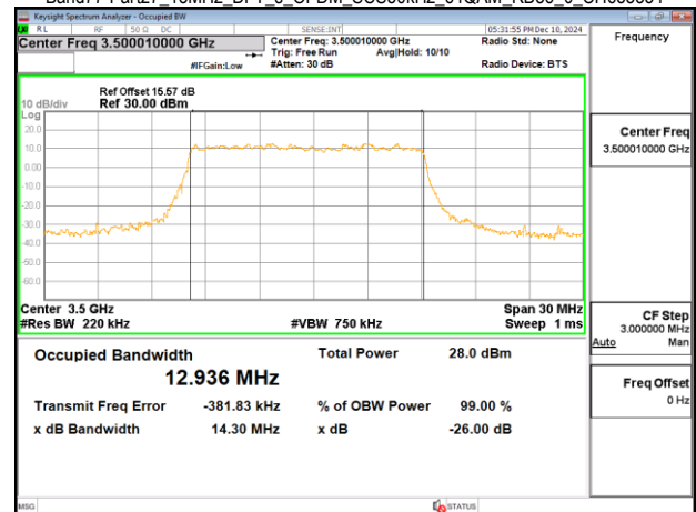
Band77-Part27 15MHz DFT s OFDM SCS30kHz 64QAM RB36 0 CH633334
