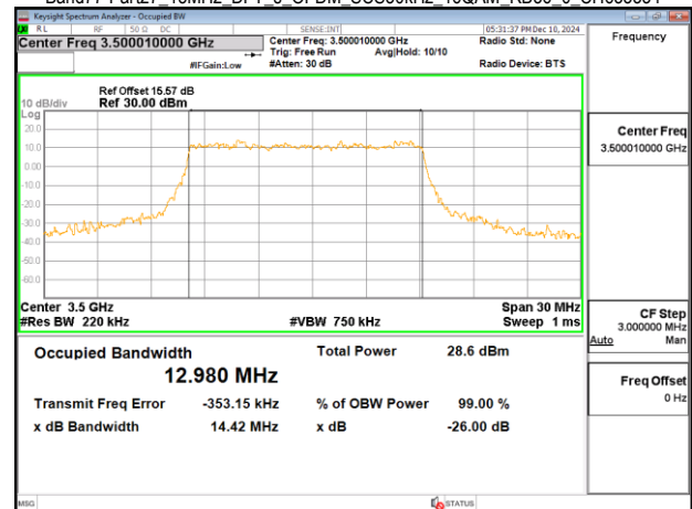
Band77-Part27_15MHz_DFT_s_OFDM_SCS30kHz_16QAM_RB36_0_CH633334
