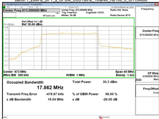
Band71 20MHz DFT s OFDM SCS15kHz 16QAM RB100_0 CH136100
