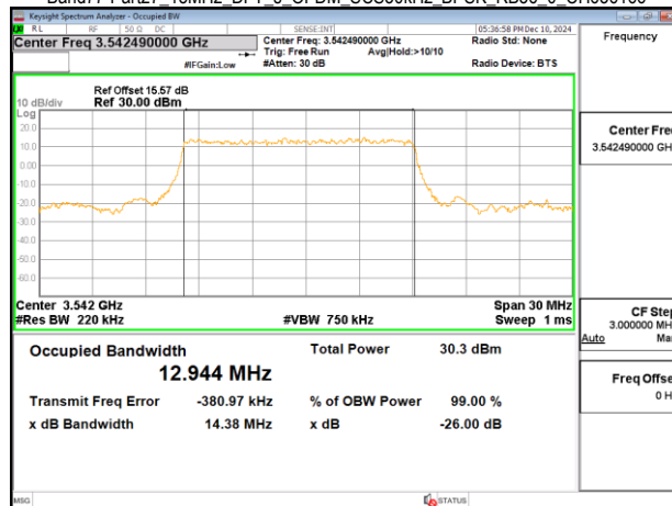
Band77-Part27 15MHz DFT s OFDM SCS30kHz BPSK RB36 0 CH636166
