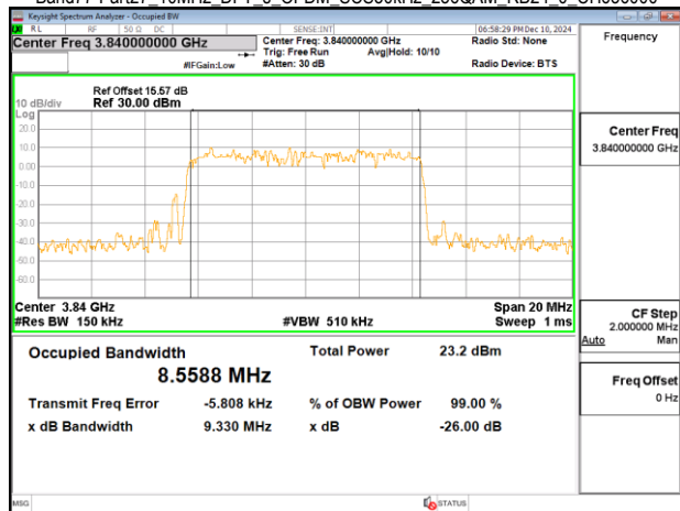
Band77-Part27 10MHz DFT s OFDM SCS30kHz 256QAM RB24 0 CH665000
