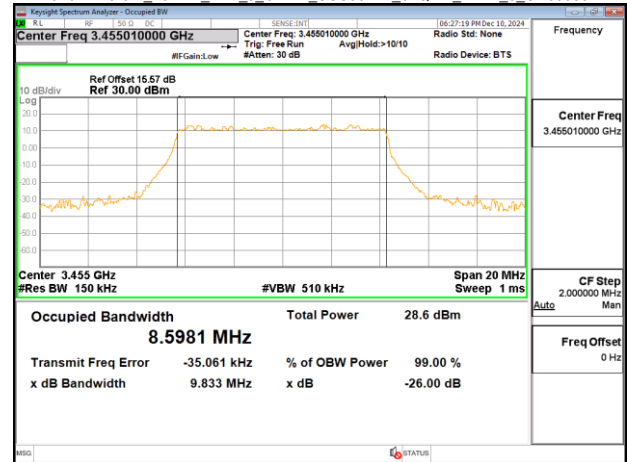
Band77-Part27 10MHz DFT s OFDM SCS30kHz 64QAM RB24 0 CH633334
