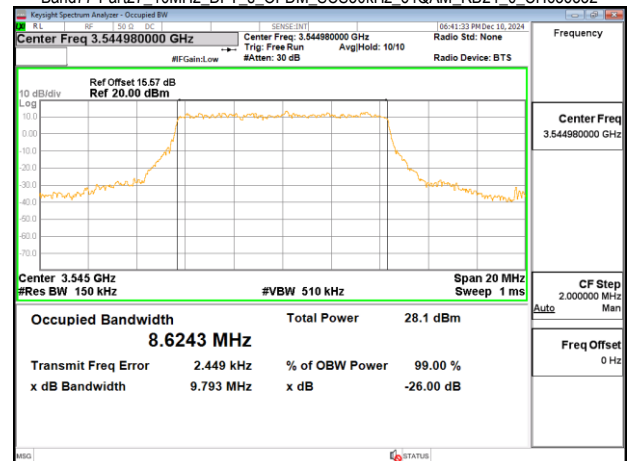
Band77-Part27 10MHz DFT s OFDM SCS30kHz 64QAM RB24 0 CH636332
