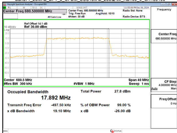
Band71 20MHz DFT s_OFDM_SCS15kHz 256QAM_RB100_0_CH137600
