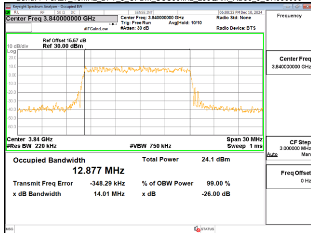
Band77-Part27 15MHz DFT s OFDM SCS30kHz 256QAM RB36_0 CH656000
