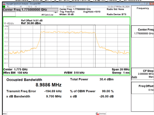
Band66_10MHz_DFT_s_OFDM_SCS15kHz_16QAM_RB50_0_CH355000
