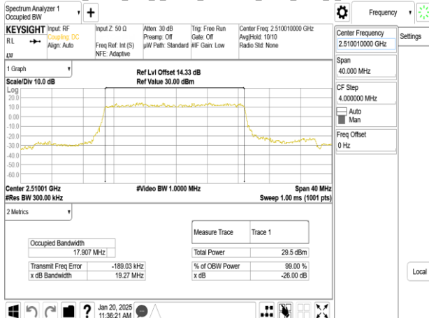
Band41_20MHz_DFT_s_OFDM_SCS30kHz_BPSK_RB50_0_CH502002
