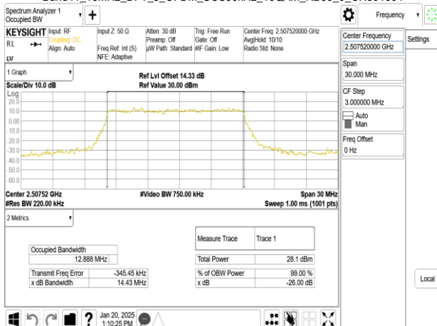
Band41_15MHz_DFT_s_OFDM_SCS30kHz_16QAM_RB36_0_CH501504
