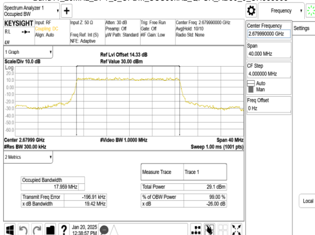
Band41_20MHz_DFT_s_OFDM_SCS30kHz_QPSK_RB50_0_CH535998
