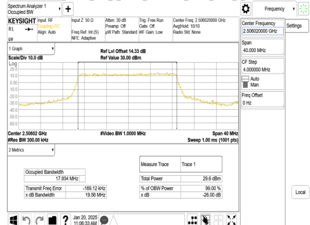
Band41_20MHz_DFT_s_OFDM_SCS30kHz_QPSK_RB50_0_CH501204
