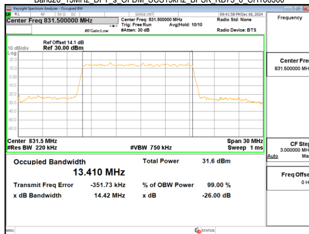
Band26 15MHz DFT s OFDM SCS15kHz BPSK RB75_0 CH167300
