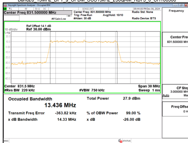
Band26 15MHz DFT s OFDM SCS15kHz 256QAM RB75_0 CH167300
