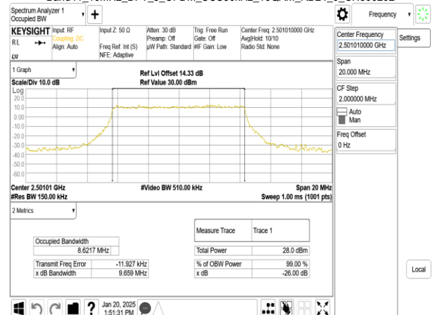
Band41_10MHz_DFT_s_OFDM_SCS30kHz_16QAM_RB24_0_CH500202
