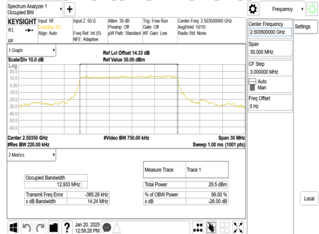
Band41_15MHz_DFT_s_OFDM_SCS30kHz_BPSK_RB36_0_CH500700
