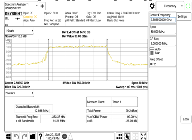
Band41_15MHz_DFT_s_OFDM_SCS30kHz_QPSK_RB36_0_CH501504
