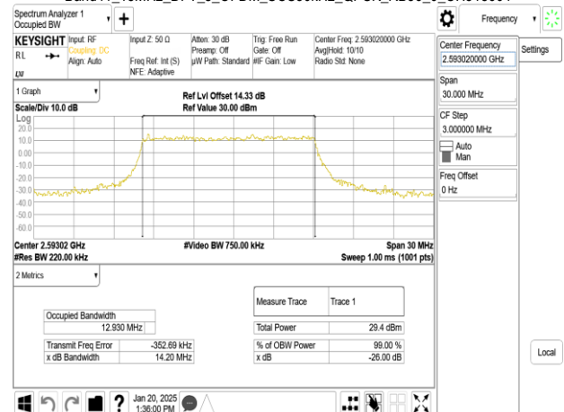
Band41_15MHz_DFT_s_OFDM_SCS30kHz_QPSK_RB36_0_CH518604
