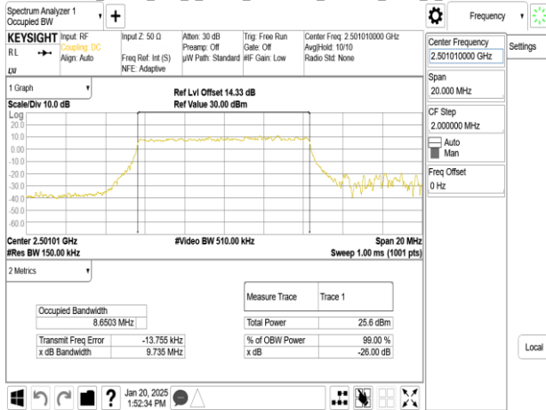
Band41_10MHz_DFT_s_OFDM_SCS30kHz_256QAM_RB24_0_CH501000
