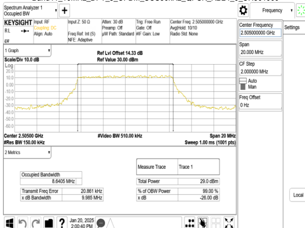
Band41_10MHz_DFT_s_OFDM_SCS30kHz_QPSK_RB24_0_CH501000
