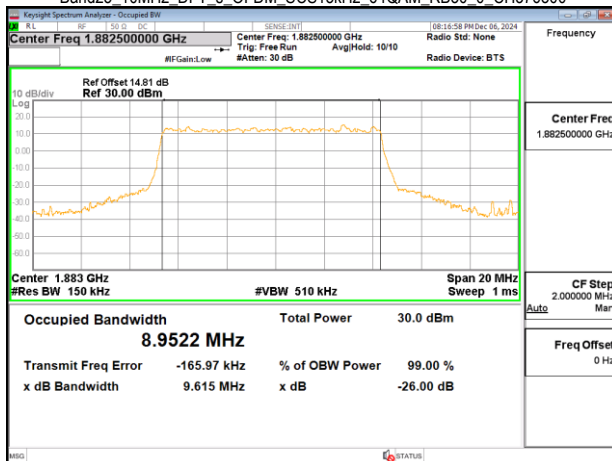
Band25_10MHz_DFT_s_OFDM_SCS15kHz_64QAM_RB50_0_CH376500
