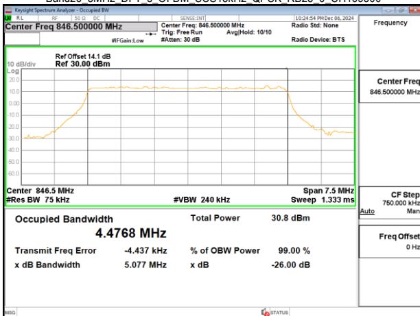
Band26_5MHz_DFT_s_OFDM_SCS15kHz_QPSK_RB25_0_CH169300
