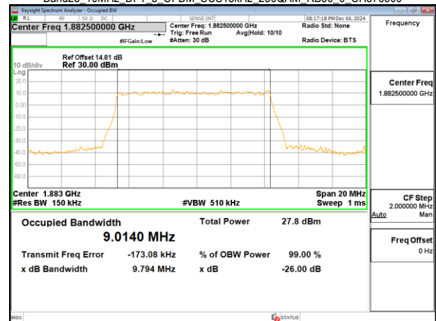
Band25_10MHz_DFT_s_OFDM_SCS15kHz_256QAM_RB50_0_CH376500
