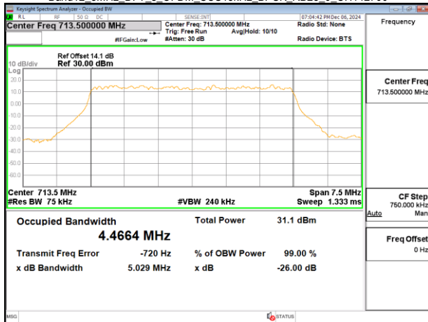
Band12_5MHz DFT s OFDM_SCS15kHz BPSK RB25_0_CH142700
