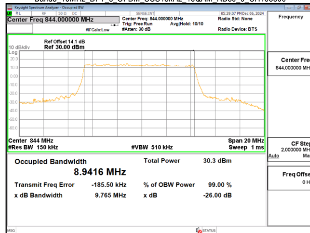
Band5_10MHz_DFT_s_OFDM_SCS15kHz_16QAM_RB50_0_CH168800
