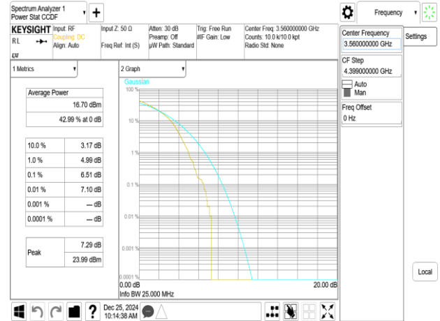
Band48_20MHz_256QAM_RB100_0_CH55990
