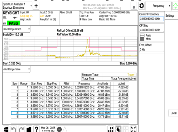
Band48_20MHz_DFT_s_OFDM_SCS30kHz_BPSK_RB50_0_CH637334
