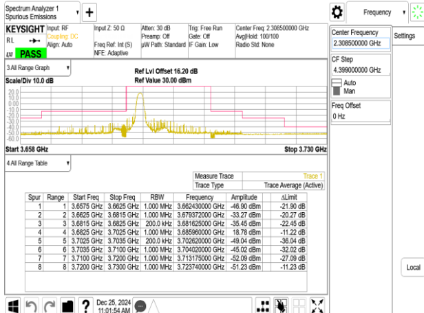
Emission Mask_Band48_15MHz_QPSK_RB1_0_CH56665
