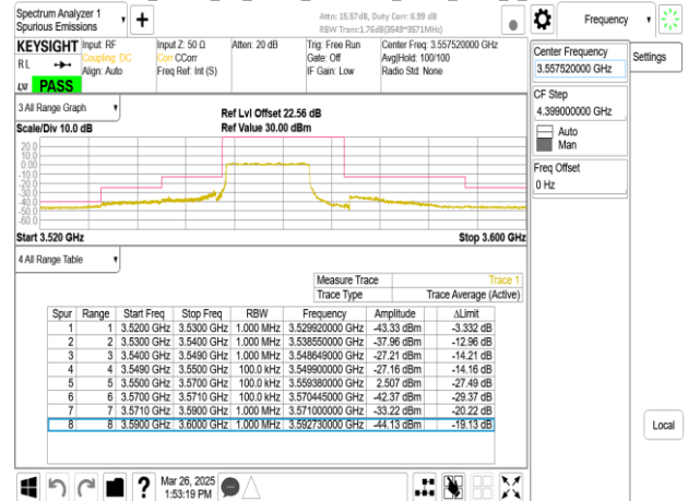
Band48_15MHz_CP_OFDM_SCS30kHz_QPSK_RB38_0_CH637168
