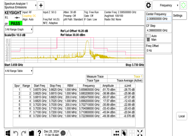
Emission Mask_Band48_15MHz_QPSK_RB1_74_CH56665
