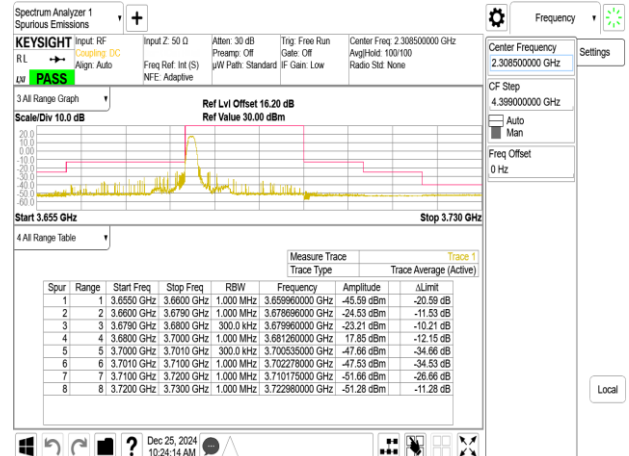
Emission Mask_Band48_20MHz_QPSK_RB1_0_CH56640
