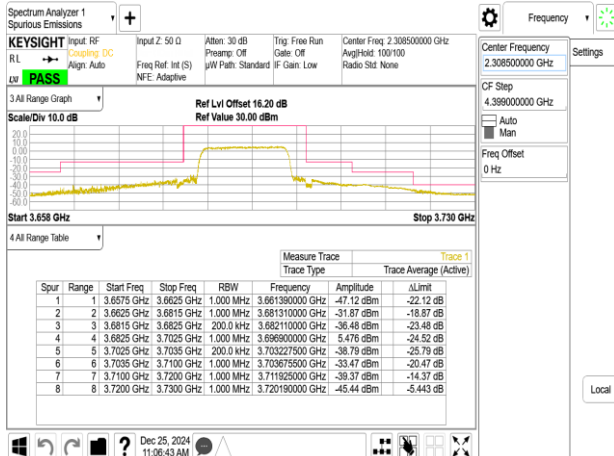
Emission Mask_Band48_15MHz_QPSK_RB75_0_CH56665
