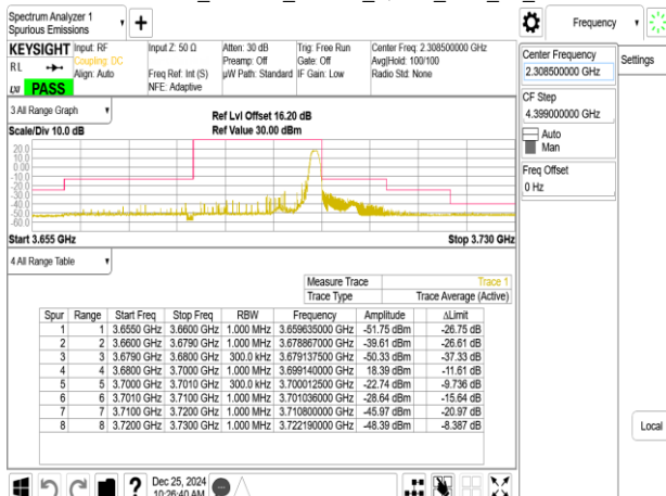
Emission Mask_Band48_20MHz_QPSK_RB1_99_CH56640
