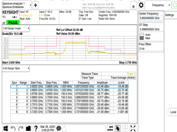
Band48_15MHz_DFT_s_OFDM_SCS30kHz_BPSK_RB36_0_CH646166
