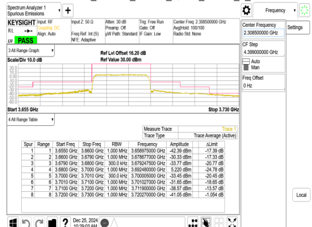
Emission Mask_Band48_20MHz_QPSK_RB100_0_CH56640
