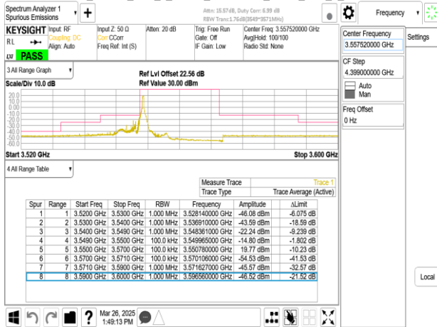
Band48_15MHz_DFT_s_OFDM_SCS30kHz_BPSK_RB1_37_CH637168
