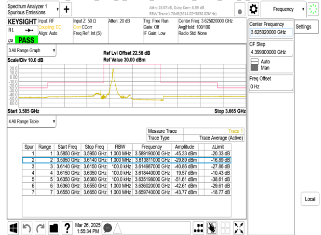
Band48_15MHz_DFT_s_OFDM_SCS30kHz_BPSK_RB1_37_CH641668
