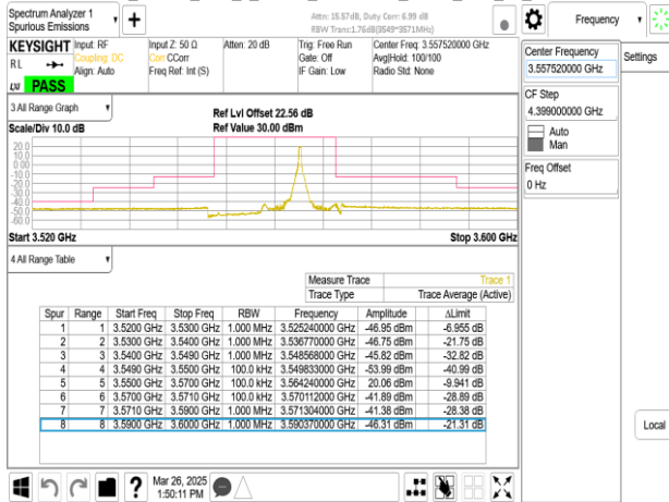
Band48_15MHz_DFT_s_OFDM_SCS30kHz_BPSK_RB36_0_CH637168
