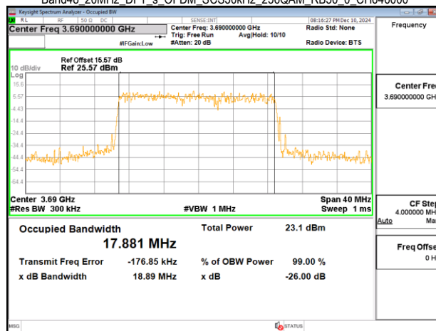
Band48 20MHz DFT s OFDM SCS30kHz 256QAM RB50_0 CH646000
