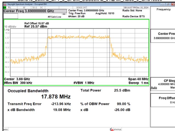
Band48 20MHz DFT s OFDM SCS30kHz 64QAM RB50_0 CH646000
