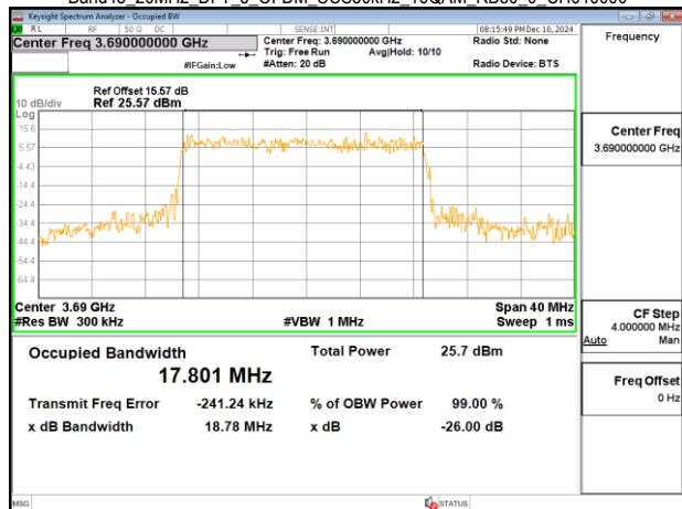
Band48 20MHz DFT s OFDM SCS30kHz 16QAM RB50_0 CH646000
