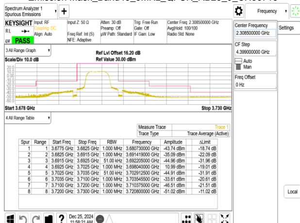
Emission Mask_Band48_5MHz_QPSK_RB25_0_CH56715
