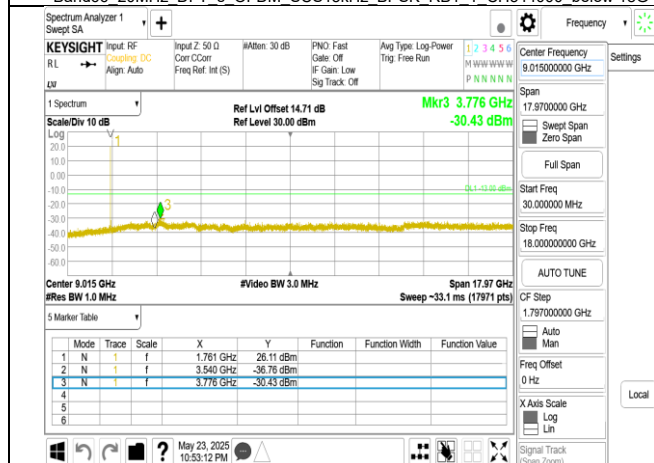
Band66 20MHz DFT s OFDM SCS15kHz BPSK RB1 1 CH354000 below 18G
