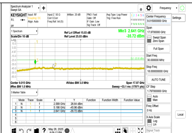
Band41_10MHz_DFT_s_OFDM_SCS30kHz_BPSK_RB1_1_CH518604_below 18G
