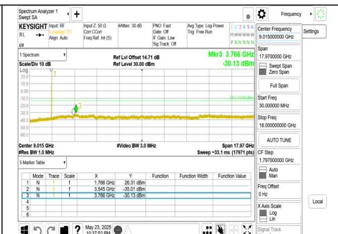
Band66 15MHz DFT s OFDM SCS15kHz BPSK RB1 1 CH354500 below 18G
