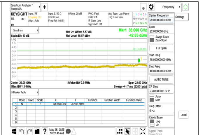
Band77-Part27_10MHz_DFT_s_OFDM_SCS30kHz_BPSK_RB1_1_CH647000_upper 18G
