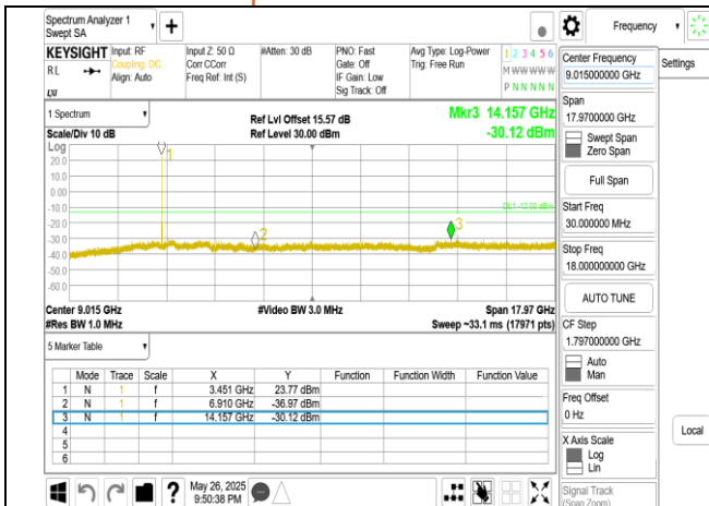
Band77-Part27_10MHz_DFT_s_OFDM_SCS30kHz_BPSK_RB1_1_CH630334_below 18G
