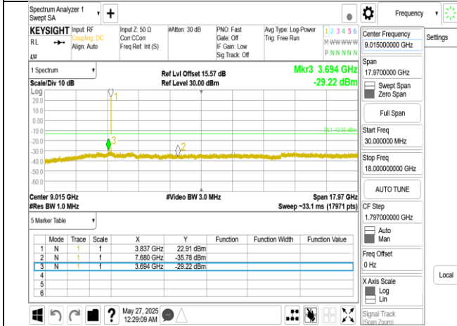
Band77-Part27_10MHz_DFT_s_OFDM_SCS30kHz_BPSK_RB1_1_CH656000_below 18G
