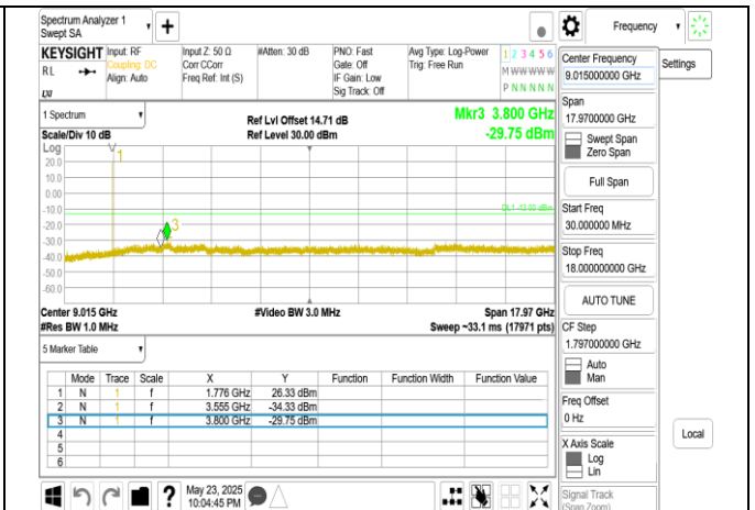
Band66 5MHz DFT s OFDM SCS15kHz BPSK RB1 1 CH355500 below 18G
