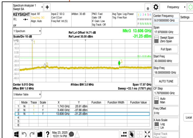
Band66 5MHz DFT s OFDM SCS15kHz BPSK RB1 1 CH349000 below 18G
