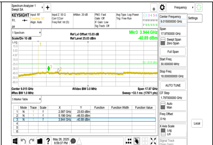
Band41_15MHz_DFT_s_OFDM_SCS30kHz_BPSK_RB1_1_CH518604_below_18G
