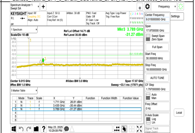
Band66 15MHz DFT s OFDM SCS15kHz BPSK RB1 1 CH343500 below 18G
