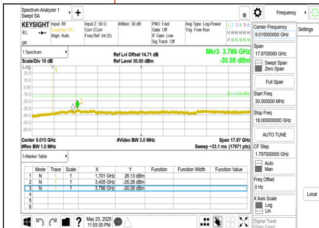
Band70 5MHz DFT s OFDM SCS15kHz BPSK RB1 1 CH340500 below 18G
