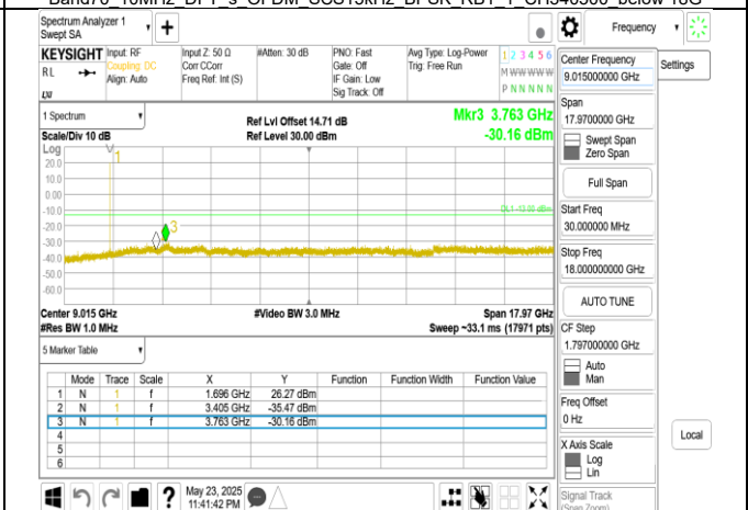
Band70 15MHz DFT s OFDM SCS15kHz BPSK RB1 1 CH340500 below 18G
