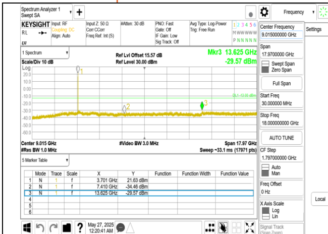
Band77-Part27_10MHz_DFT_s_OFDM_SCS30kHz_BPSK_RB1_1_CH647000_below 18G
