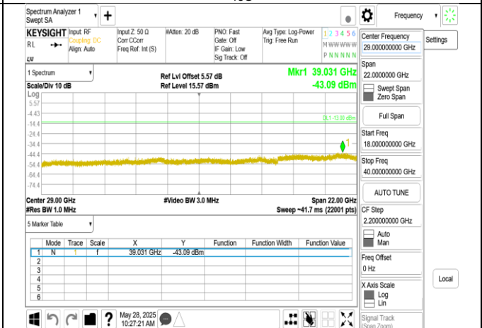
Band77-Part27_10MHz_DFT_s_OFDM_SCS30kHz_BPSK_RB1_1_CH636332_upper 18G
