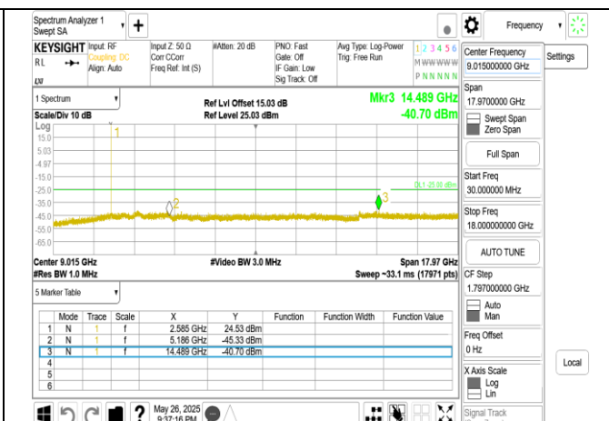
Band41_20MHz_DFT_s_OFDM_SCS30kHz_BPSK_RB1_1_CH518604_below 18G
