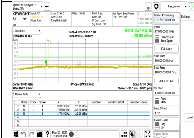
Band77-Part27_10MHz_DFT_s_OFDM_SCS30kHz_BPSK_RB1_1_CH665000_below 18G
