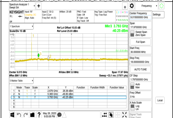
Band41_15MHz_DFT_s_OFDM_SCS30kHz_BPSK_RB1_1_CH536496_below_18G
