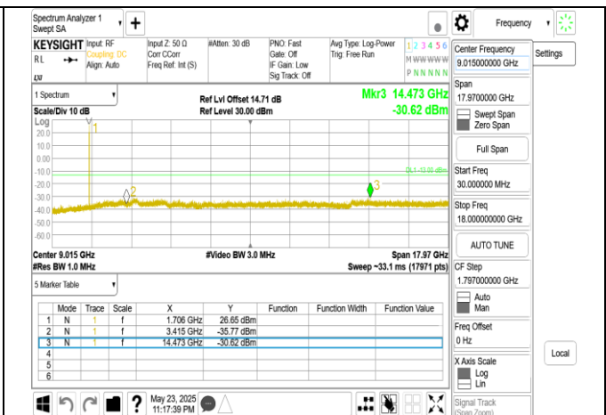
Band70 5MHz DFT s OFDM SCS15kHz BPSK RB1 1 CH341500 below 18G
