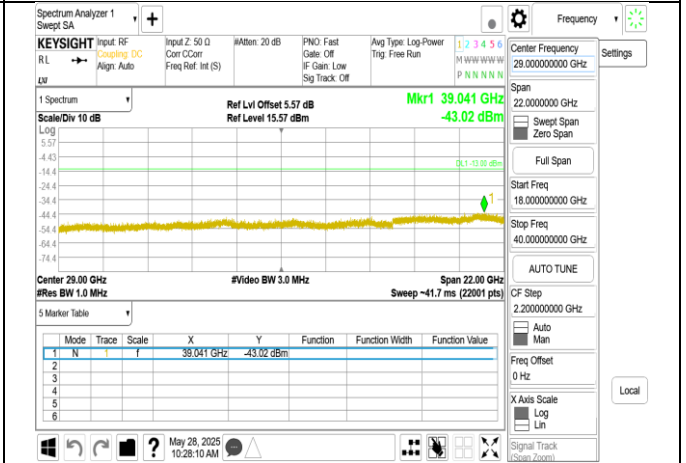
Band77-Part27_10MHz_DFT_s_OFDM_SCS30kHz_BPSK_RB1_1_CH656000_upper 18G
