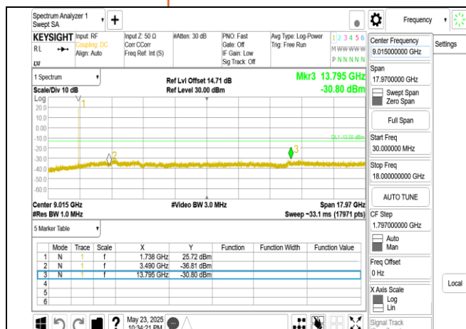
Band66 15MHz DFT s OFDM SCS15kHz BPSK RB1 1 CH349000 below 18G
