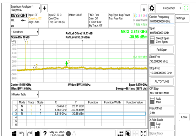
Band71_15MHz_DFT_s_OFDM_SCS15kHz_BPSK_RB1_1_CH136100_below_18G
