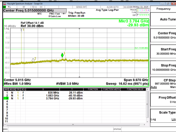
Band26 15MHz DFT s OFDM SCS15kHz BPSK RB1 1 CH168300 below 18G
