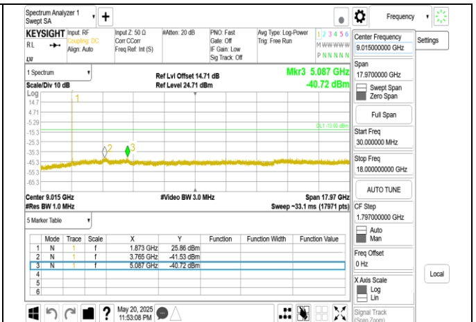
Band25 20MHz DFT s OFDM SCS15kHz BPSK RB1_1 CH376500 below 18G
