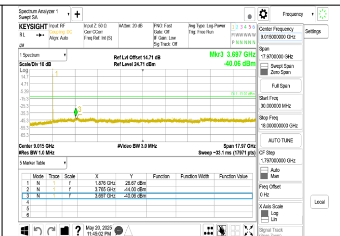
Band25 15MHz DFT s OFDM SCS15kHz BPSK RB1_1 CH376500 below 18G
