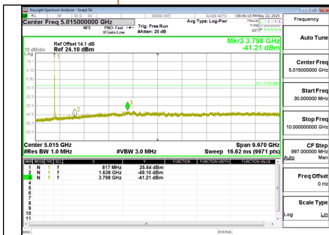
Band26-Part90s_5MHz_DFT_s_OFDM_SCS15kHz_BPSK_RB1_1_CH163800_below 18G
