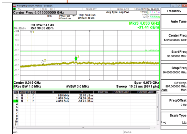
Band26 20MHz DFT s OFDM SCS15kHz BPSK RB1 1 CH166800 below 18G
