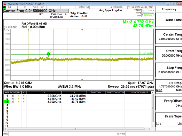
Band30 5MHz DFT s OFDM SCS15kHz BPSK RB1 1 CH461500 below 18G
