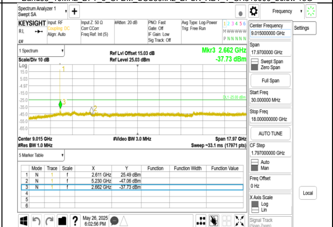
Band38 10MHz DFT s OFDM SCS30kHz BPSK RB1 1 CH523000 below 18G
