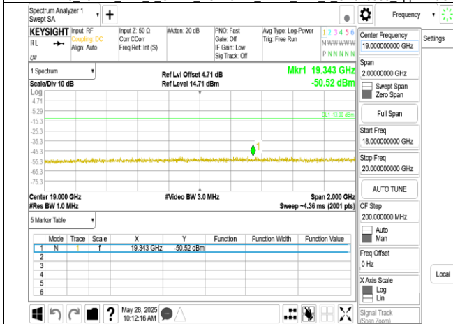
Band25_20MHz_DFT_s_OFDM_SCS15kHz_BPSK_RB1_1_CH381000_upper 18G
