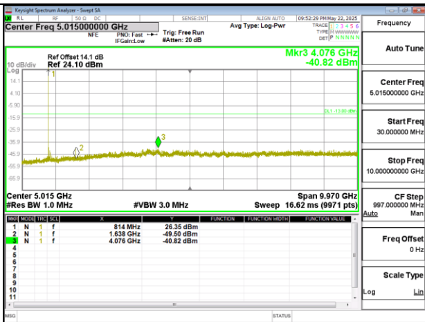
Band26-Part90s_10MHz_DFT_s_OFDM_SCS15kHz_BPSK_RB1_1_CH163800_below 18G
