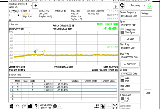
Band41 10MHz DFT s OFDM SCS30kHz BPSK RB1_1 CH500202 below 18G
