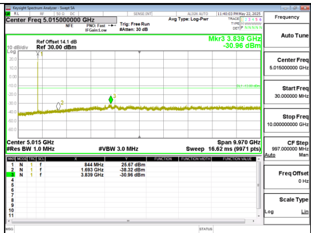
Band26_5MHz_DFT_s_OFDM_SCS15kHz_BPSK_RB1_1_CH169300_below 18G
