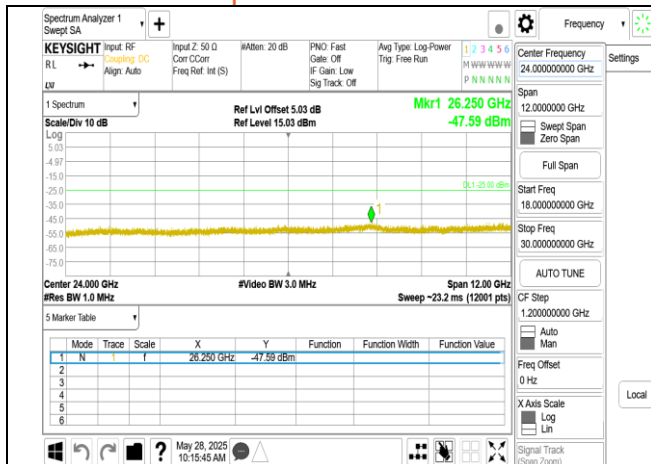
Band38 15MHz DFT s OFDM SCS30kHz BPSK RB1 1 CH515500 upper 18G
