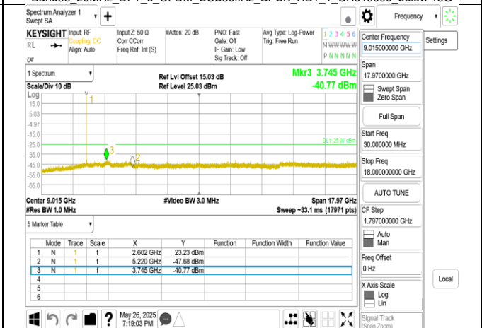
Band38 20MHz DFT s OFDM SCS30kHz BPSK RB1_1 CH522000 below 18G
