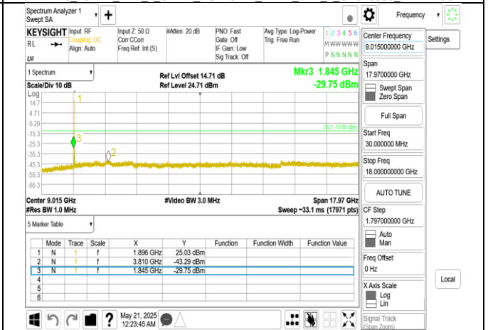
Band25 20MHz DFT s OFDM SCS15kHz BPSK RB1_1 CH381000 below 18G
