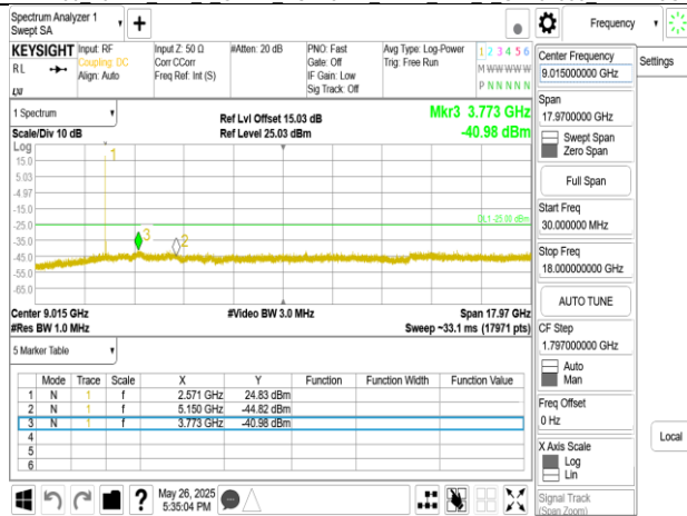
Band38 10MHz DFT s OFDM SCS30kHz BPSK RB1 1 CH515000 below 18G
