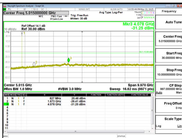
Band26 20MHz DFT s OFDM SCS15kHz BPSK RB1 1 CH167300 below 18G
