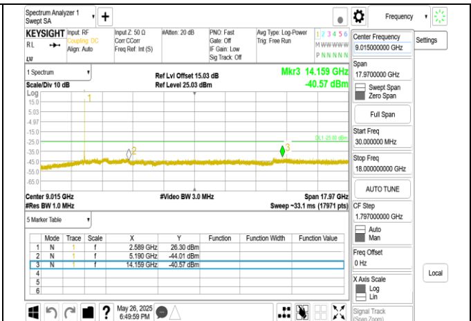
Band38 15MHz DFT s OFDM SCS30kHz BPSK RB1 1 CH519000 below 18G
