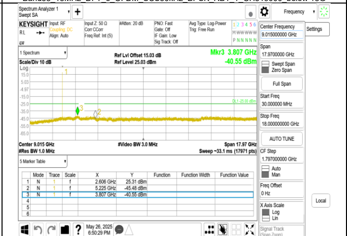
Band38 15MHz DFT s OFDM SCS30kHz BPSK RB1 1 CH522500 below 18G
