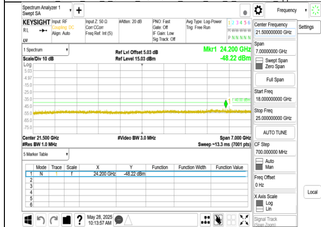
Band30 10MHz DFT s OFDM SCS15kHz BPSK RB1 1 CH462000 upper 18G
