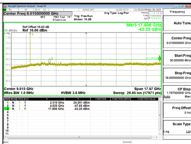
Band30 5MHz DFT s OFDM SCS15kHz BPSK RB1 1 CH462500 below 18G
