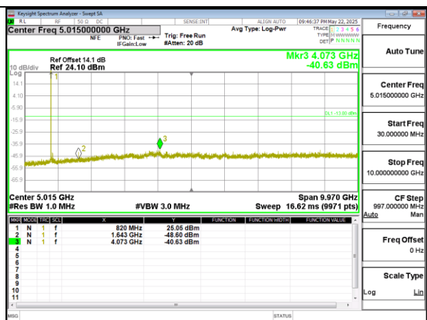
Band26-Part90s_5MHz_DFT_s_OFDM_SCS15kHz_BPSK_RB1_1_CH164300_below 18G
