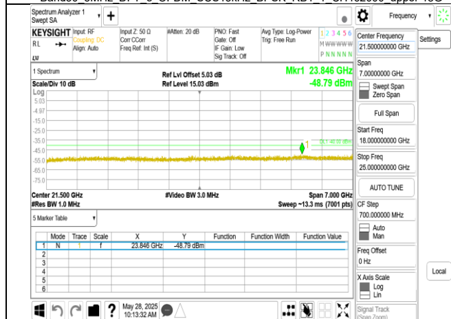
Band30 5MHz DFT s OFDM SCS15kHz BPSK RB1 1 CH462500 upper 18G
