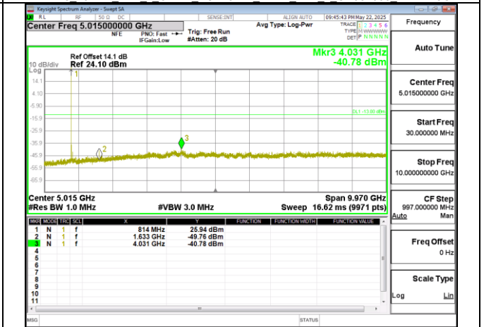
Band26-Part90s_5MHz_DFT_s_OFDM_SCS15kHz_BPSK_RB1_1_CH163300_below 18G
