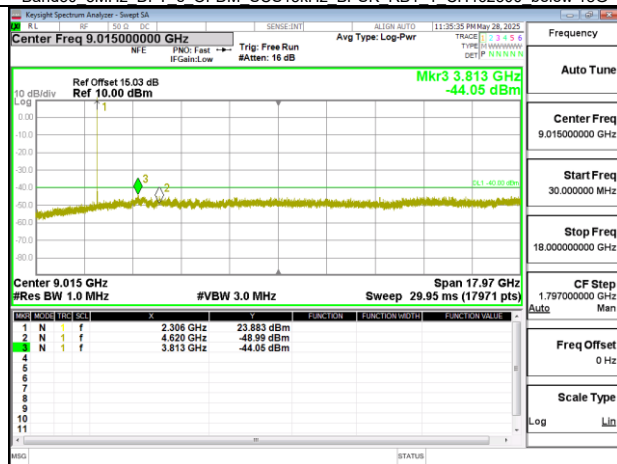
Band30 10MHz DFT s OFDM SCS15kHz BPSK RB1 1 CH462000 below 18G
