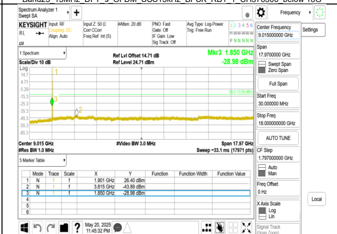
Band25 15MHz DFT s OFDM SCS15kHz BPSK RB1_1 CH381500 below 18G
