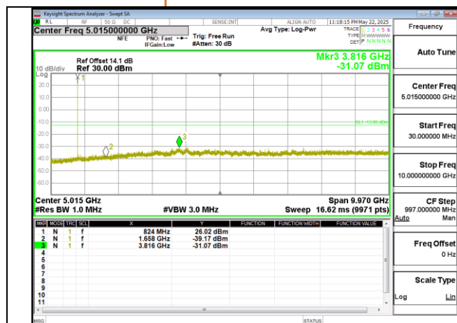
Band26 10MHz DFT s OFDM SCS15kHz BPSK RB1 1 CH165800 below 18G
