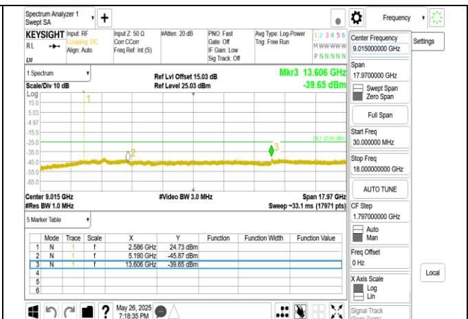
Band38 20MHz DFT s OFDM SCS30kHz BPSK RB1_1 CH519000 below 18G
