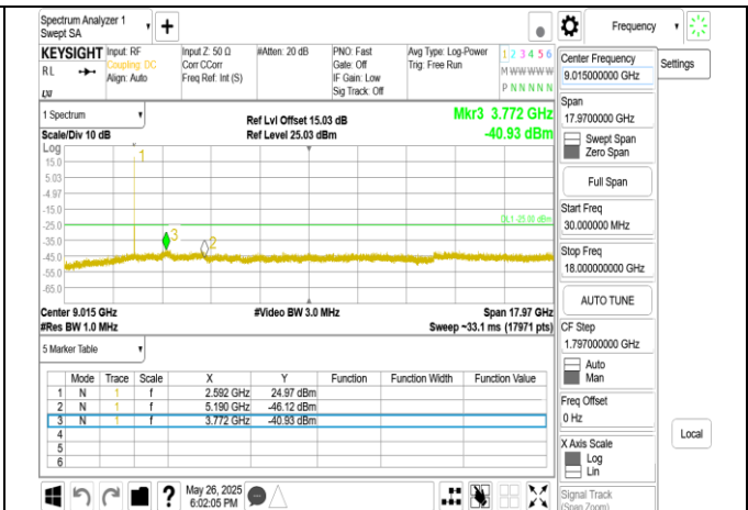
Band38 10MHz DFT s OFDM SCS30kHz BPSK RB1 1 CH519000 below 18G
