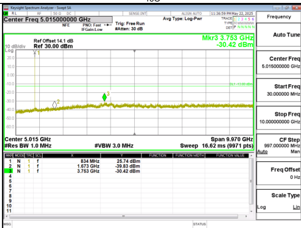
Band26_5MHz_DFT_s_OFDM_SCS15kHz_BPSK_RB1_1_CH167300_below 18G
