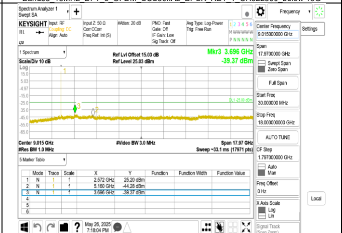
Band38 20MHz DFT s OFDM SCS30kHz BPSK RB1 1 CH516000 below 18G
