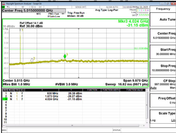
Band26 15MHz DFT s OFDM SCS15kHz BPSK RB1 1 CH167300 below 18G
