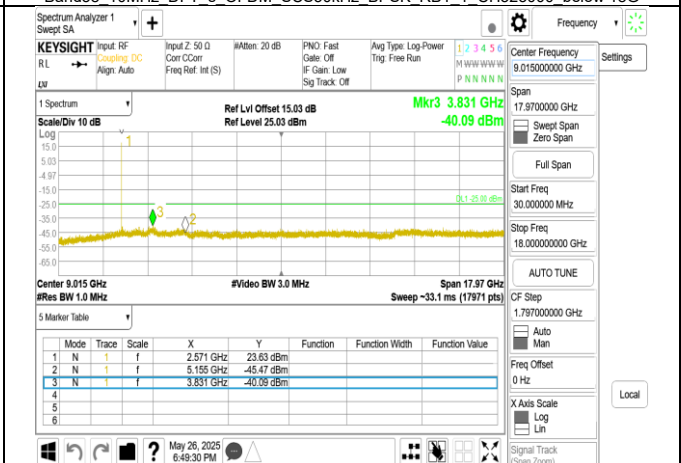
Band38 15MHz DFT s OFDM SCS30kHz BPSK RB1 1 CH515500 below 18G
