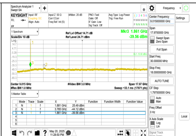
Band25 5MHz DFT s OFDM SCS15kHz BPSK RB1 1 CH376500 below 18G
