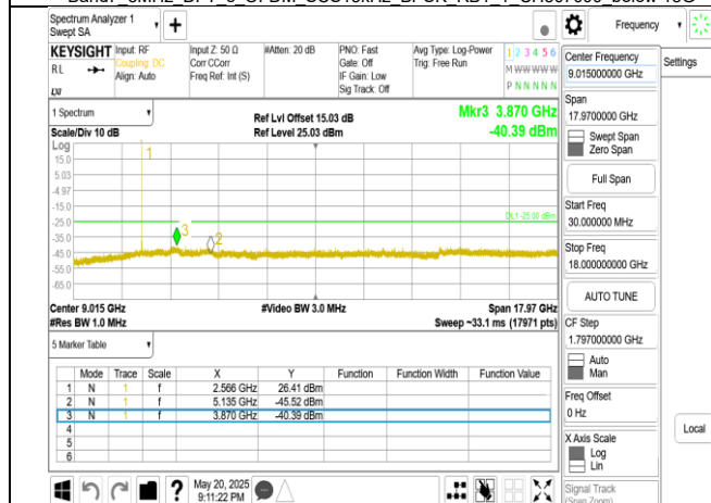
Band7_5MHz_DFT_s_OFDM_SCS15kHz_BPSK_RB1_1_CH513500_below_18G
