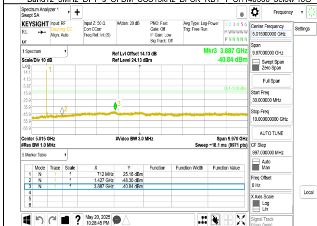
Band12_5MHz_DFT s OFDM_SCS15kHz_BPSK_RB1_1_CH142700 below 18G
