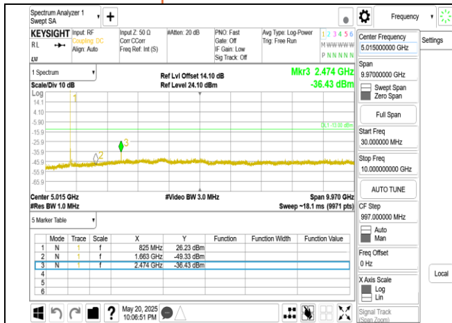
Band5 15MHz DFT s OFDM SCS15kHz BPSK RB1 1 CH166300 below 18G
