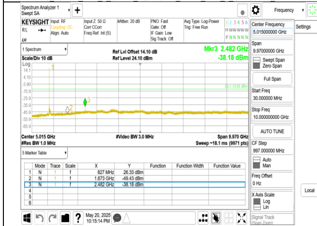
Band5 20MHz DFT s OFDM SCS15kHz BPSK RB1 1 CH167300 below 18G
