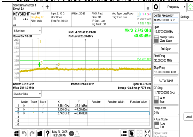
Band7 10MHz DFT s OFDM SCS15kHz BPSK RB1 1 CH513000 below 18G
