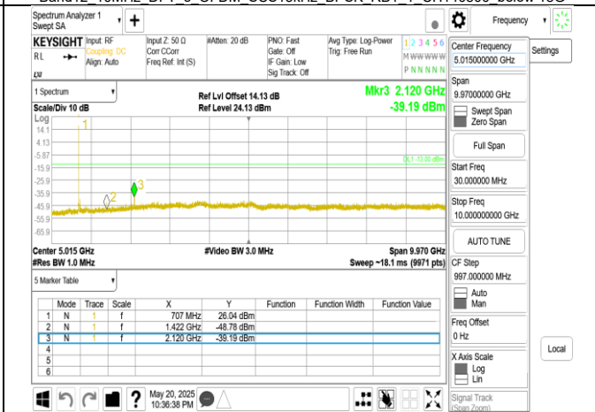
Band12_10MHz_DFT s OFDM_SCS15kHz_BPSK_RB1_1_CH142200 below 18G
