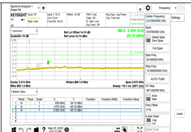
Band5 5MHz DFT s OFDM SCS15kHz BPSK RB1 1 CH167300 below 18G
