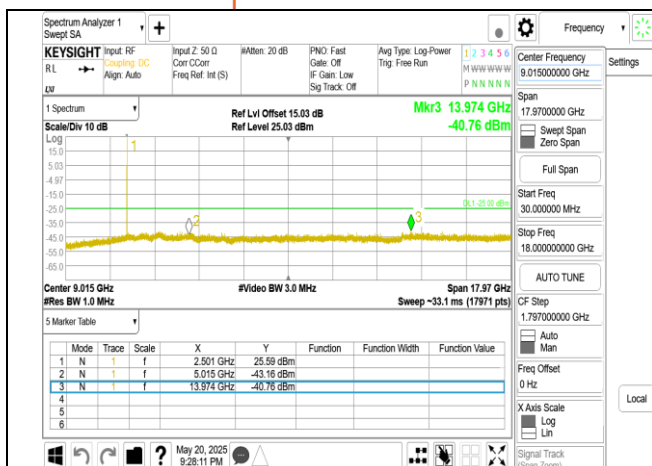
Band7 15MHz DFT s OFDM SCS15kHz BPSK RB1 1 CH501500 below 18G
