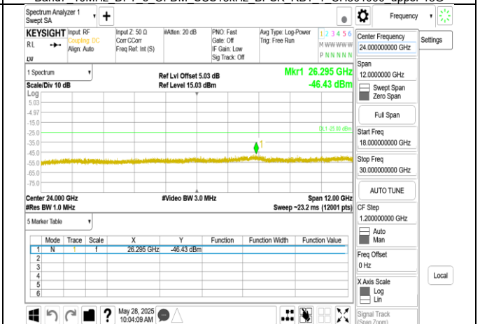
Band7 10MHz DFT s OFDM SCS15kHz BPSK RB1 1 CH507000 upper 18G
