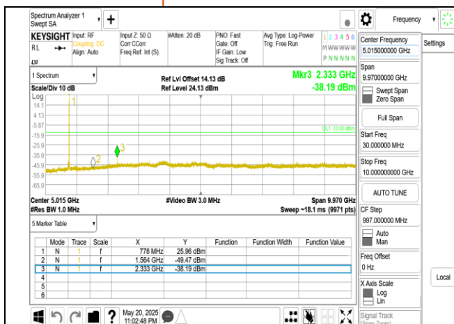
Band13 10MHz DFT s OFDM SCS15kHz BPSK RB1 1 CH156400 below 18G
