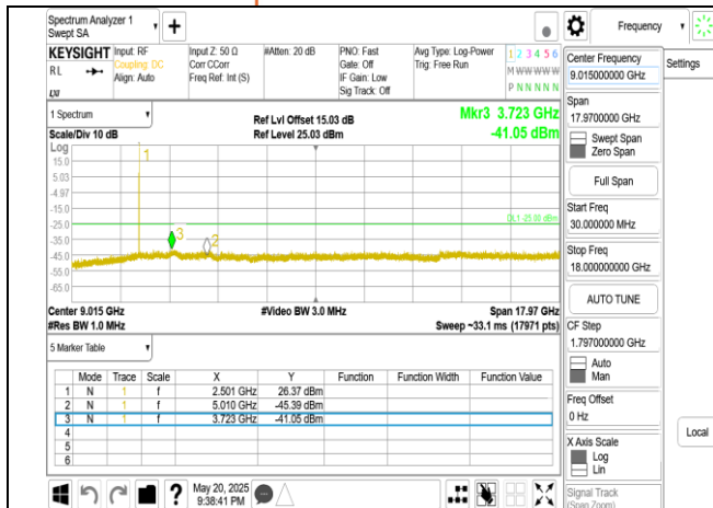
Band7 10MHz DFT s OFDM SCS15kHz BPSK RB1 1 CH501000 below 18G
