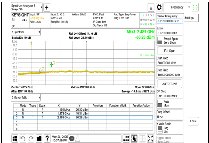
Band5 15MHz DFT s OFDM SCS15kHz BPSK RB1 1 CH167300 below 18G
