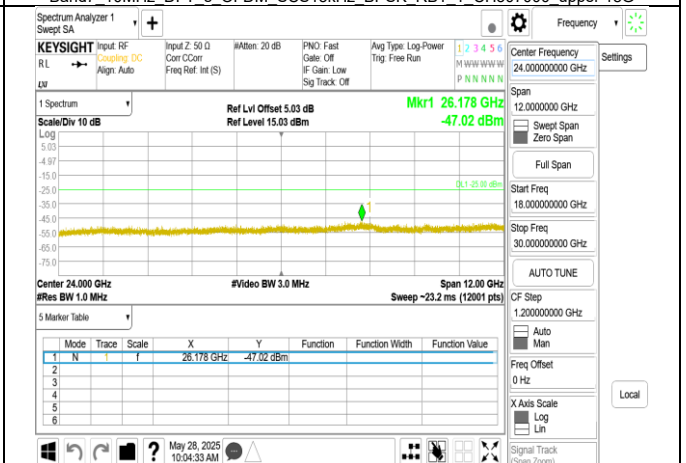
Band7 10MHz DFT s OFDM SCS15kHz BPSK RB1 1 CH513000 upper 18G
