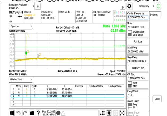
Band25 5MHz DFT s OFDM SCS15kHz BPSK RB1 1 CH382500 below 18G
