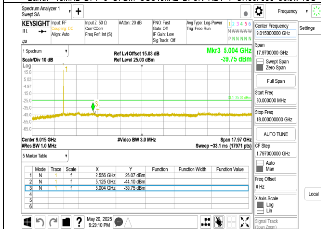
Band7 15MHz DFT s OFDM SCS15kHz BPSK RB1 1 CH512500 below 18G
