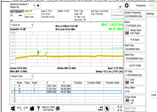
Band7_20MHz_DFT_s_OFDM_SCS15kHz_BPSK_RB1_1_CH512000_below_18G
