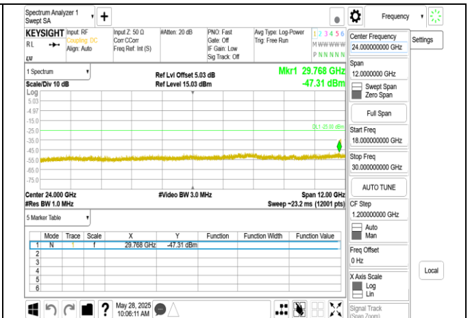
Band7_20MHz_DFT_s_OFDM_SCS15kHz_BPSK_RB1_1_CH502000_upper_18G
