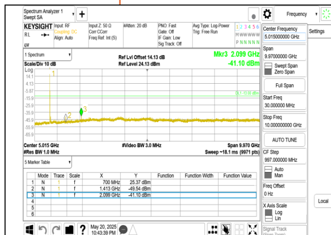
Band12_15MHz_DFT s OFDM SCS15kHz_BPSK RB1_1_CH141300 below 18G
