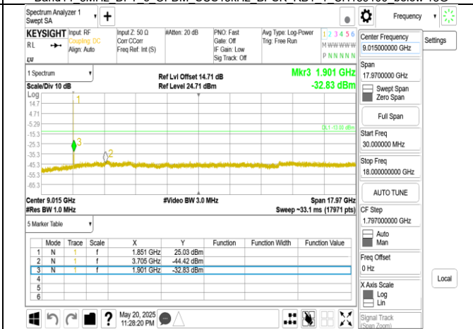
Band25 5MHz DFT s OFDM SCS15kHz BPSK RB1 1 CH370500 below 18G
