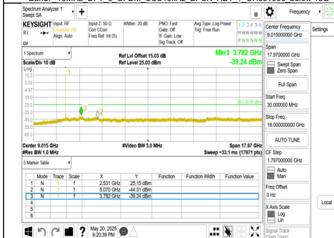
Band7 10MHz DFT s OFDM SCS15kHz BPSK RB1 1 CH507000 below 18G
