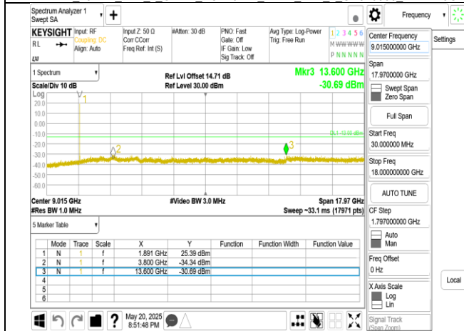
Band2 20MHz DFT s OFDM SCS15kHz BPSK RB1 1 CH380000 below 18G
