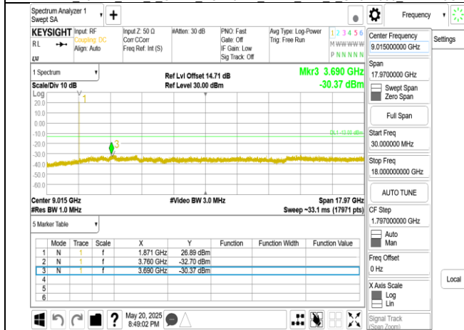
Band2 20MHz DFT s OFDM SCS15kHz BPSK RB1 1 CH376000 below 18G
