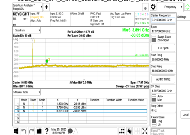
Band2_5MHz_DFT_s_OFDM_SCS15kHz_BPSK_RB1_1_CH376000 below 18G
