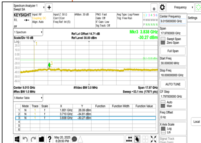
Band2 10MHz DFT s OFDM SCS15kHz BPSK RB1 1 CH371000 below 18G
