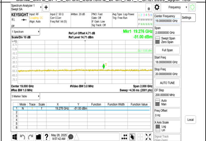
Band2_5MHz_DFT_s_OFDM_SCS15kHz_BPSK_RB1_1_CH381500 upper 18G
