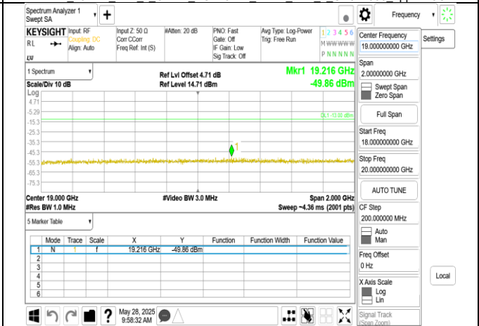
Band2 10MHz DFT s OFDM SCS15kHz BPSK RB1 1 CH376000 upper 18G
