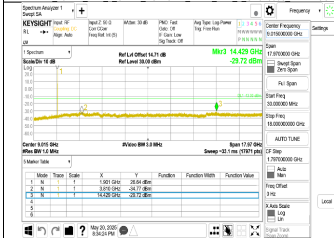
Band2 10MHz DFT s OFDM SCS15kHz BPSK RB1 1 CH381000 below 18G
