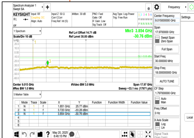
Band2 20MHz DFT s OFDM SCS15kHz BPSK RB1 1 CH372000 below 18G
