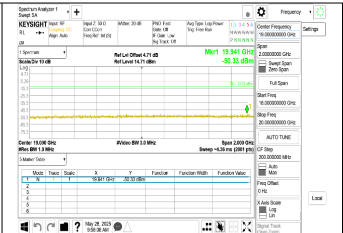
Band2 10MHz DFT s OFDM SCS15kHz BPSK RB1 1 CH371000 upper 18G
