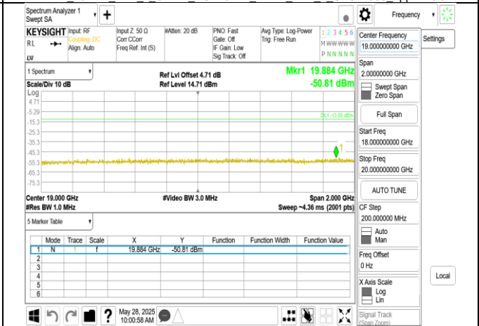
Band2 20MHz DFT s OFDM SCS15kHz BPSK RB1 1 CH376000 upper 18G
