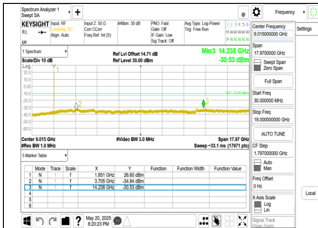
Band2_5MHz_DFT_s_OFDM_SCS15kHz_BPSK_RB1_1_CH370500 below 18G
