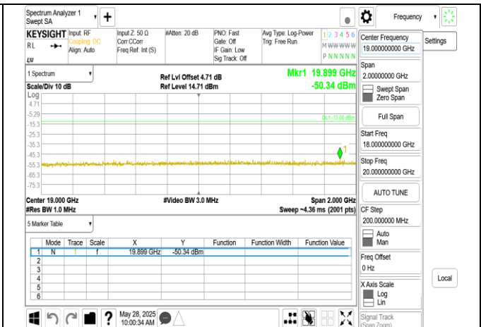
Band2 20MHz DFT s OFDM SCS15kHz BPSK RB1 1 CH372000 upper 18G
