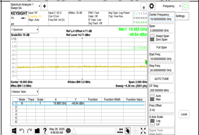
Band2 10MHz DFT s OFDM SCS15kHz BPSK RB1 1 CH381000 upper 18G
