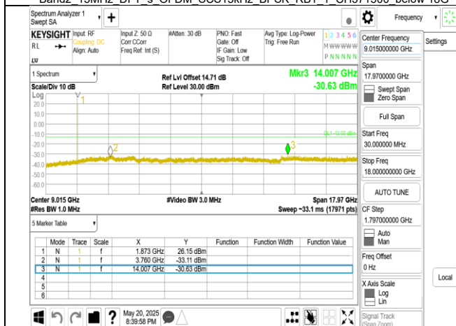
Band2 15MHz DFT s OFDM SCS15kHz BPSK RB1 1 CH376000 below 18G
