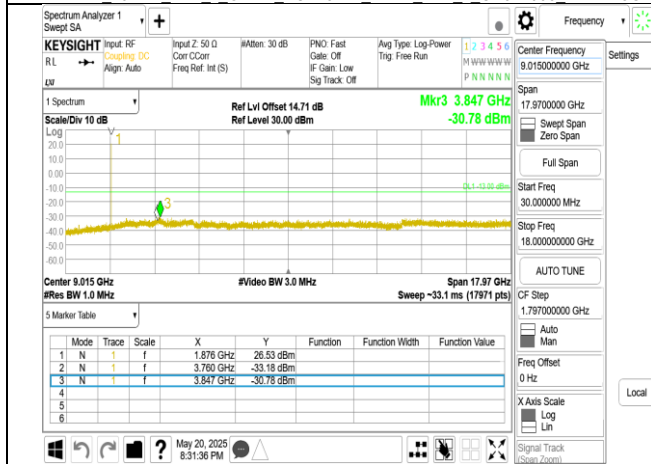
Band2 10MHz DFT s OFDM SCS15kHz BPSK RB1 1 CH376000 below 18G
