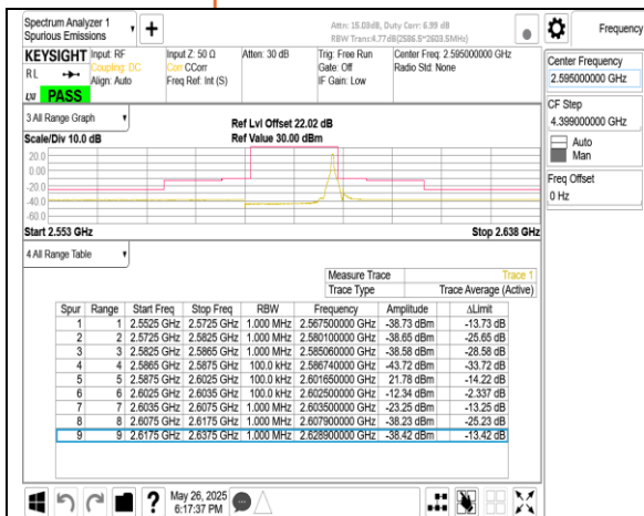
Band38 15MHz DFT s OFDM SCS30kHz BPSK RB1 37 CH519000
