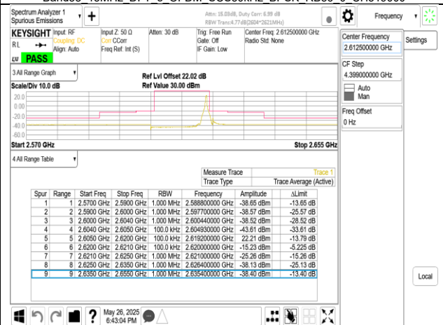
Band38 15MHz DFT s OFDM SCS30kHz BPSK RB1 37 CH522500
