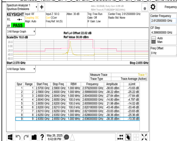
Band38 15MHz DFT s OFDM SCS30kHz BPSK RB1 0 CH522500
