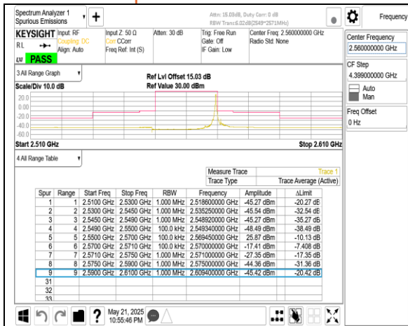
Band7 20MHz DFT s OFDM SCS15kHz BPSK RB1 105 CH512000
