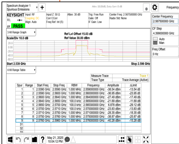
Band7 5MHz DFT s OFDM SCS15kHz BPSK RB25 0 CH513500
