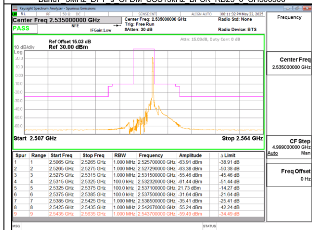
Band7 5MHz DFT s OFDM SCS15kHz BPSK RB1 24 CH507000
