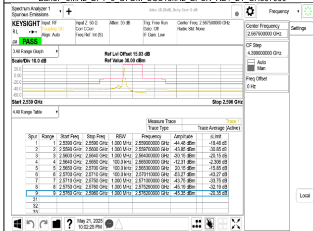
Band7 5MHz DFT s OFDM SCS15kHz BPSK RB1 0 CH513500
