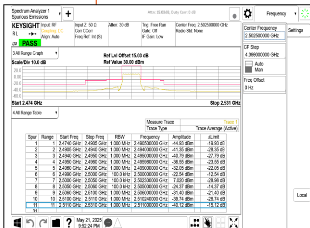
Band7 5MHz DFT s OFDM SCS15kHz BPSK RB25 0 CH500500
