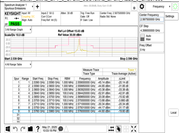
Band7 5MHz DFT s OFDM SCS15kHz BPSK RB1 24 CH513500
