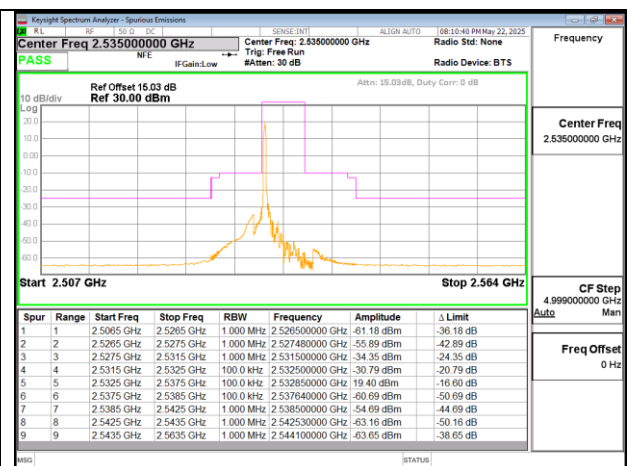
Band7 5MHz DFT s OFDM SCS15kHz BPSK RB1 0 CH507000
