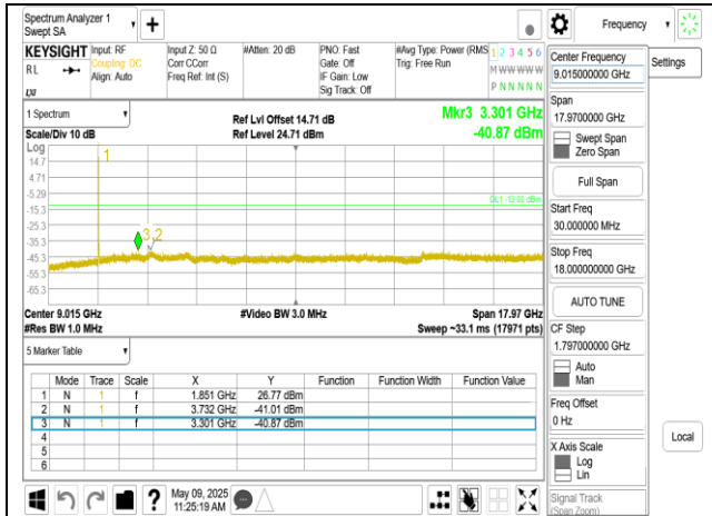
Band2_15MHz_QPSK_RB1_0_CH18675_below_18G
