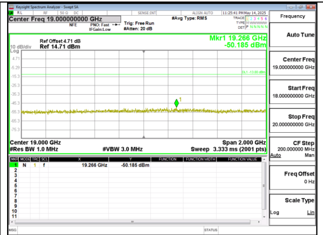
Band2_15MHz_QPSK_RB1_0_CH18675_upper_18G
