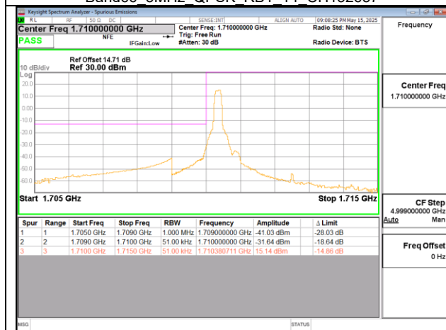
Band66 5MHz QPSK RB1 0 CH131997
