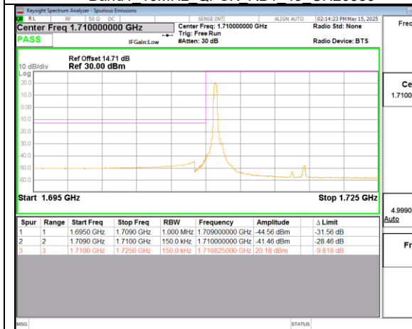
Band4 15MHz QPSK RB1 0 CH20025
