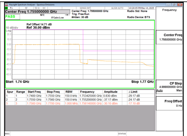
Band4 15MHz QPSK RB75 0 CH20325
