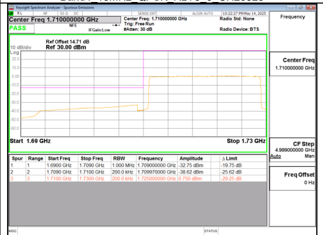
Band4 20MHz QPSK RB100 0 CH20050
