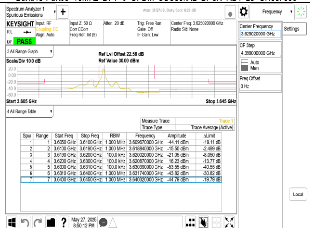
Band48-Part96 10MHz DFT s OFDM SCS30kHz BPSK RB1 0 CH641668
