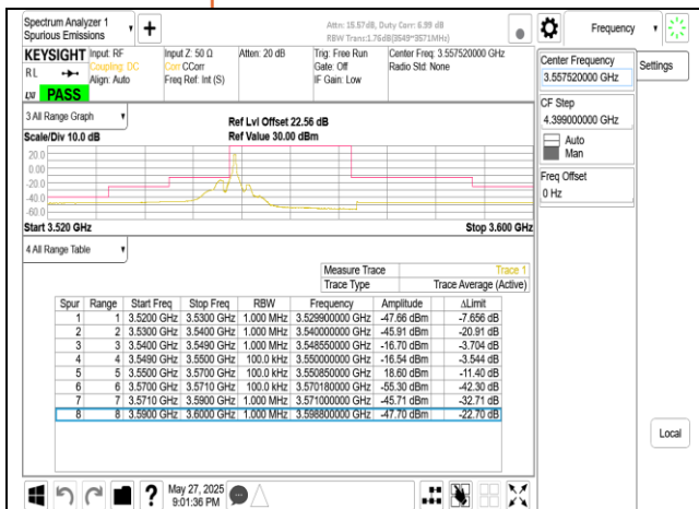
Band48-Part96 15MHz DFT s OFDM SCS30kHz BPSK RB1_0 CH637168
