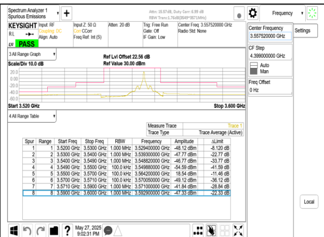
Band48-Part96 15MHz DFT s OFDM SCS30kHz BPSK RB1_37 CH637168
