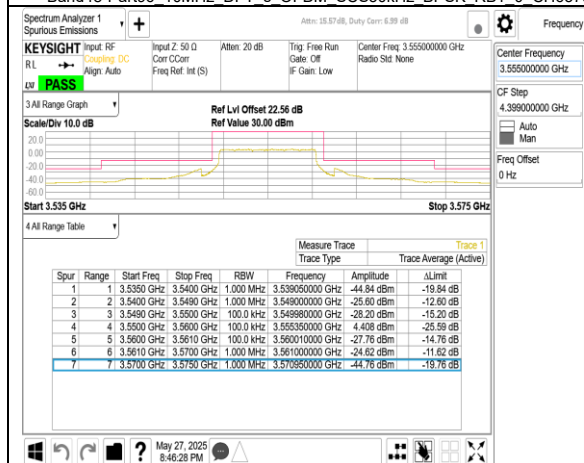
Band48-Part96 10MHz DFT s OFDM SCS30kHz BPSK RB24 0 CH637000
