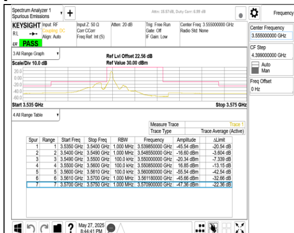
Band48-Part96 10MHz DFT s OFDM SCS30kHz BPSK RB1 0 CH637000
