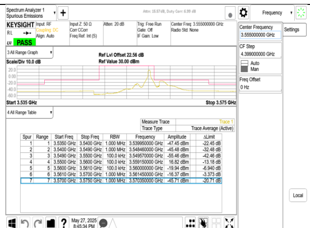
Band48-Part96 10MHz DFT s OFDM SCS30kHz BPSK RB1 23 CH637000
