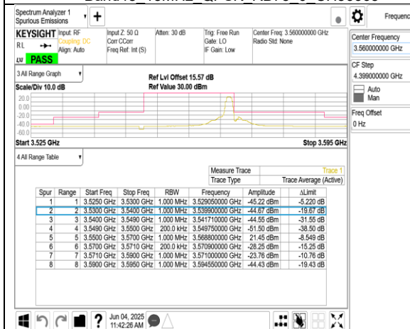
Band48 20MHz QPSK RB1 99 CH55340
