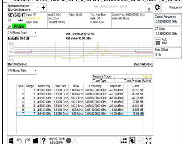
Band48-Part96 10MHz DFT s OFDM SCS30kHz BPSK RB1 23 CH641668
