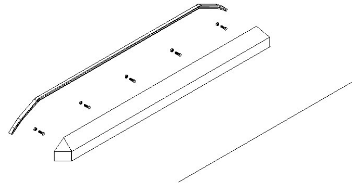
211480 FENDER KIT 211439 FENDER WELDMENT 211481 EDGE TRIM
