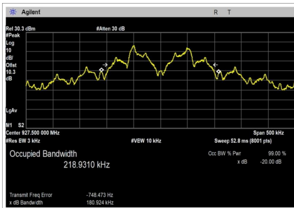
Rate6-06-PWR31-Radio2-High Channel
