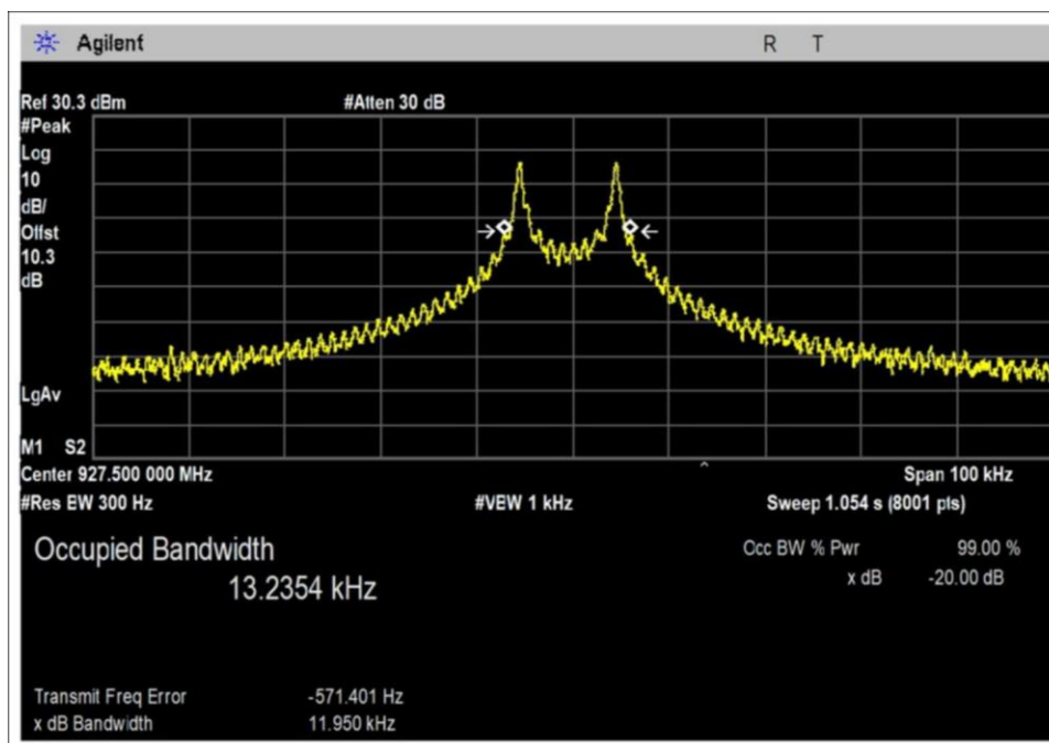
Rate0-06-PWR31-Radio2-High Channel
