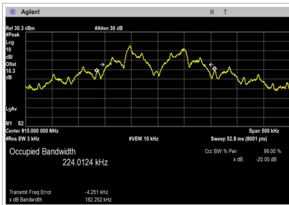
Rate6-02-PWR31-Radio1-Middle Channel
