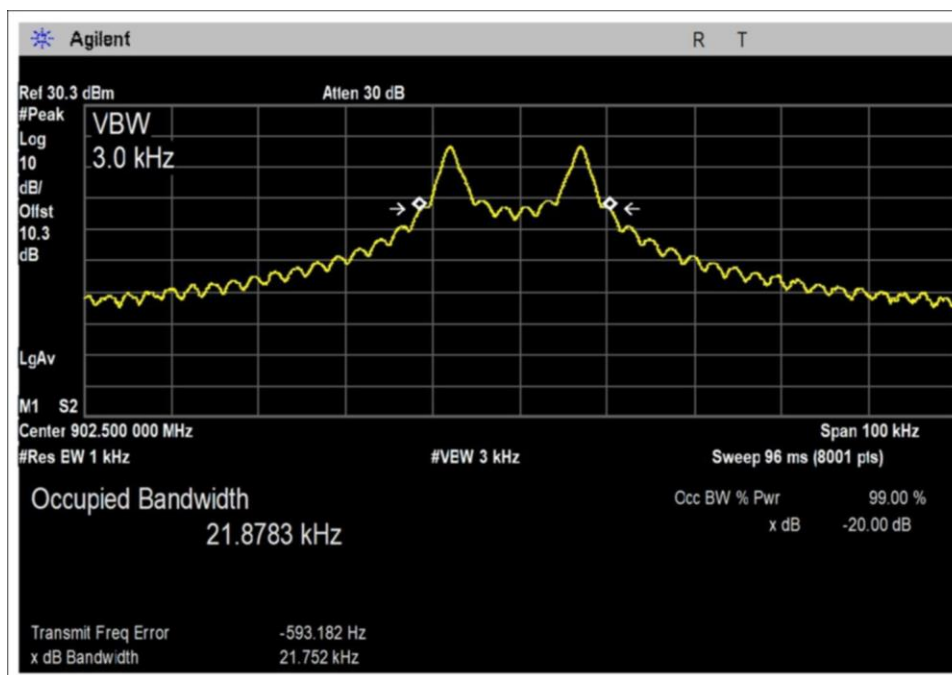
Rate1-04-PWR31-Radio2-Low Channel
