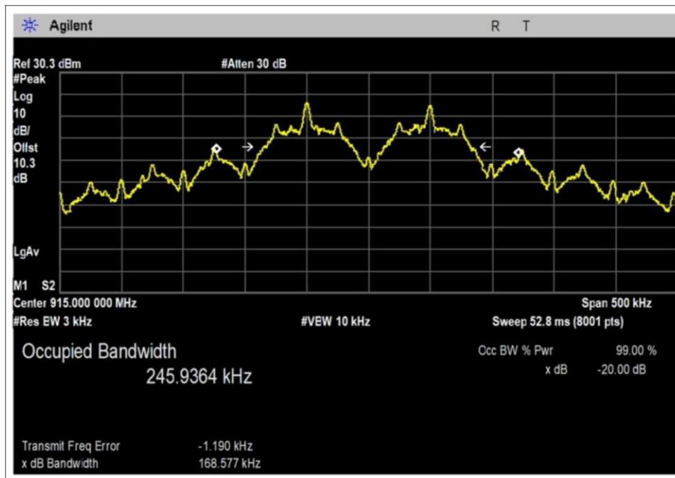
Rate5-05-PWR31-Radio2-Middle Channel
