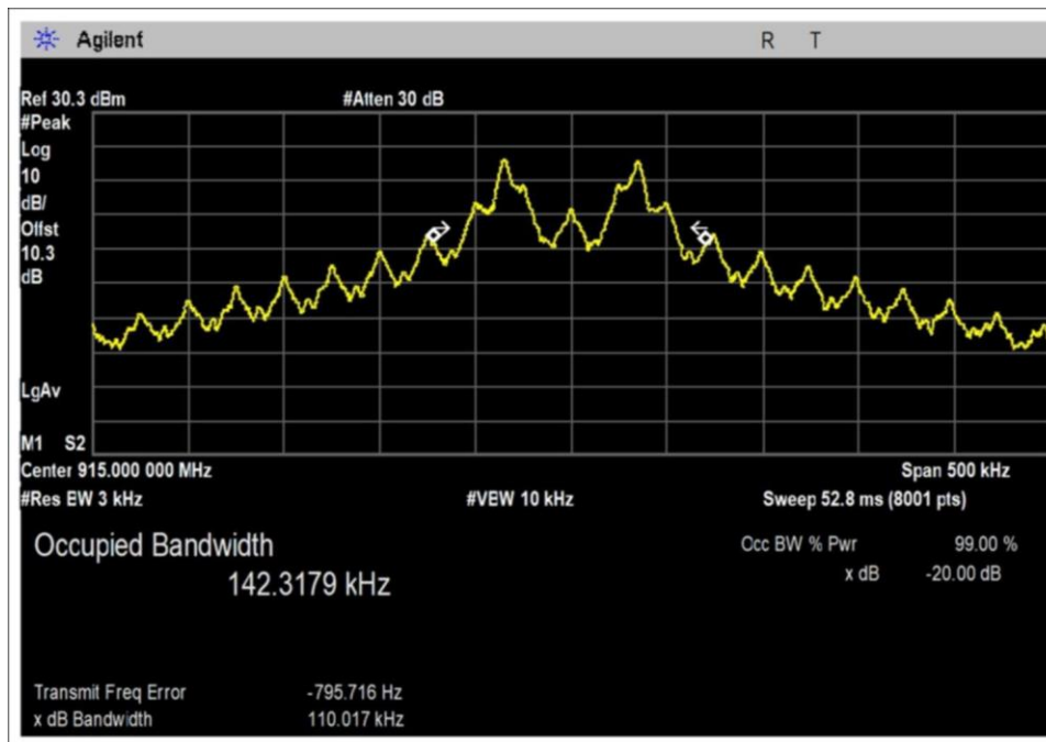
Rate4-05-PWR31-Radio2-Middle Channel
