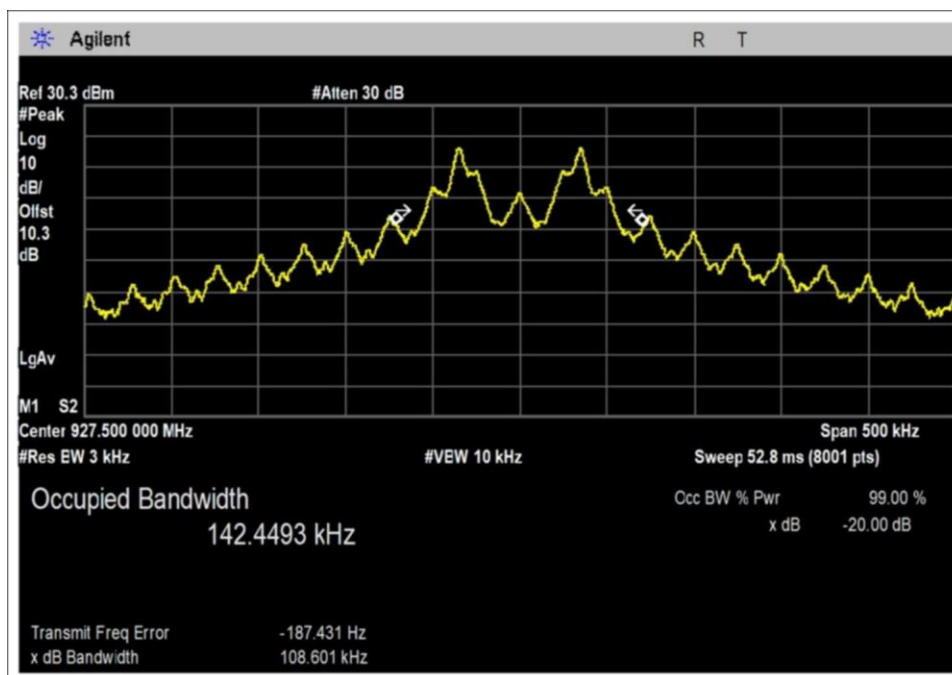
Rate4-06-PWR31-Radio2-High Channel
