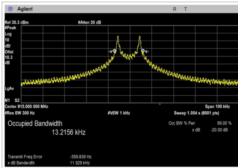
Rate0-05-PWR31-Radio2-Middle Channel
