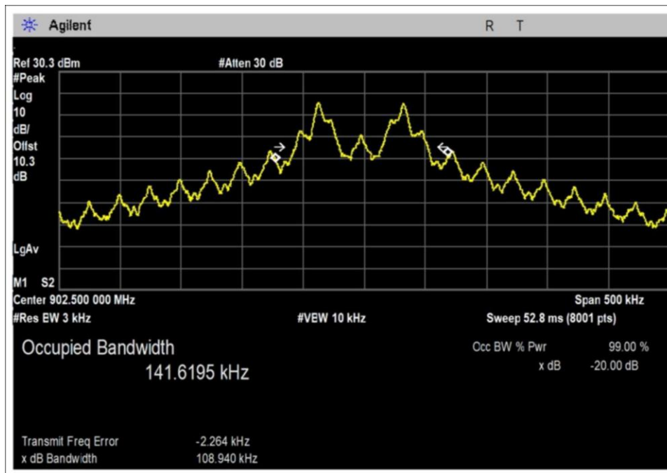
Rate4-01-PWR31-Radio1-Low Channel
