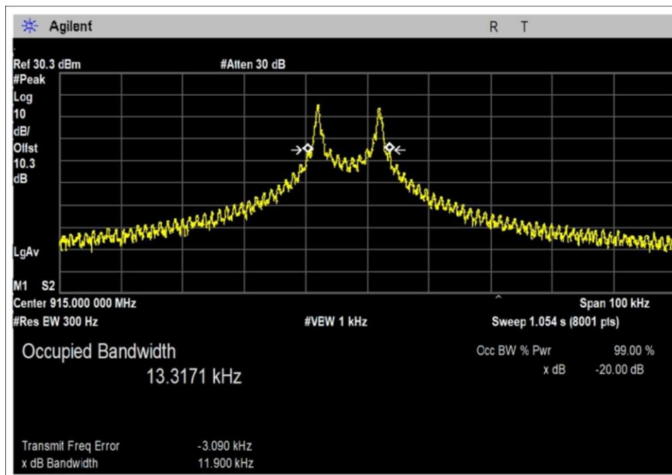
Rate0-02-PWR31-Radio1-Middle Channel
