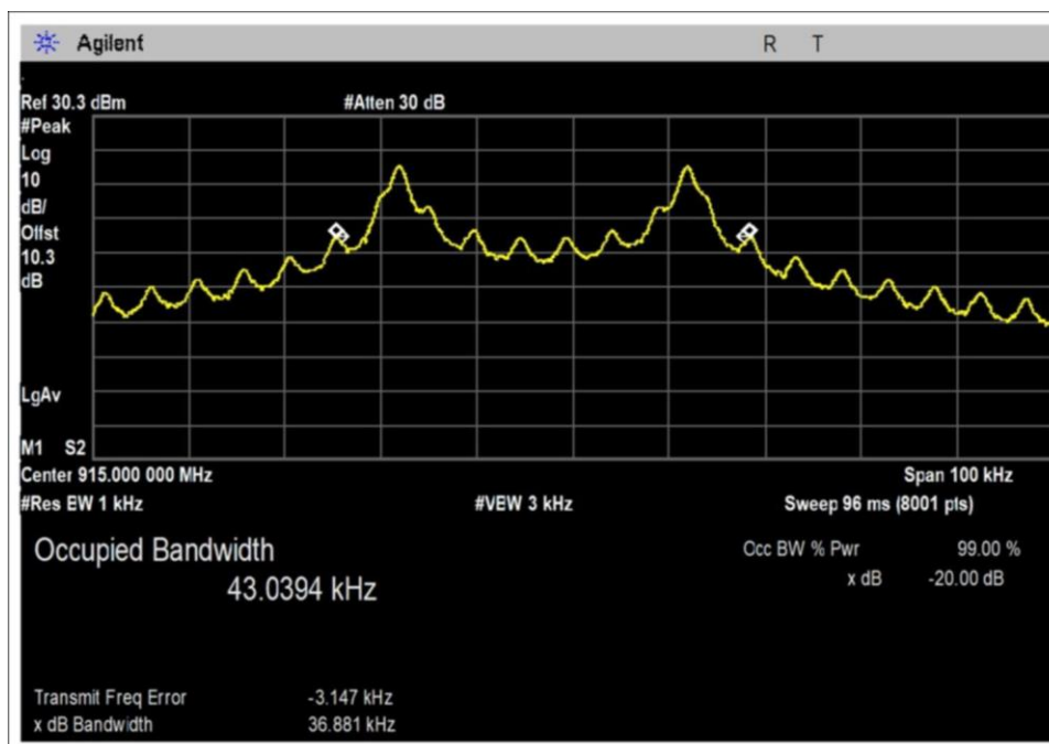
Rate2-02-PWR31-Radio1-Middle Channel
