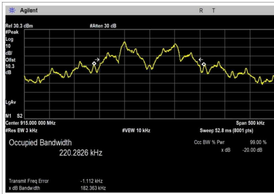
Rate6-05-PWR31-Radio2-Middle Channel
