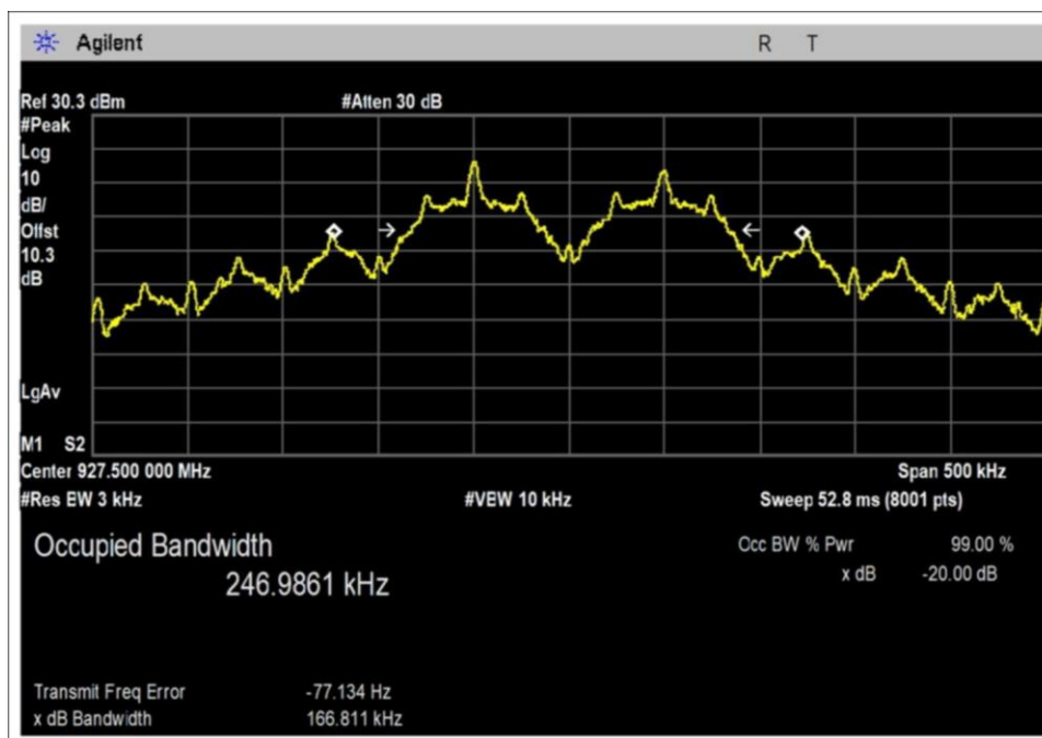
Rate5-06-PWR31-Radio2-High Channel
