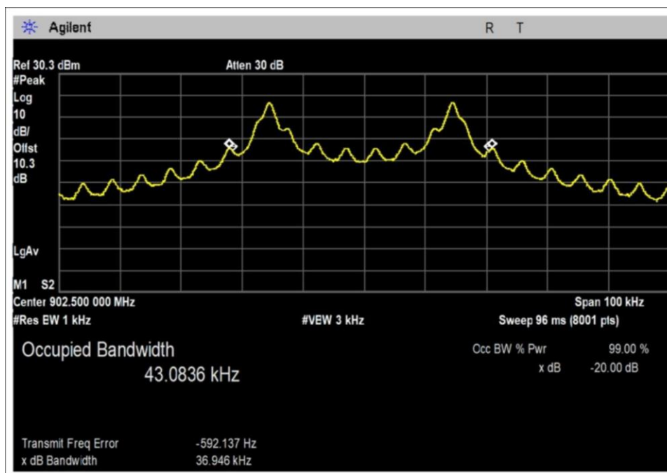
Rate2-04-PWR31-Radio2-Low Channel
