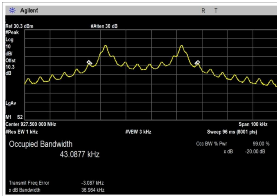
Rate2-03-PWR31-Radio1-High Channel
