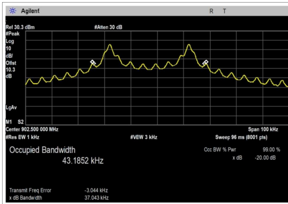
Rate2-01-PWR31-Radio1-Low Channel
