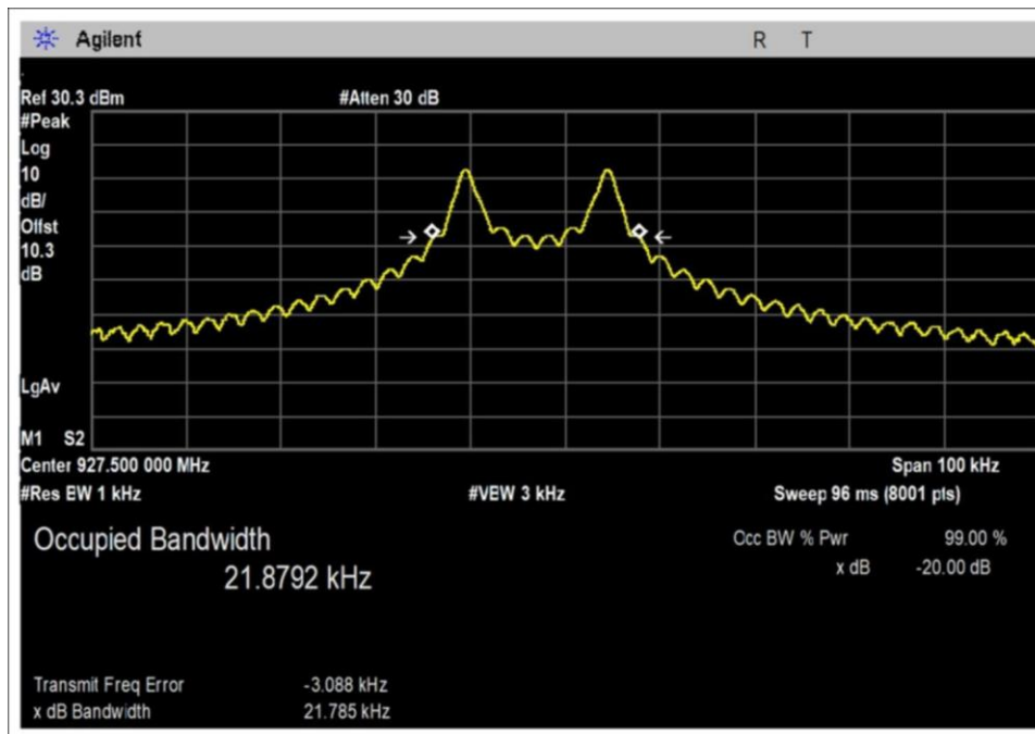
Rate1-03-PWR31-Radio1-High Channel
