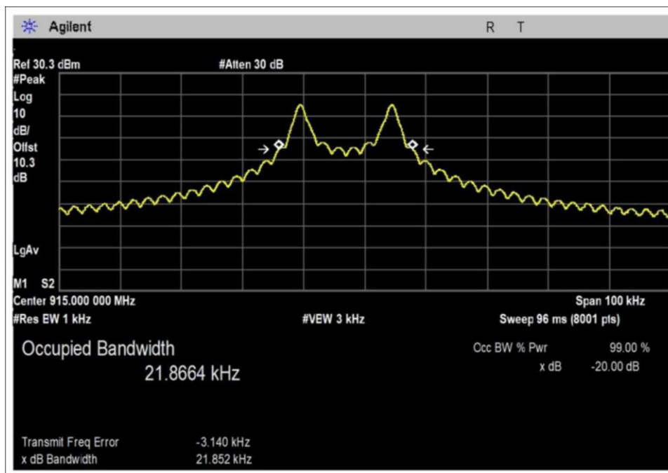
Rate1-05-PWR31-Radio2-Middle Channel
