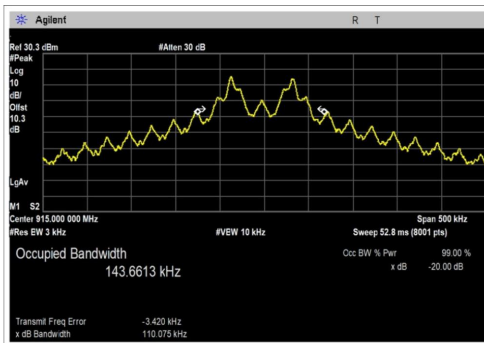
Rate4-02-PWR31-Radio1-Middle Channel
