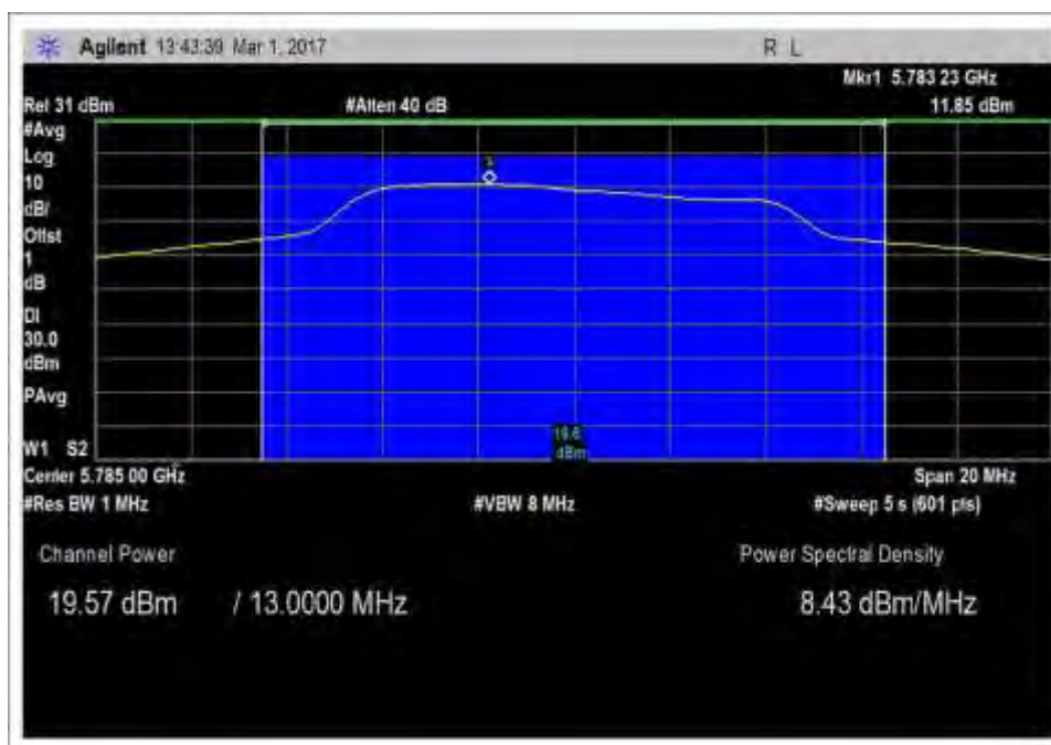
Power_TX24dBm_5785MHz_chain 1_RMS
