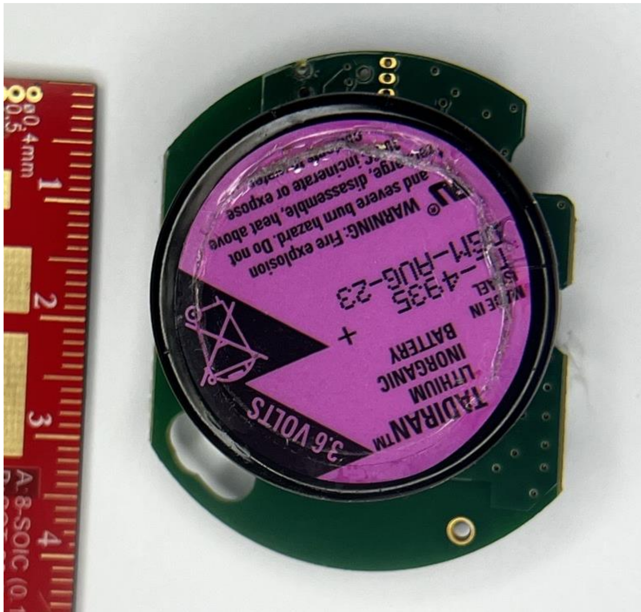
Figure 3: PCB Assembly Bottom View with intergtated battery
