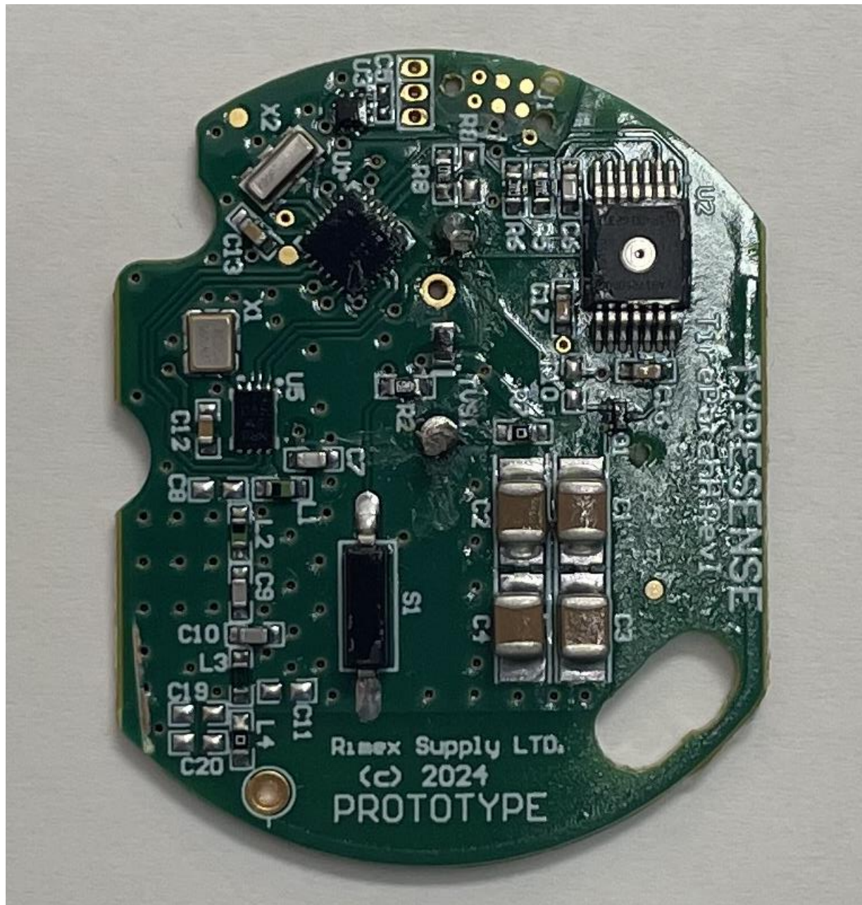
Figure 1: PCB Assembly Top View
