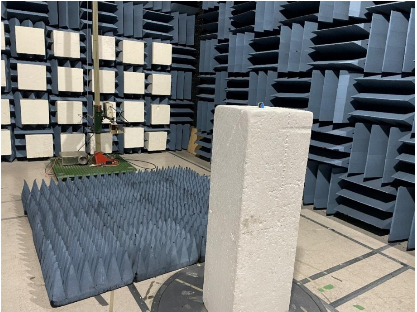
Figure 2: Radiated Emissions (Above 1GHz) Test Setup
