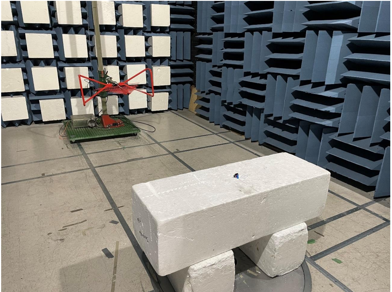
Figure 1: Radiated Emissions (Below 1GHz) Test Setup
