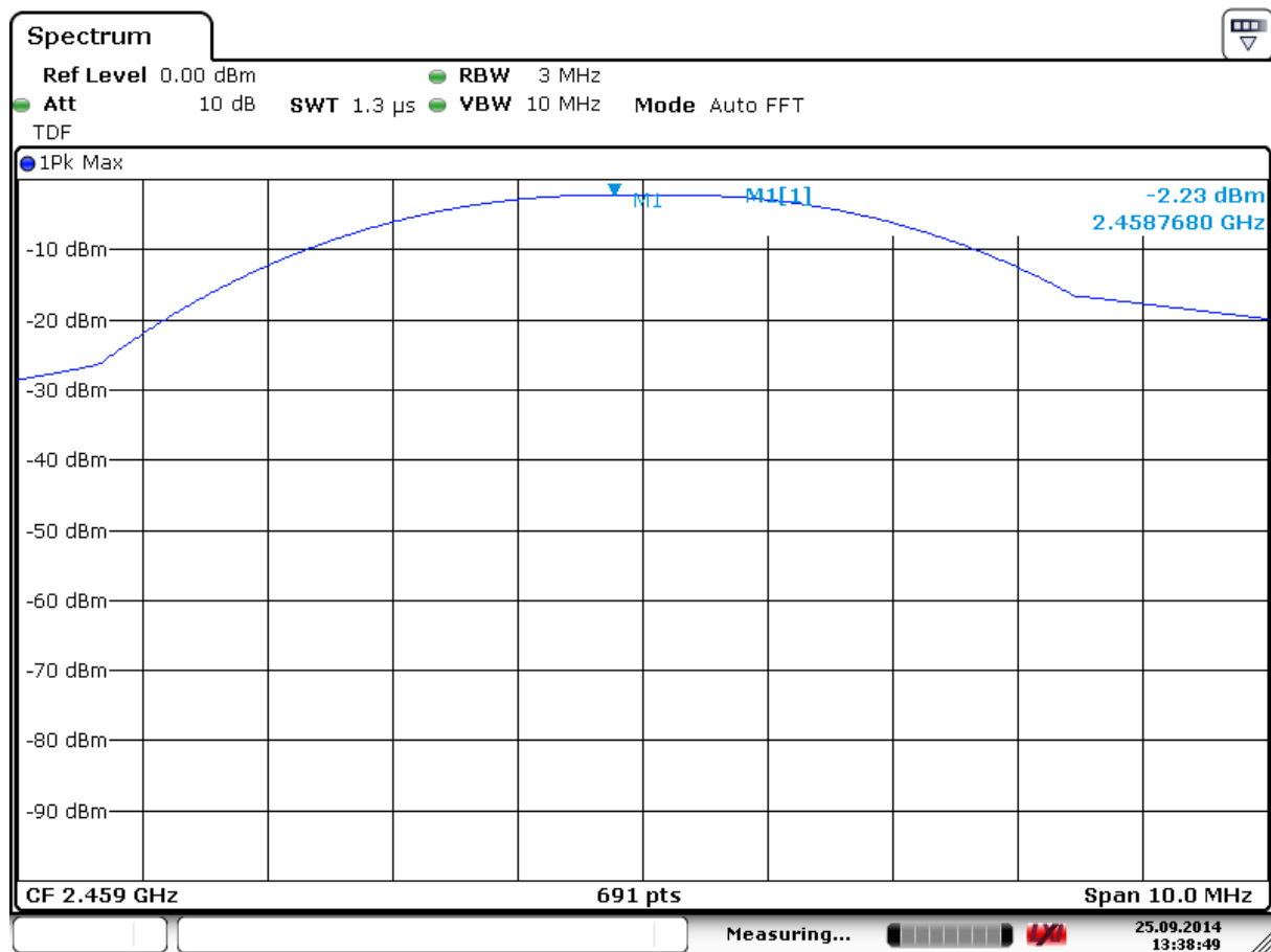
Plot 3: Peak Output Power (2459 MHz)
