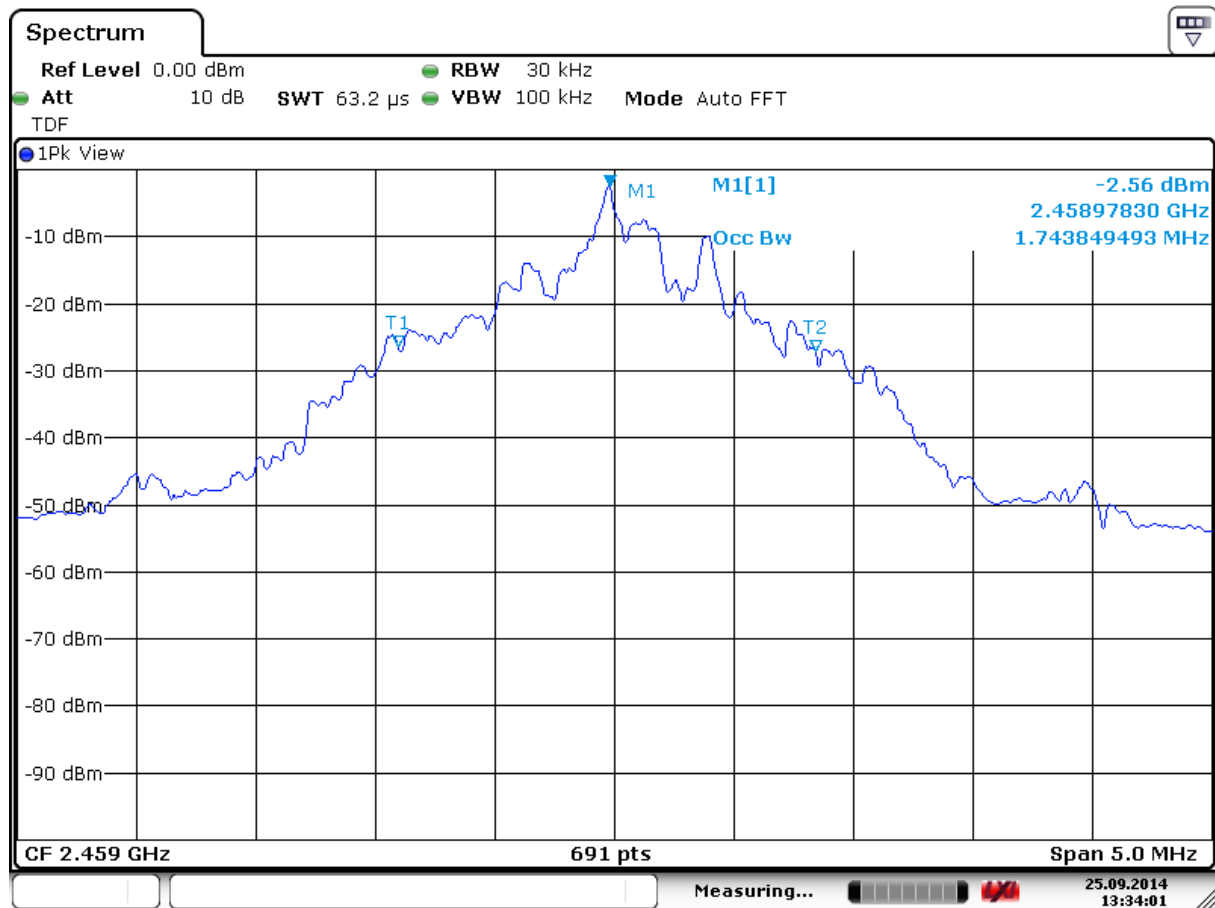
Plot 6: Emission 20dB Bandwidth (= 1.74 MHz) of the EUT transmitting at 2459 MHz
