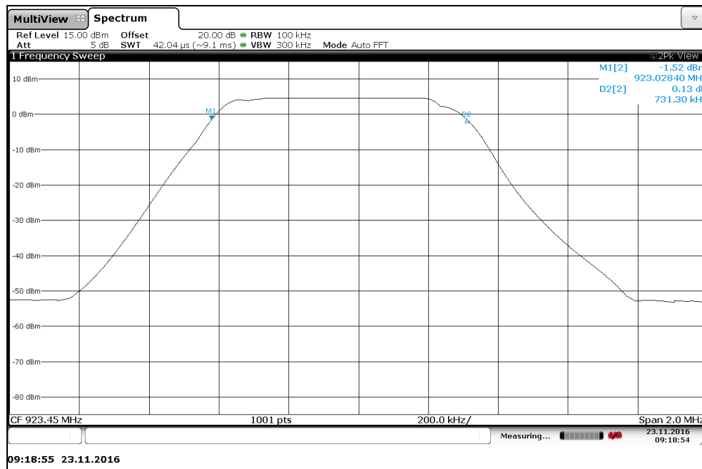
Figure 7.4.2-1: 6dB Bandwidth
