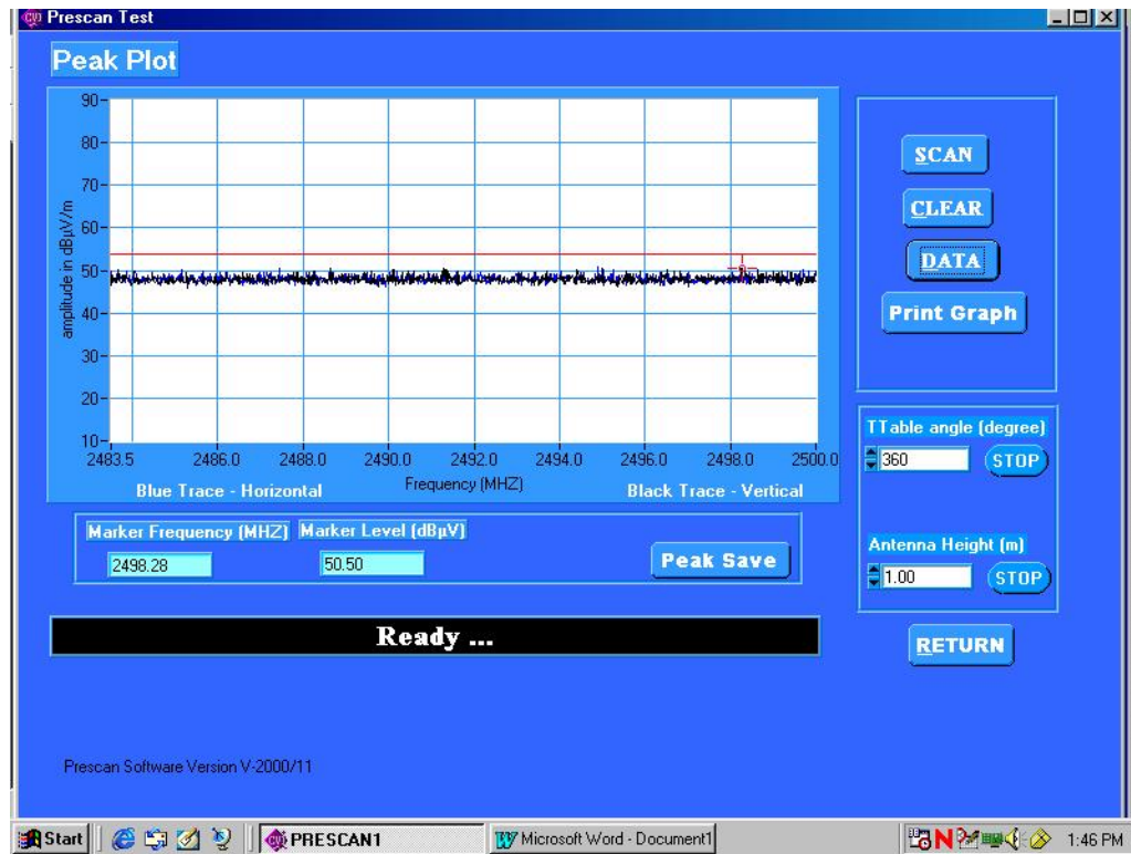
Channel 13 @ 1Mbps
