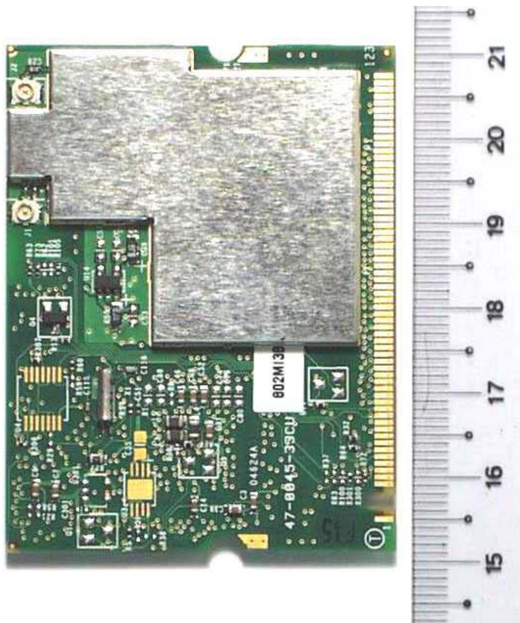
EUT PCB3 – View 2
