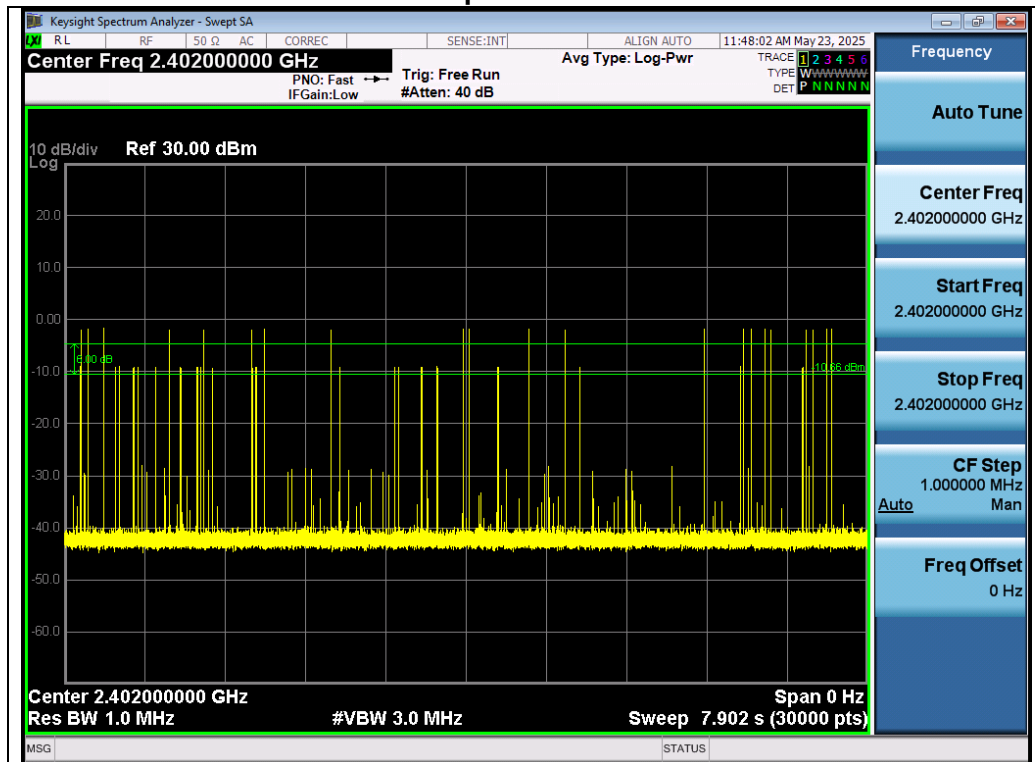
Test_Graph_EDR_HOP_ANT1_NA_3Mbps_2402_Number of Burstr
