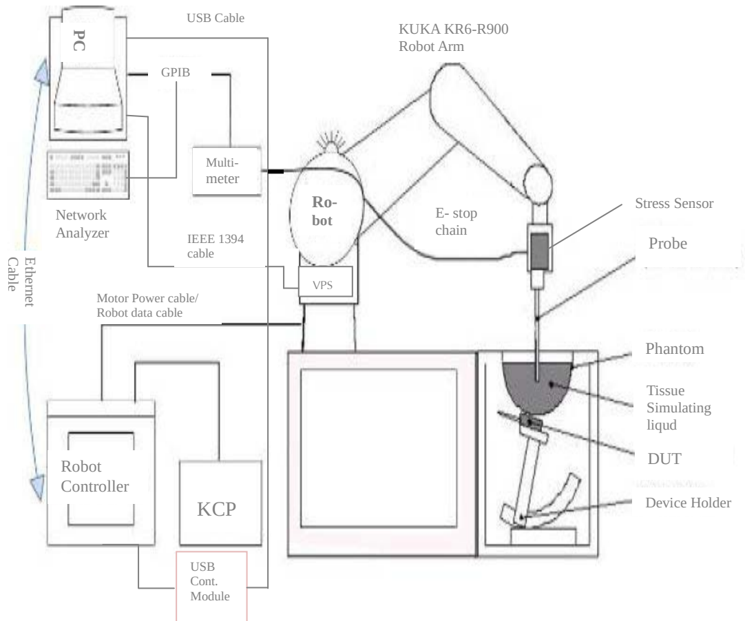
Figure a. SAR Measurement System Configuration
