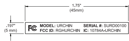
SN Label Artwork Scale: Full Size 5 mm W x 45 mm H
